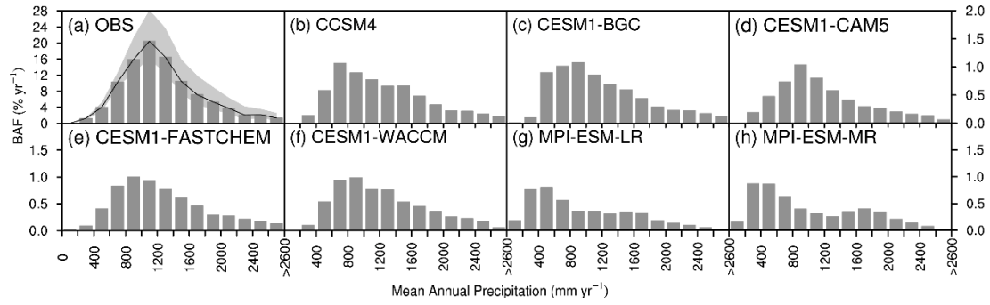
Fig. S11. Burned area fraction between 35°N and 35°S in 200 mm yr -1 bin of mean annual precipitation for benchmarks and CMIP5 models.
