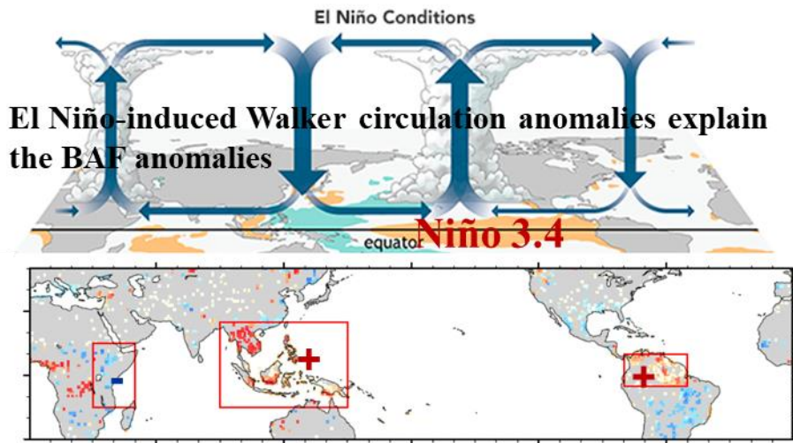
Fig. S10. Influence of ENSO on the burned area. The lower panel shows the regressed coefficient of Jun-May GFED5 BAF anomalies related to the DJF Niño 3.4 index from 1997 to 2020. The El Niño event leads to an increase in burned area fraction in equatorial Southeast Asia and South America, while a decrease in eastern Africa, due to the El Niño-induced zonal Walker circulations along the equator.
