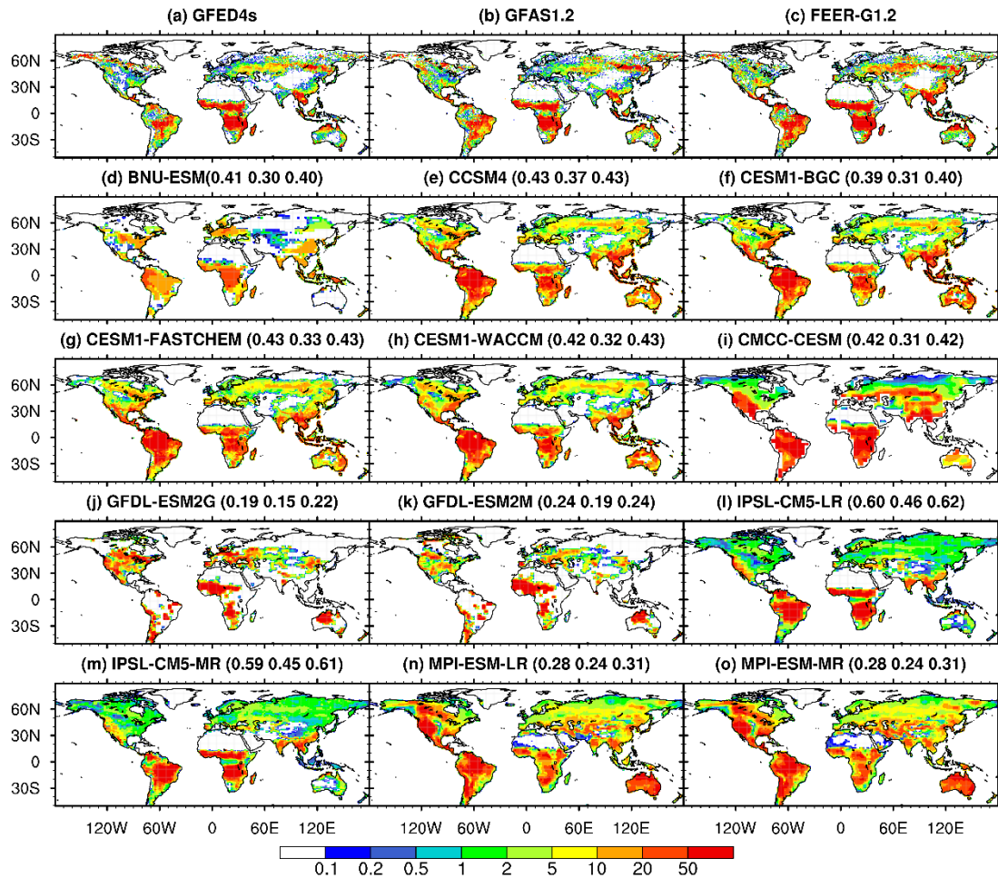
Fig. S6. Same as Fig. S2, but for the 2003–2004 average of fire carbon emissions ( \text{g C m}^{-2} \text{yr}^{-1} ).
