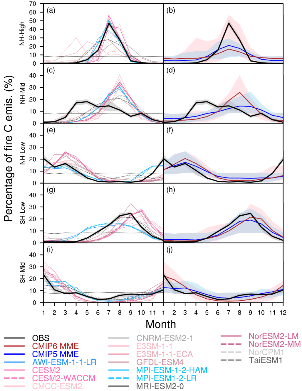
Fig. S8. Seasonal cycle of fire carbon emissions for observations and (left) CMIP6 models averaged over 2003–2014 and (right) CMIP6 and CMIP5 multi-model mean (MME) for 2003–2005. EC-Earth3 models that update fire emissions annually are excluded.
