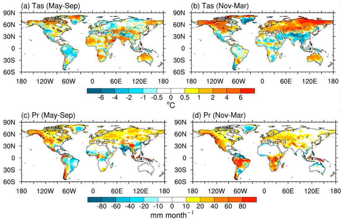
Fig. S5. Same as Fig. S3, but for the simulation bias of MRI-ESM2-0 in (a–b) surface air temperature and (c–d) precipitation for 2003–2014.
