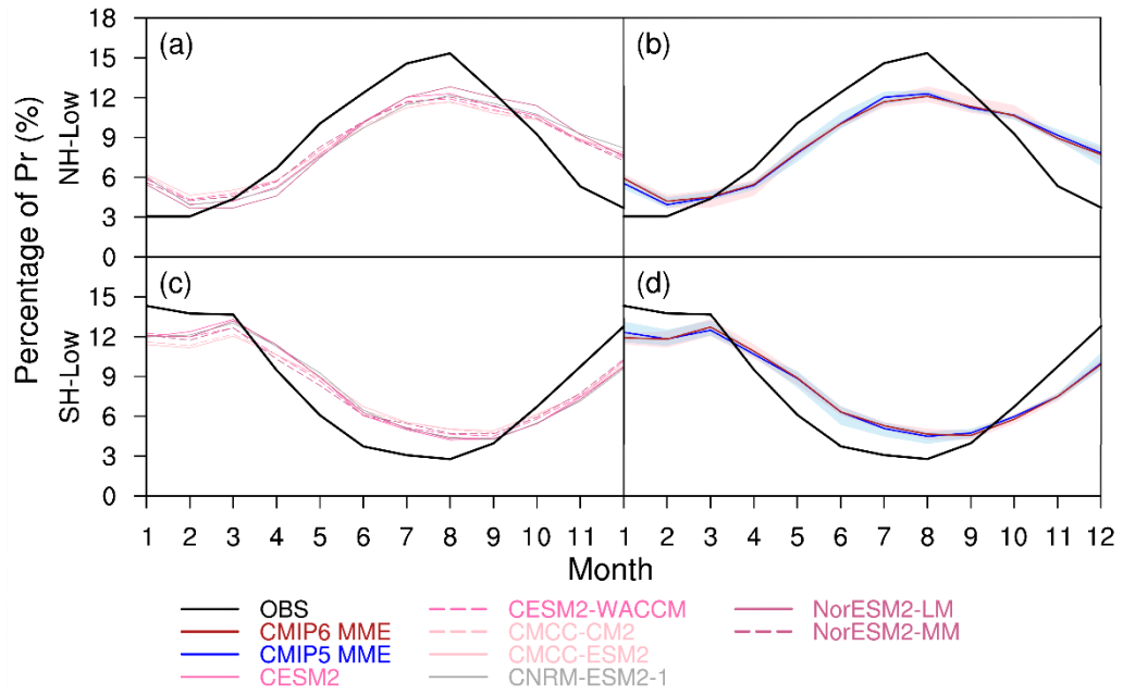
Fig. S7. Seasonal cycle of precipitation in low latitudes for observations and (left) CMIP6 models averaged over 2001–2014 and (right) CMIP6 and CMIP5 multi-model mean (MME) for 2001–2005.
