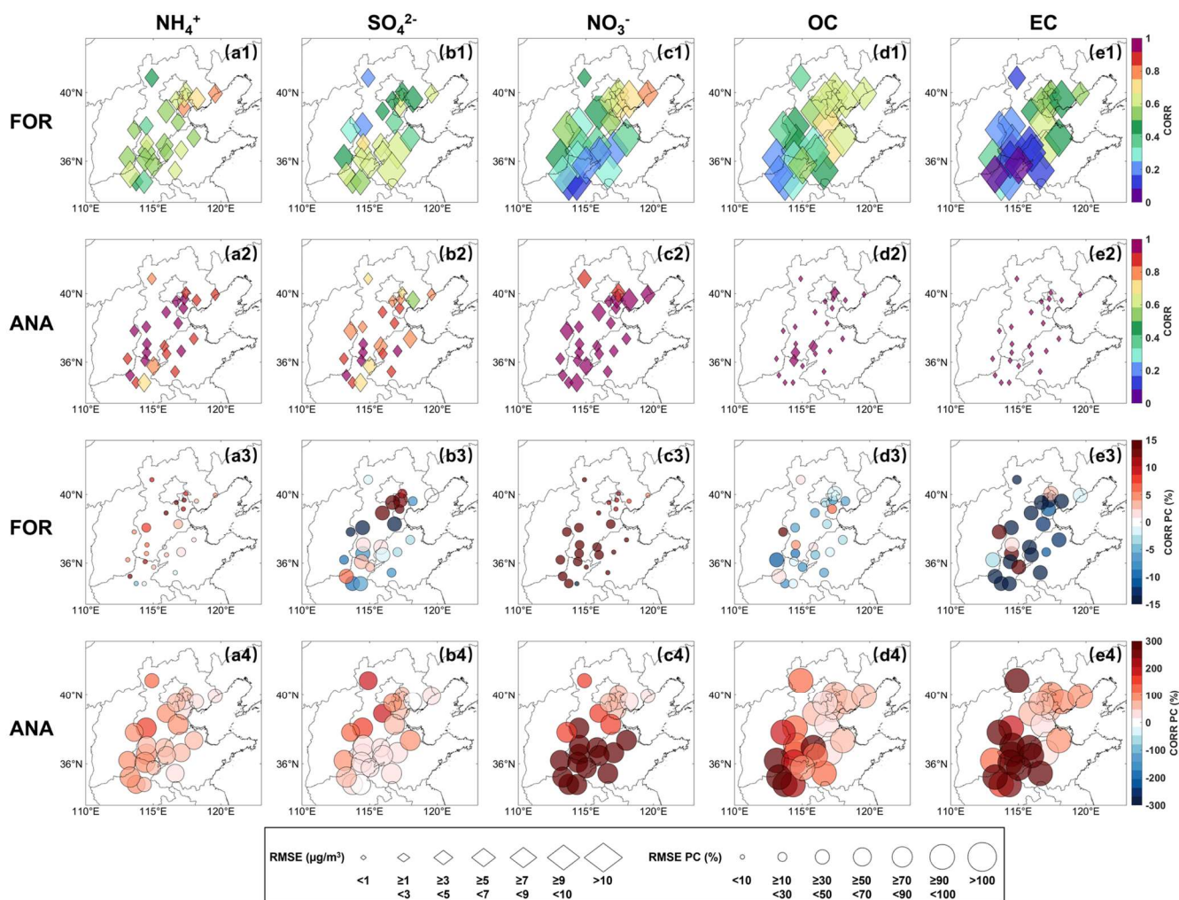
537 538 Figure 12: Spatial distribution of DA-site statistical indicators for five PM 2.5 chemical components. (a1-e1) represents the values of 539 RMSE and CORR for the forecast field (FOR), (a2-e2) same as (a1-e1) but for analysis field (ANA), (a3-e3) represents the 540 improvement of RMSE and CORR for the forecast field (FOR), (a4-e4) same as (a3-e3) but for analysis field (ANA). The size 541 represents the value of RMSE in (a1-e2) and the improvement percentage compared to non-assimilation in (a3-e4), respectively.
