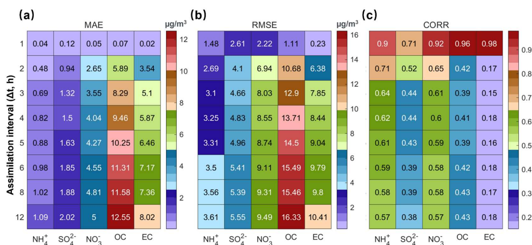
446 447 Figure 5: Assessment of assimilation interval dependency based on mean absolute error (MAE) (a), root mean square error (RMSE) 448 (b), and correlation coefficient (CORR) (c) at the analysis step.
