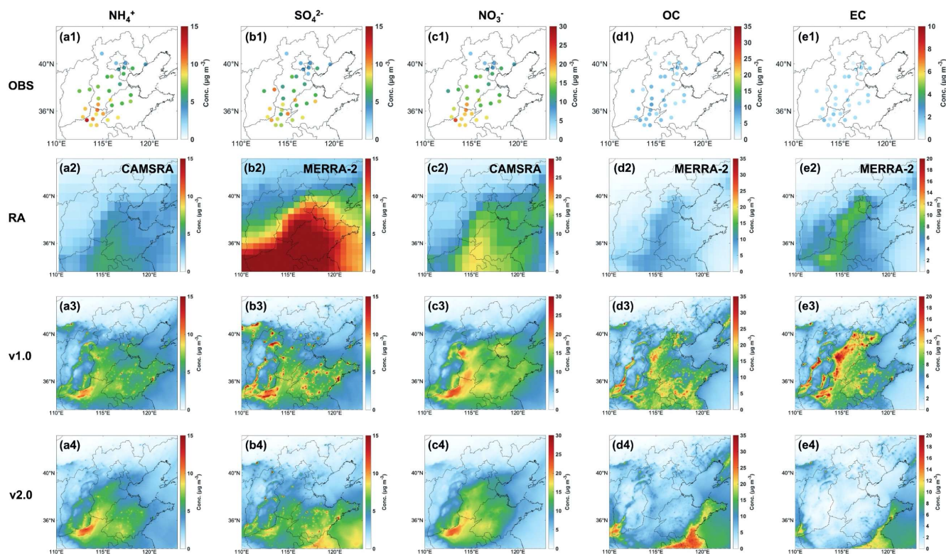
606 607 Figure 13: Spatial distribution of the monthly averaged concentration of five PM 2.5 chemical components for observations (OBS, a1- 608 e1), global reanalysis data (RA, a2-e2), NAQPMS-PDAF v1.0 analysis data (a3-e3) and NAQPMS-PDAF v2.0 analysis data (a4-e4).
