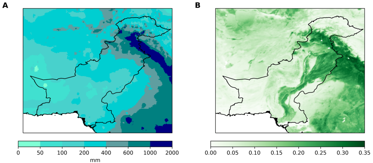
285 Figure 5: Maps of precipitation and NDVI annual means. A) Annual mean precipitation in the case study region; B) Annual mean maximum 15-day NDVI in the case study region. The country outline shows the border of Pakistan.
