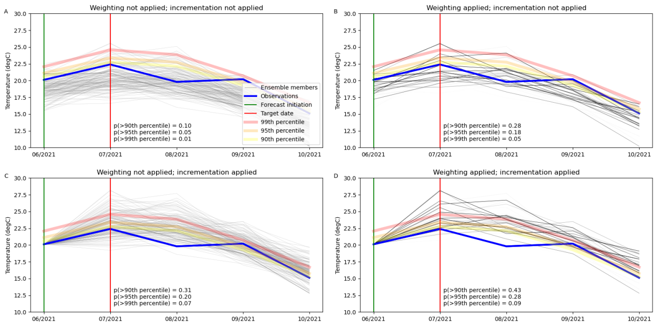
245 Figure 3: Example forecasts with one-month lead for July 2021. A) No weighting or incrementation of the time series B) Weighting of the climatology by year proximity but no incrementation of the time series; C) Incrementation of the time series from the initiation but no weighting; D) Weighting by year proximity and incrementation of the time series. In all of the plots, observations are blue, the 90 th , 95 th , and 99 th percentiles are pale yellow, yellow and orange and individual ensemble members are grey. The green vertical line is the date of forecast initiation and the red line is the target date. In B and D, the weighting is denoted by the darkness of the lines.
