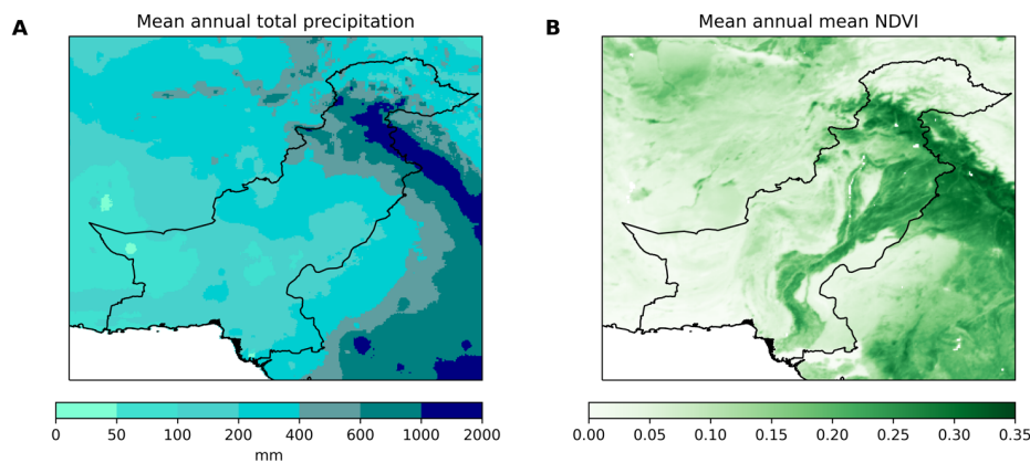
310 Figure 5: Maps of precipitation and NDVI annual means. A) Annual mean precipitation in the case study region; B) Annual mean maximum 15-day NDVI in the case study region. The country outline shows the border of Pakistan.
