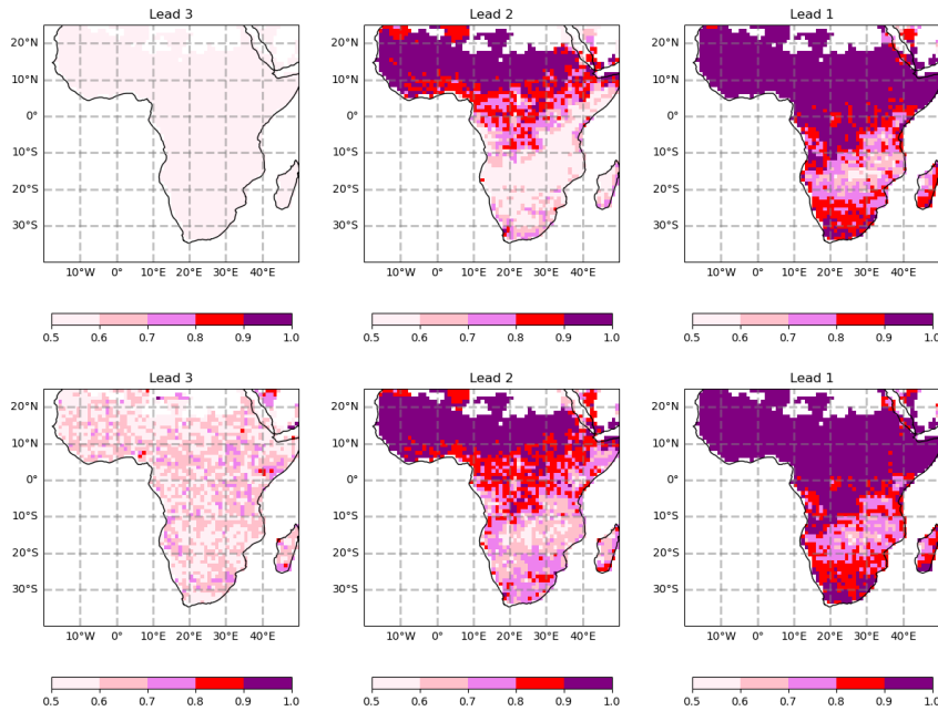
445 Figure 10: ROC scores for 3-month SPI3 on November 15 th . From left to right: 3-month lead (forecast initiated on 15 th August); 2-month lead (forecast initiated on 15 th September); 1-month lead (forecast initiated on 15 th October); Observed SPI3. The top row displays forecasts with no weighting applied to the ensemble. The bottom row displays forecasts, with the ensemble weighted using the Oceanic Nino Index (ONI).
