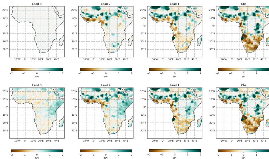
Figure 9: Example forecast for 3-month SPI3 on November 15 th 2015. From left to right: 3-month lead (forecast initiated on 15 th August); 2-month lead (forecast initiated on 15 th September); 1-month lead (forecast initiated on 15 th October); Observed SPI3. The top row displays forecasts with no weighting applied to the ensemble. The bottom row displays forecasts, with the ensemble weighted using the Oceanic Nino Index (ONI).
