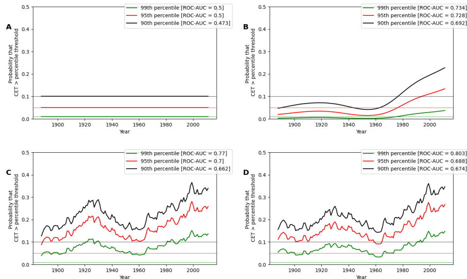
290 Figure 4: Time series of predicted probabilities that the July Central England Temperature (CET) will exceed the 1850-2020 90 th , 95 th and 99 th percentile for a 1-month lead – i.e. forecasts initiated in June. A) No weighting or incrementation of the time series B) Weighting of the climatology by year proximity but no incrementation of the time series; C) Incrementation of the time series but no weighting; D) Both weighting and incrementation applied. The bold lines show modelled probabilities of exceedance of the 90 th , 95 th and 99 th percentile thresholds, and the fine lines show the climatological probabilities.
