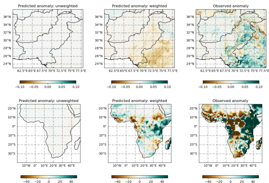
510 Figure 11: Forecasts and observations of Pakistan (and surround region) seasonal mean NDVI anomaly (top) and Africa cumulative precipitation anomaly (bottom). Comparison between unweighted forecasts (left), weighted forecasts (middle) and observations (right). Forecasts are initiated on 1 st August 1997 and target the September-November 1997 season. The weighting is based on the Oceanic Nino Index.
