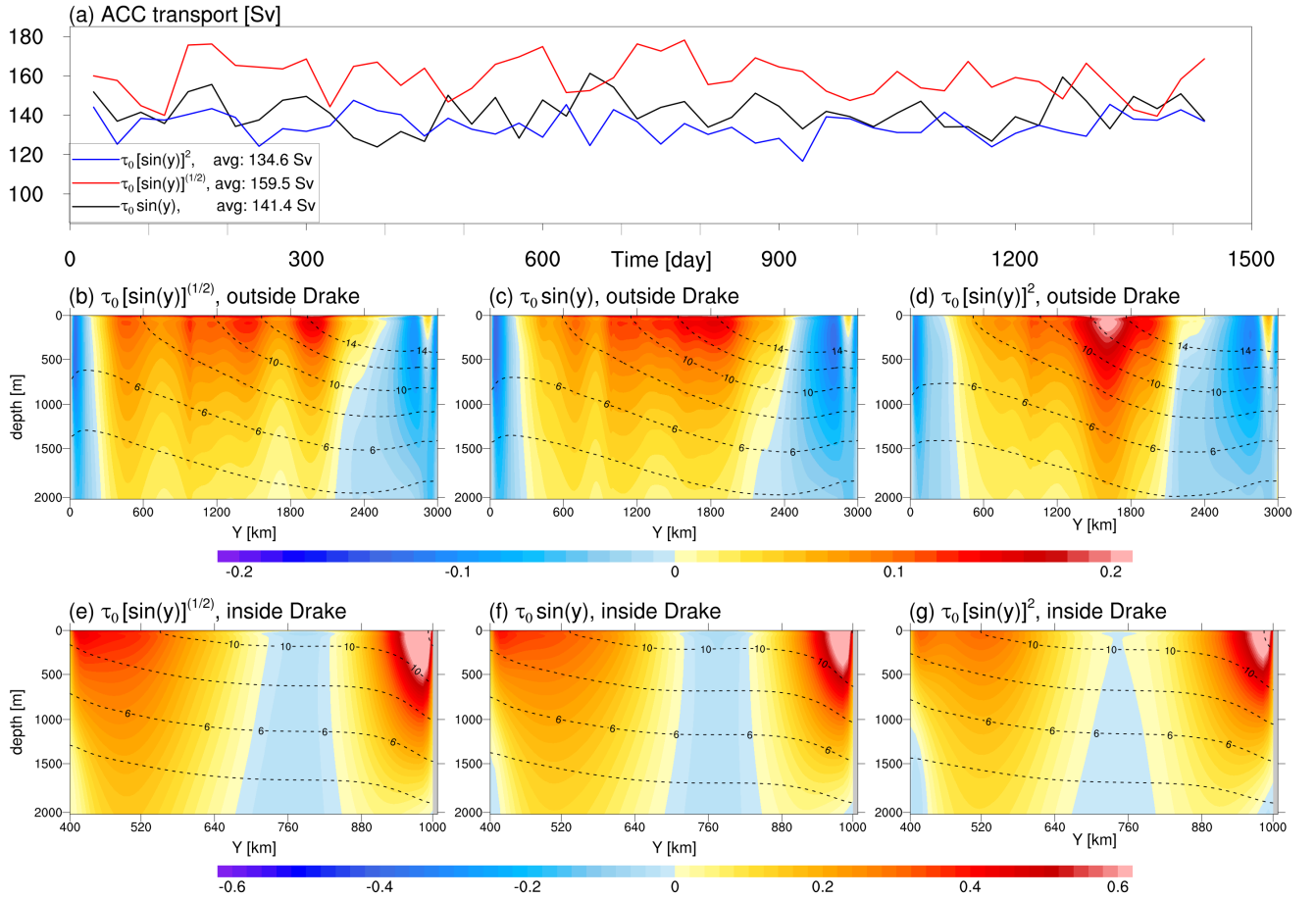
Figure 2. (a) The monthly-averaged ACC transport under three wind stress profiles. (b-d) are zonal-averaged zonal velocity (shading) and zonal-averaged potential temperature (contours) outside the idealized Drake passage under three wind stress profiles. (e-g) are as (b-d) but inside the idealized Drake passage.
