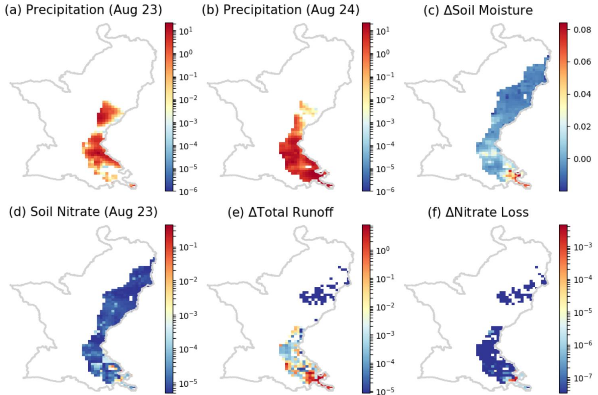
Figure 7. Comparison of variables between August 23rd and 24 th for the calibrated model: (a) precipitation (mm/d) on August 23 rd , (b) precipitation (mm/d) on August 24 th , positive increase of soil moisture ( m^3/m^3 )(c), soil nitrate-nitrogen ( gN/m^2 ) on August 23 rd (d), positive increase in runoff (mm/d) (e), and positive increase in nitrate-nitrogen leaching loss ( gN/m^2/d ) (f) from August 23 rd .
