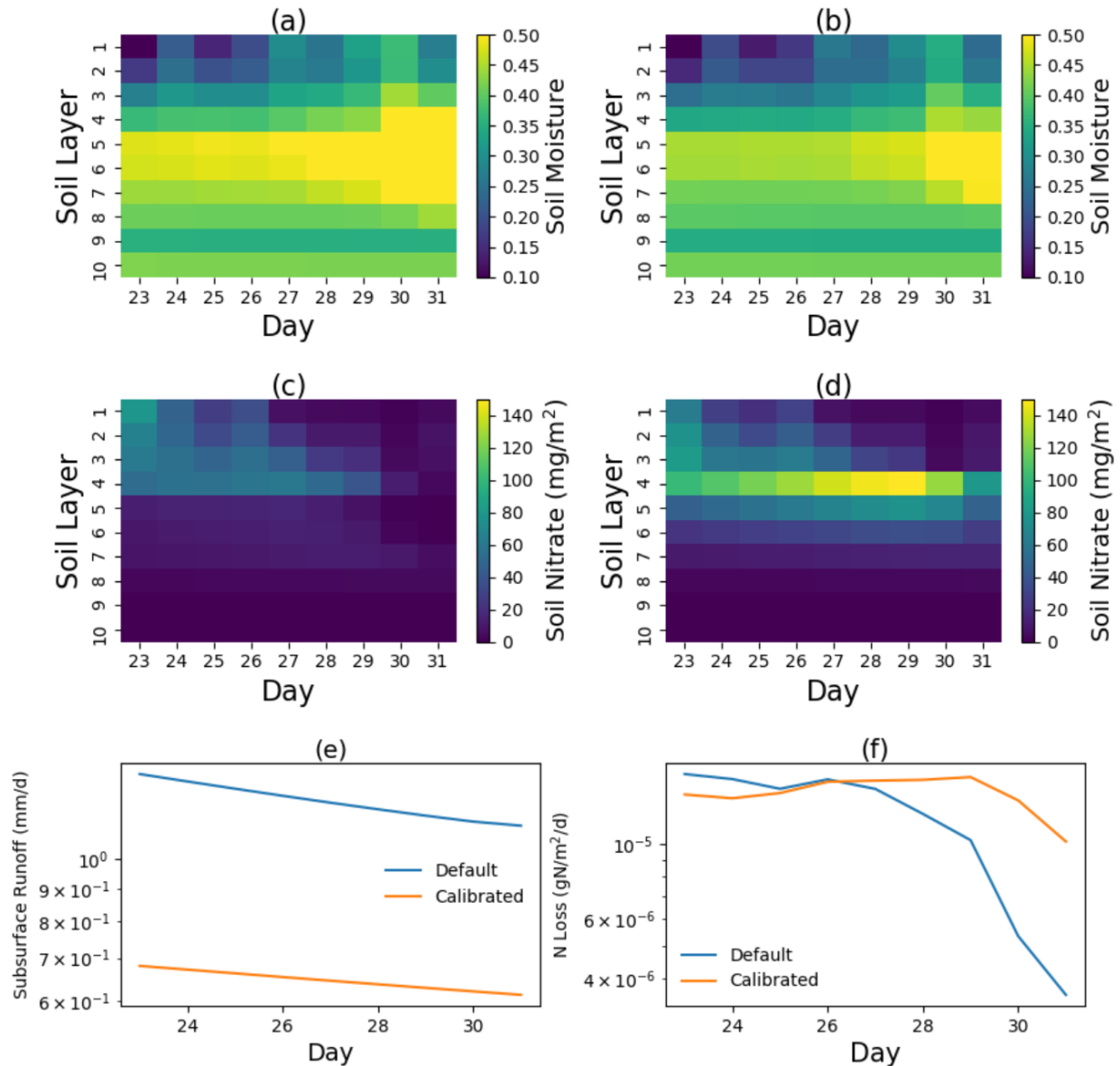
415 Figure 8. Heatmap comparison of soil moisture and soil mineral nitrate-nitrogen between the default model (a,c), the calibrated model (b,d), subsurface runoff (e) and nitrogen leaching loss (f) at a selected nearshore grid.
