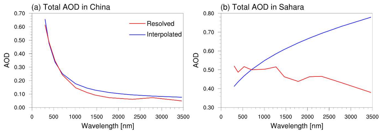
Figure 2. Simulated AOD as a function of wavelength, averaged for January and July 2015 (a) AOD averaged over anthropo-dominant region in East China (as shown in Fig. 1); (b) AOD averaged over dust-dominant region in the Sahara (as shown in Fig. 1). The blue and red line represent the “Interpolated” and the “Resolved” method, respectively.
