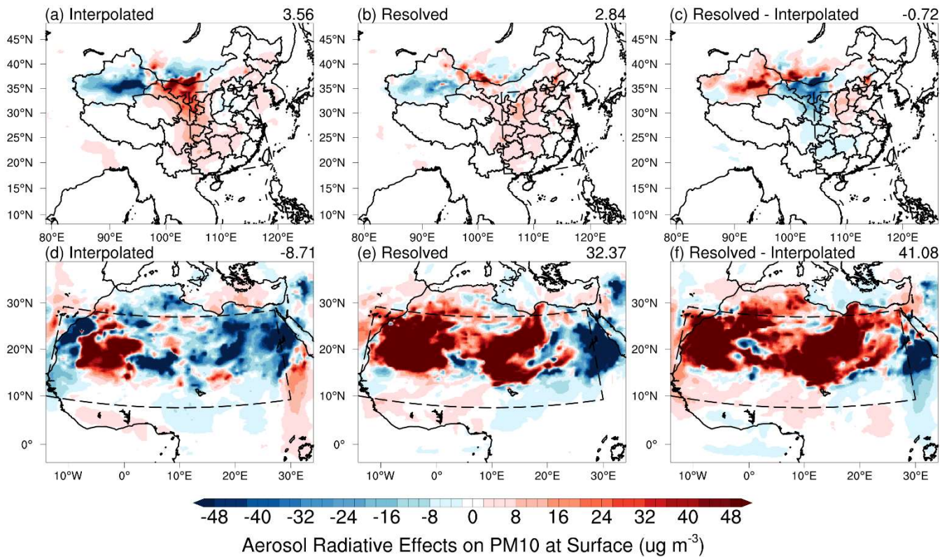
Figure 13. Same as Fig. 9 but for particulate matter with diameters 10 \mu\text{m} and smaller (PM10) at surface.
