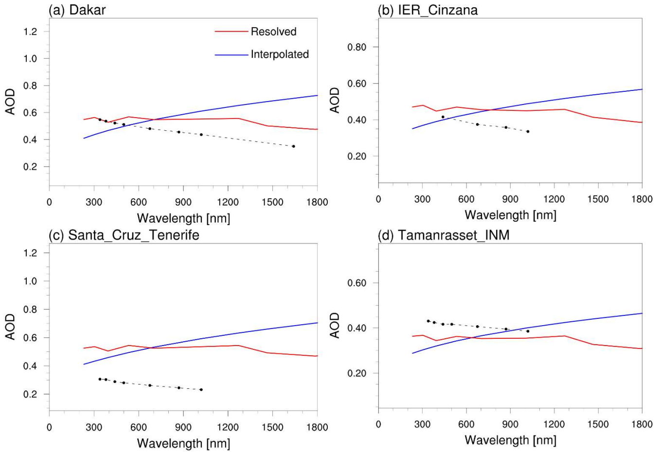
Figure 3. Comparison of total AOD from simulations and AERONET observations in dust-dominant areas. The results are both averaged for January and July 2015. The blue and red line represent the “Interpolated” and the “Resolved” method, respectively. The AERONET AOD values are indicated by black dots in each panel. The simulation results are obtained from the grid box closest to the AERONET stations.
