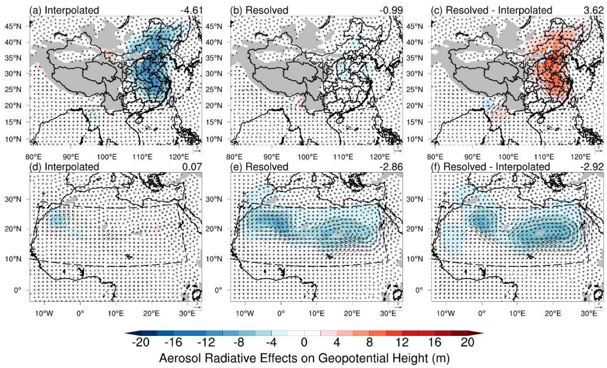
Figure 11. Same as Fig. 9 but for wind fields (vectors) and geopotential height (shaded contour) at 850 hPa.
