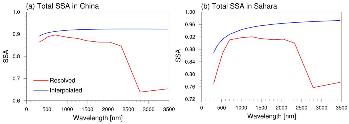
Figure 4. Simulated SSA as a function of wavelength, averaged for January and July 2015 (a) SSA averaged over anthropo- 685 dominant region in East China (as shown in Fig. 1); (b) SSA averaged over dust-dominant region in the Sahara (as shown in Fig. 1). The blue and red line represent the “Interpolated” and the “Resolved” method, respectively.
