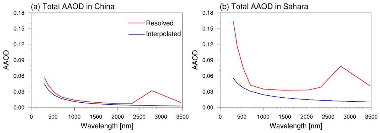
Figure 5. Simulated AAOD as a function of wavelength, averaged for January and July 2015 (a) AAOD averaged over anthro-dominant region in East China (as shown in Fig. 1); (b) AAOD averaged over dust-dominant region in the Sahara (as shown in Fig. 1). The blue and red line represent the “Interpolated” and the “Resolved” method, respectively.
