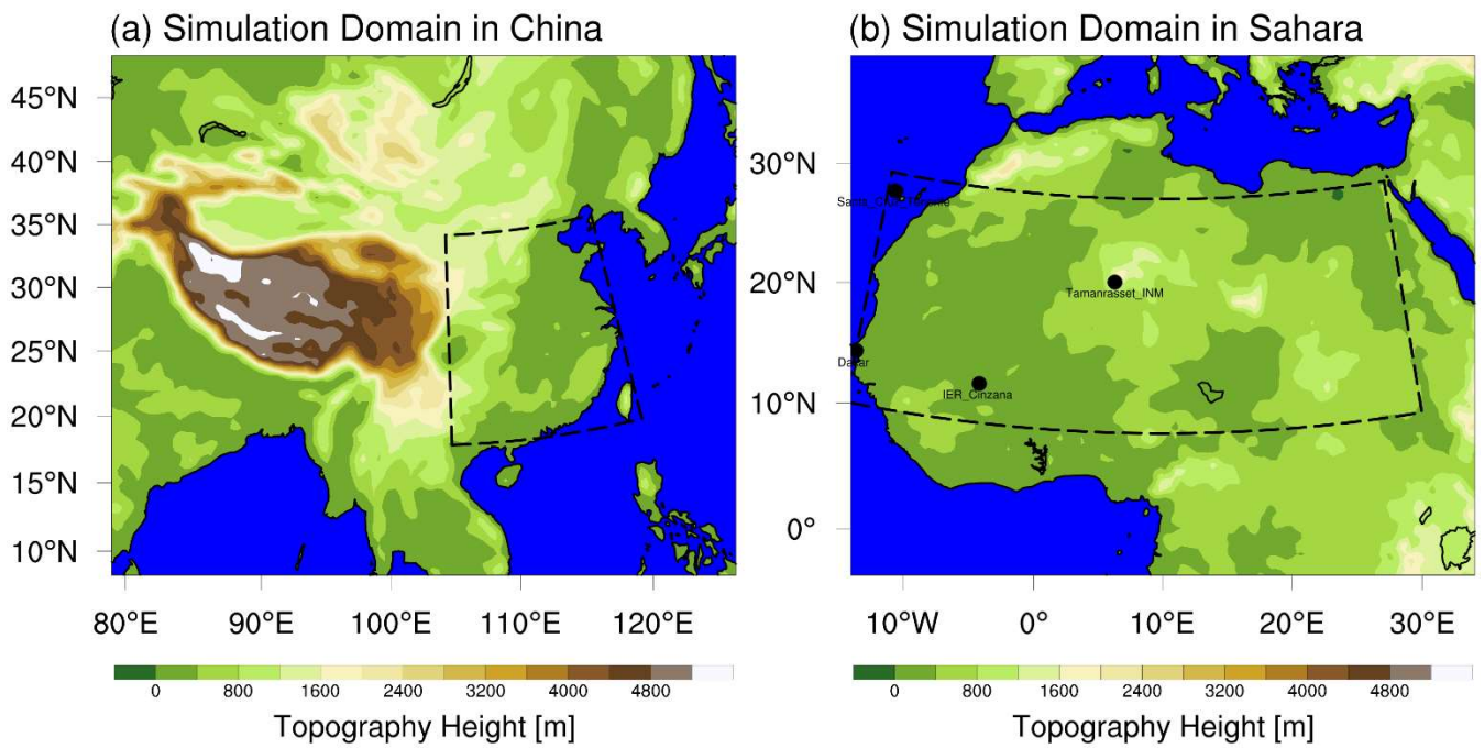
665 Figure 1. Simulation domains. (a) in China; (b) in Sahara. The dashed-line boxes in panel (a) and (b) represent regions dominated by anthropogenic aerosols and dust aerosols, respectively. Spatial distributions of topography height are also shown. Locations of selected AERONET stations over dust-dominant areas in Sahara are also denoted in panel (b) .
