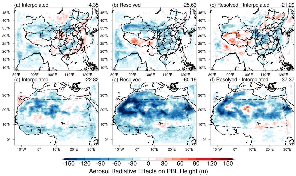
Figure 12. Same as Fig. 9 but for PBL height.
