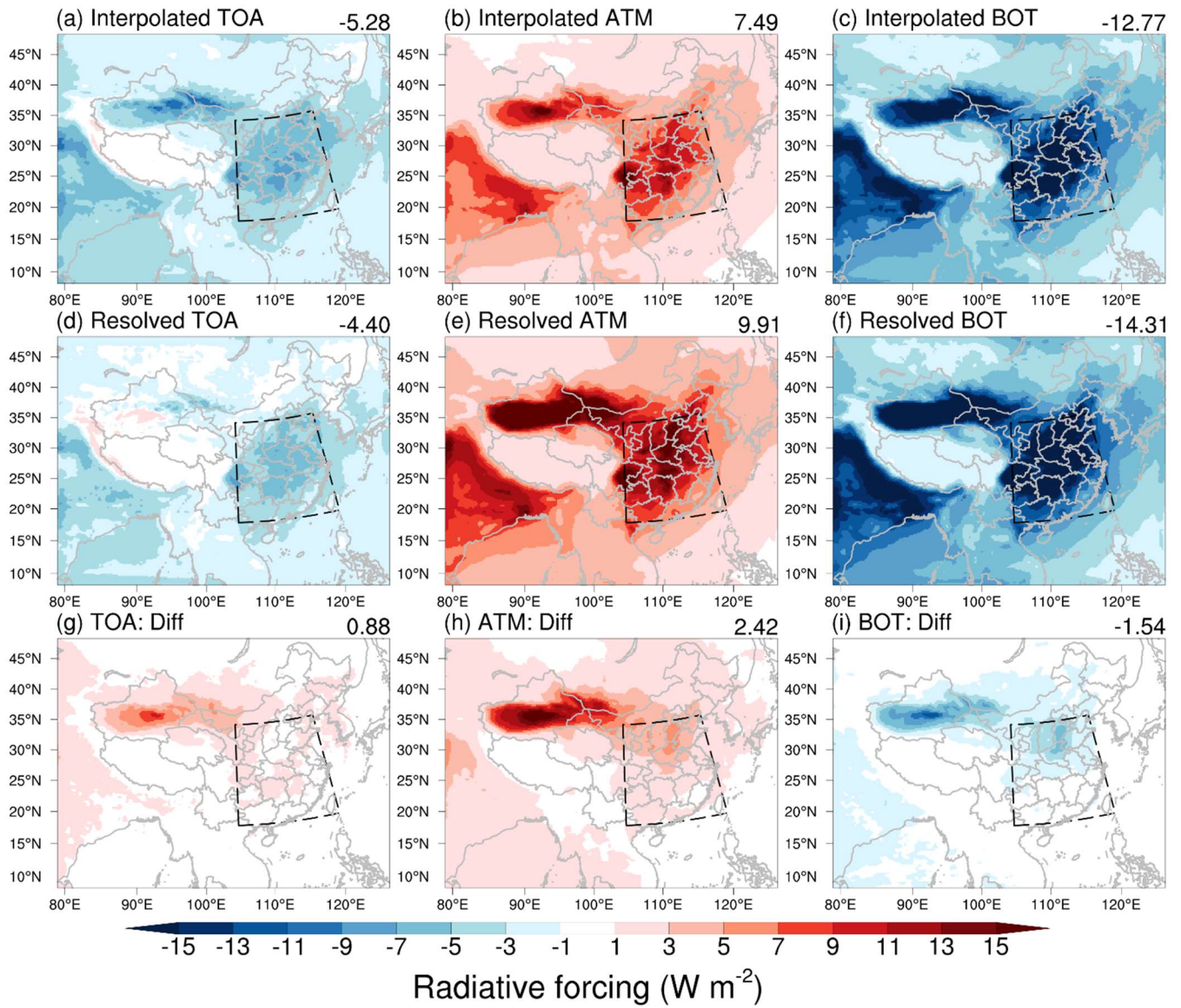
695 ss Figure 6. Radiative forcing of all aerosols in China at TOA, BOT, and in ATM, averaged for January and July 2015. The top and middle panels show the results using “Interpolated” and “Resolved” methods, respectively. The bottom panels show the differences between the “Interpolated” method and the “Resolved” method. The average results of anthro-dominant areas (dashed-line boxes) are shown in the top right corner.
