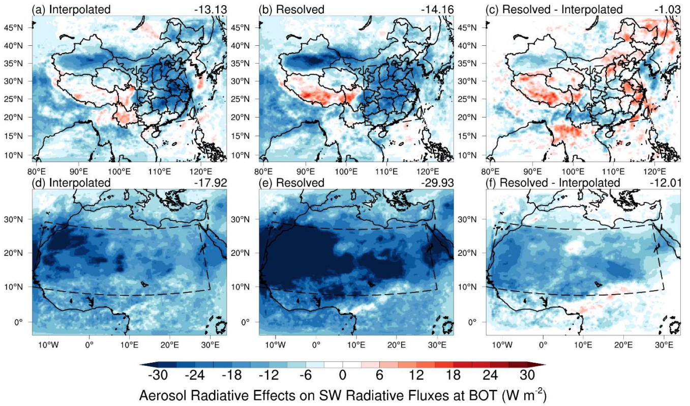
Figure 10. Same as Fig. 9 but for the net short-wave radiative fluxes at the bottom of the atmosphere (positive denotes downward).
