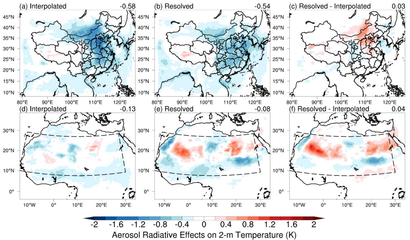
715 Figure 9. (a, d) Spatial distribution of aerosol radiative effects on 2-m temperature from the “Interpolated” experiments in China and Sahara, respectively; (b, e) Spatial distribution of aerosol radiative effects on 2-m temperature from the “Resolved” experiments in China and Sahara, respectively; (c, f) The impacts of algorithm amendment on the simulated aerosol radiative effects (difference in aerosol radiative effects between “Resolved” and “Interpolated”) on 2-m temperature in China and Sahara, respectively. The average results of anthro-dominant (dashed-line boxes in a, b, and c) and dust-dominant areas (dashed-line boxes in d, e, and f) are shown in the top right corner. The results are averaged for January and July 2015.
