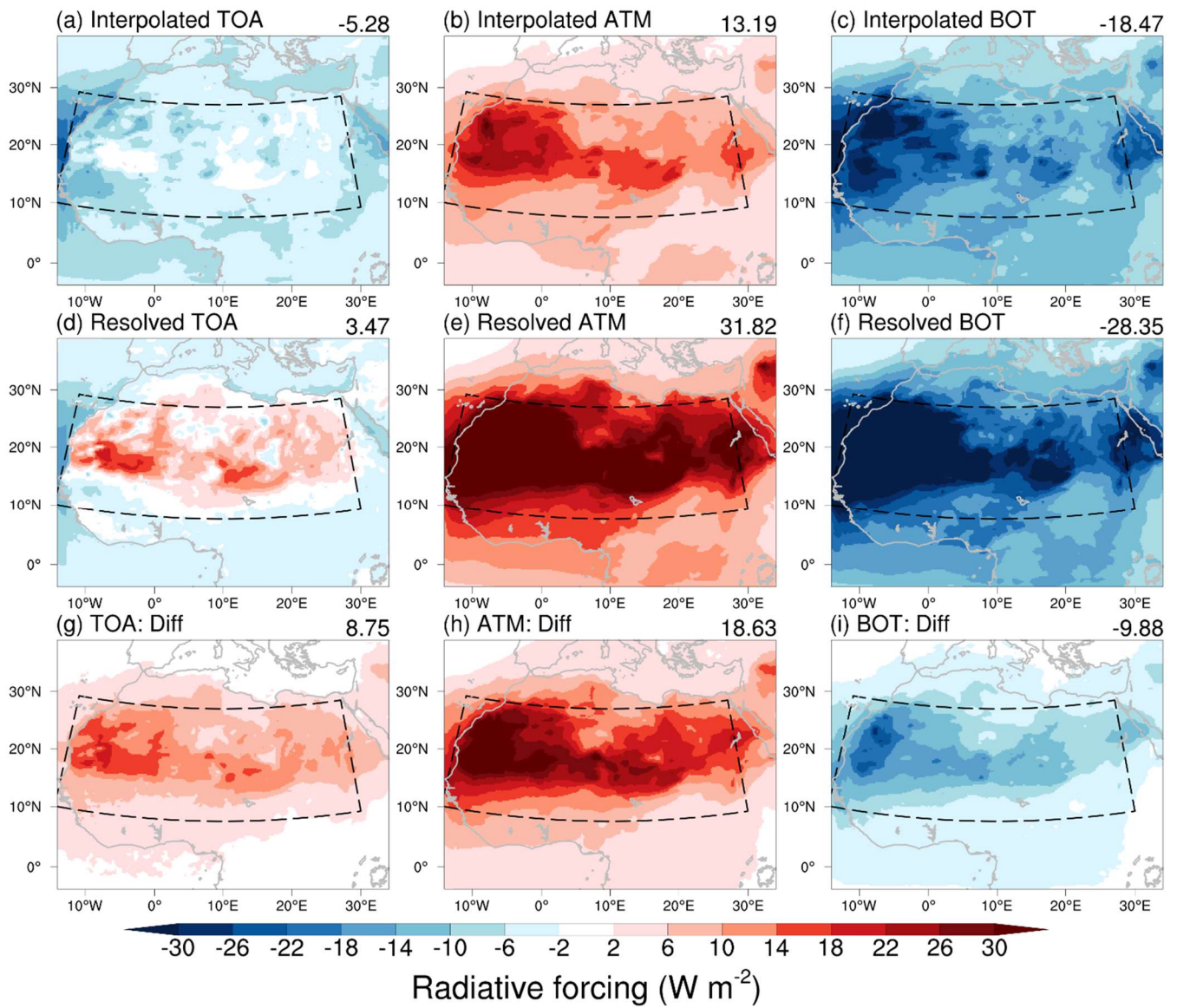
Figure 7. Radiative forcing of aerosols in Sahara at TOA, BOT, and in ATM, averaged for January and July 2015. The top and middle panels show the results using “Interpolated” and “Resolved” methods, respectively. The bottom panels show the differences between the “Interpolated” method and the “Resolved” method. The average results of dust-dominant areas (dashed-line boxes) are shown in the top right corner.
