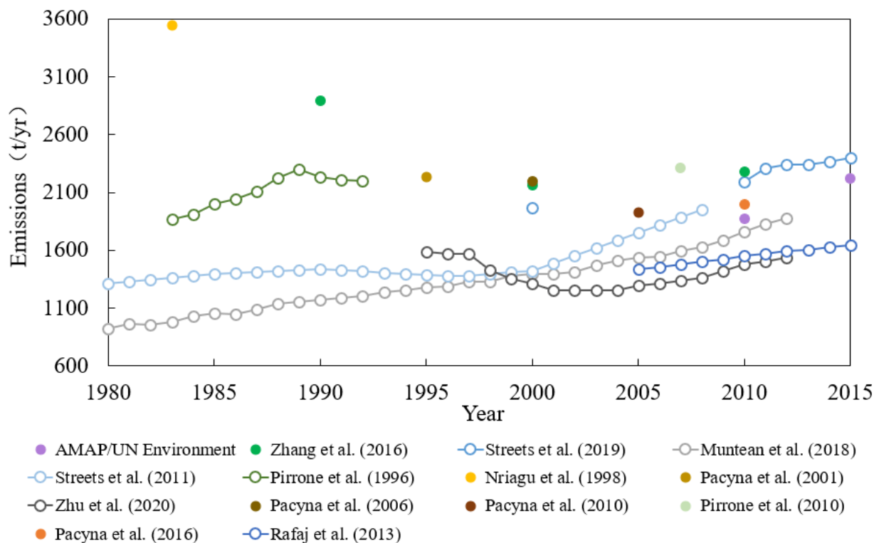
Figure 2. Temporal trends of global anthropogenic Hg emissions to air based on available inventories (AMAP/ UN Environnement, 2019; Streets et al., 2011; Zhu et al., 2020; Pacyna et al., 2016; Zhang et al., 2016b; Pacyna et al., 2006a; Rafaj et al., 2013; Streets et al., 2019b; Pacyna et al., 2010; Muntean et al., 2018; Pacyna et al., 2001; Pirrone et al., 2010, 1996, 1998).
