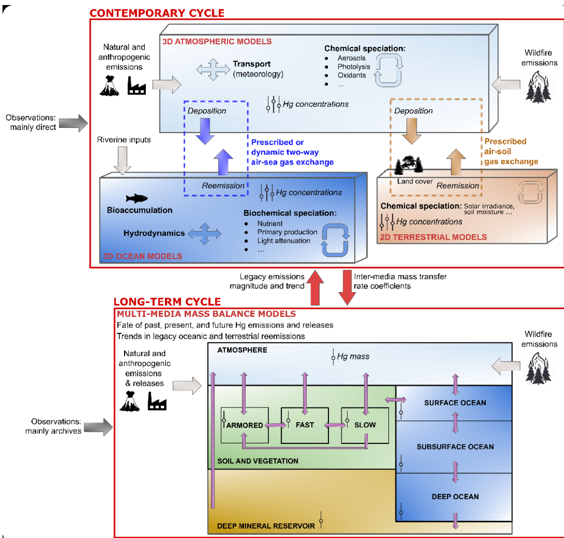
455 Figure 1. Conceptual design of large-scale environmental Hg models and their coordination in MCHgMAP. Summary of key drivers and coupling between 3D atmospheric, 3D marine, 2D terrestrial, and multi-media mass balance models. Different configurations are possible, ranging from prescribed to dynamic two-way surface–atmosphere gas exchange.
