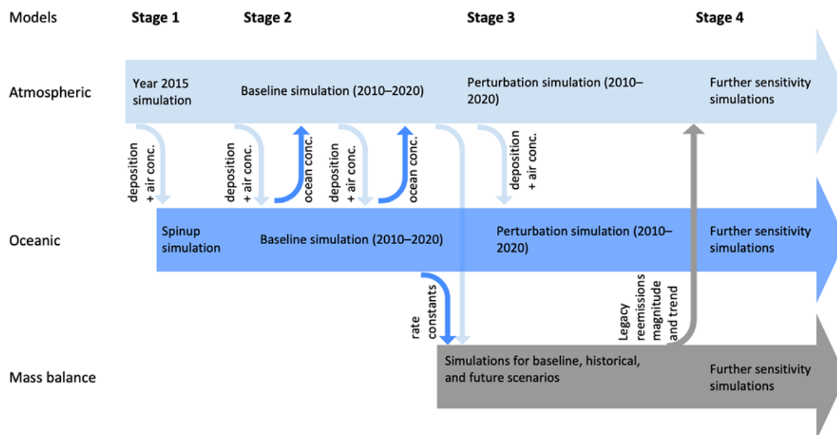
1675 Figure 8. Diagram showing how the coupling between atmospheric, oceanic, and mass balance models will be achieved by conducting the work in stages and exchanging information between model types in MCHgMAP.
