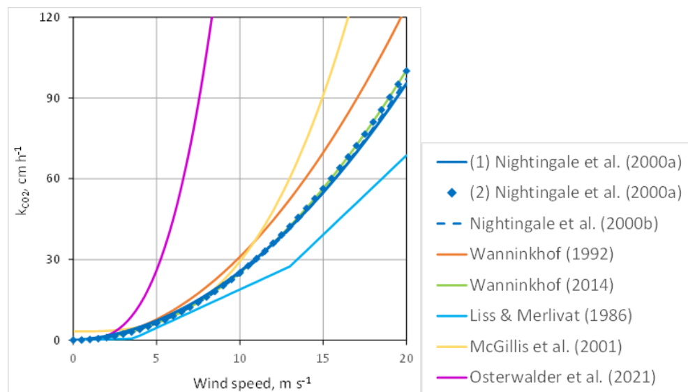
Figure B1. Wind speed dependence of air-water gas transfer velocities from various parameterizations often applied in Hg modelling and measurement studies scaled to a Schmidt number of CO 2 at 20°C ( k_{CO_2} ). Nightingale et al. (2000a) parameterizations 1 and 2 (in solid dark blue) are both commonly used in Hg work and give almost identical results. The dark blue dotted line refers to Nightingale et al. (2000b), the orange line to Wanninkhof (1992), the green line to Wanninkhof (2014), the light blue line to Liss and Merlivat (1986), the yellow line to McGillis et al. (2001), and the pink line to Osterwalder et al. (2021).
