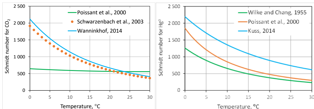
2635 Figure B2. A) Temperature dependence of the Schmidt number for CO 2 in seawater (from Poissant et al. (2000) in green, Schwarzenbach et al. (2003) in orange, and Wanninkhof (2014) in blue). Data from Schwarzenbach et al. (2003) are added for comparison, B) Temperature dependence of the Schmidt number of Hg(0) in seawater (from Wilke and Chang (1955) in green, Poissant et al. (2000) in orange, and Kuss (2014) in blue).
