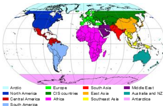
2665 Figure C1. Geographical receptor regions for atmospheric model analysis.
