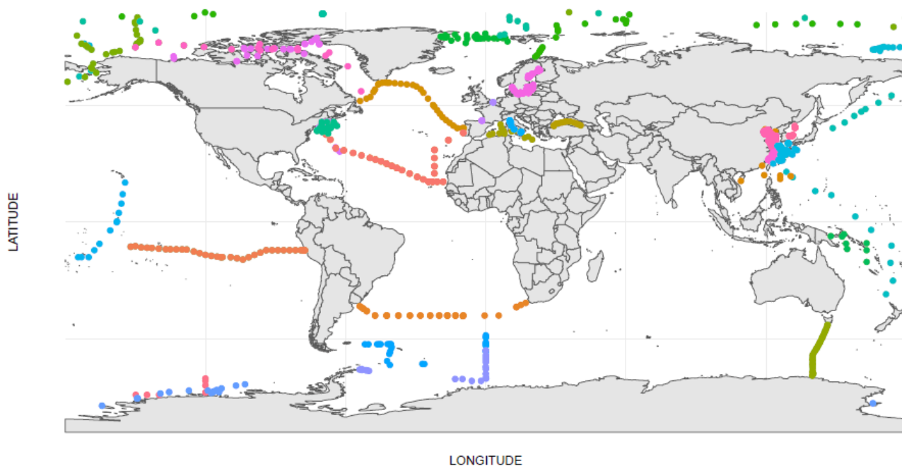
1420 Figure 7. THg and MeHg marine sampling locations conducted with rosette during the past ~15 years showing a global coverage (except for the Indian Ocean and parts of the Pacific Ocean). Note that this is a subset of existing published datasets. References: Agather et al., (2019), Bowman et al., (2015, 2016), Bratkič et al. (2016), Ci et al., (2016b), Cossa et al., (2018), Hammerschmidt et al., (2013), Jonsson et al., (2022), Kim et al., (2017, 2020), Marumoto et al., (2018), Munson et al., (2015), Nerentorp Mastromonaco et al., (2017b, a), Perrot et al., (2023), Petrova et al., (2020), Sharif et al., (2014), Soerensen et al., (2013, 2016a, 2018), Yang et al., (2017), Yue et al., (2023), Wang et al., (2016a, 2020a). GEOTRACES cruises downloaded from the repository www.bodc.ac.uk .
