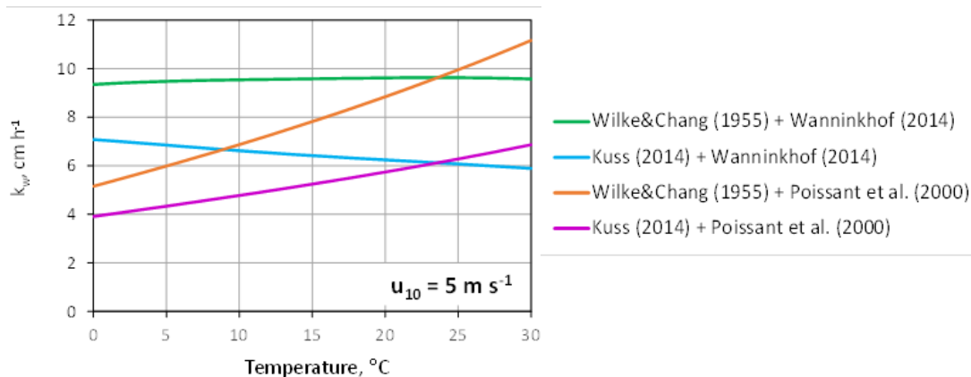
2640 Figure B3. Temperature dependence of air-seawater gas transfer velocity for Hg(0) (from Wilke and Chang (1955) and Wanninkhof (2014) in green, from Kuss (2014) and Wanninkhof (2014) in blue, from Wilke and Chang (1955) and Poissant et al. (2000) in orange, and from Kuss (2014) and Poissant et al. (2000) in pink).
