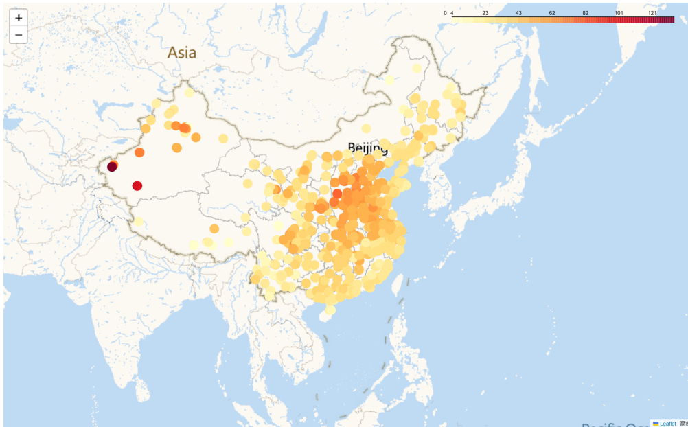
Figure 5. Diagram of the spatial distribution of PM2.5. Redder points represent higher PM2.5 values.
