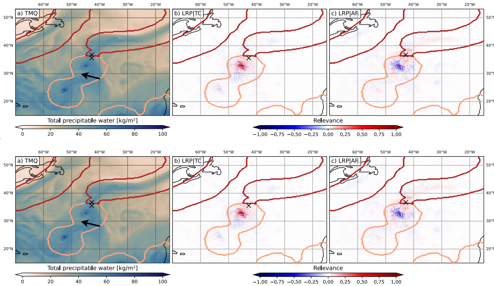
Figure 4: (a) Close-up of TMQ as shown in Fig. 3a for the NorthNorth Atlantic region. Black “x” mark two selected single grid points, the southern one within the TC feature, the northern one within the AR. (b) TMQ relevance for the southern (TC) grid point. (c) TMQ relevance for the northern (AR) grid point.
