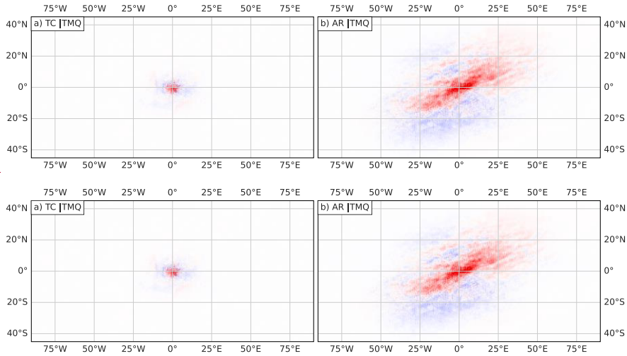
500 Figure 7: Composite relevance maps for TMQ, averaged over (a) all TC features in the test dataset, and centred on the features. (b) The same for ARs. For clarity of presentation only AR features from the northern hemisphere are composited due to the difference in orientation on the southern hemisphere.
