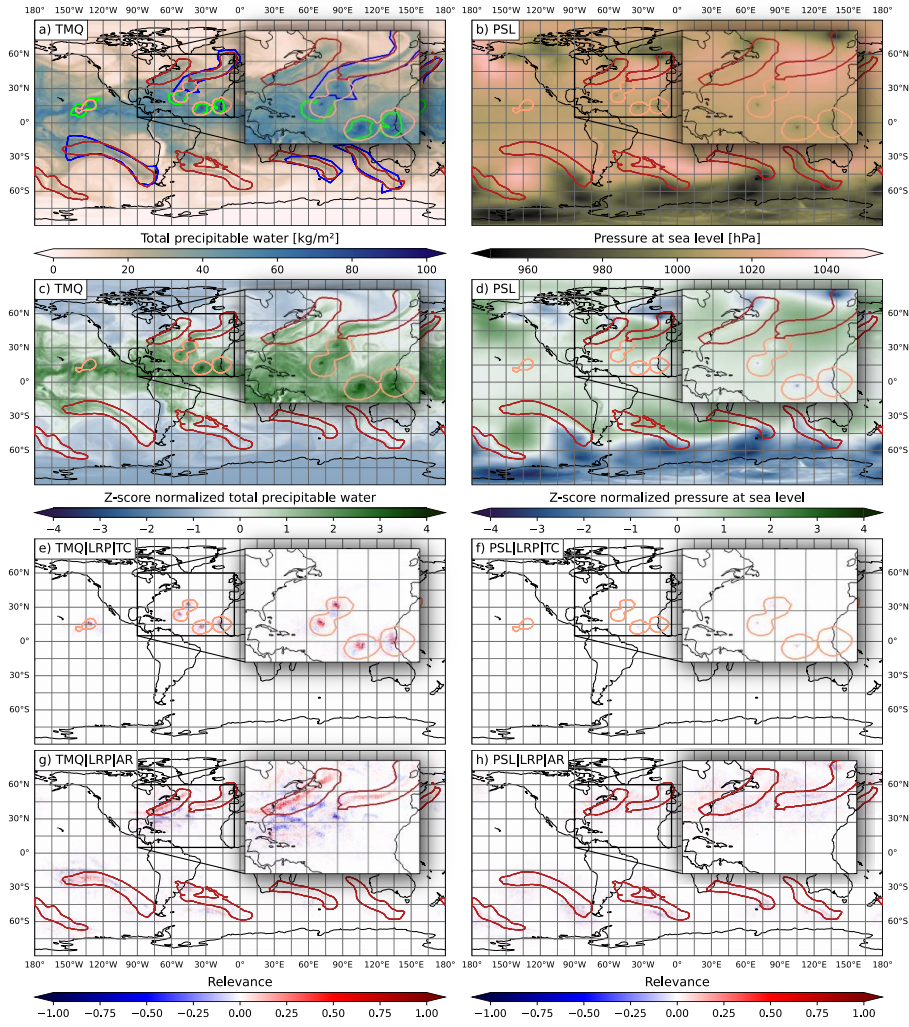
325 Figure 3: Global maps of (a) TMQ and (b) PSL for the time step contained for 27 September 2013 in the ClimateNet dataset. Orange (red) contours show TC (AR) features detected with CG-Net using the KS20 setup. Green (blue) contours show TC (AR) features
