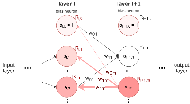
Figure 2: Schematic illustration of two (hidden) layers of an ANN (cf. Eq. 1). a_{l,m} denotes the activation of neuron m in layer l , R_{l,m}
