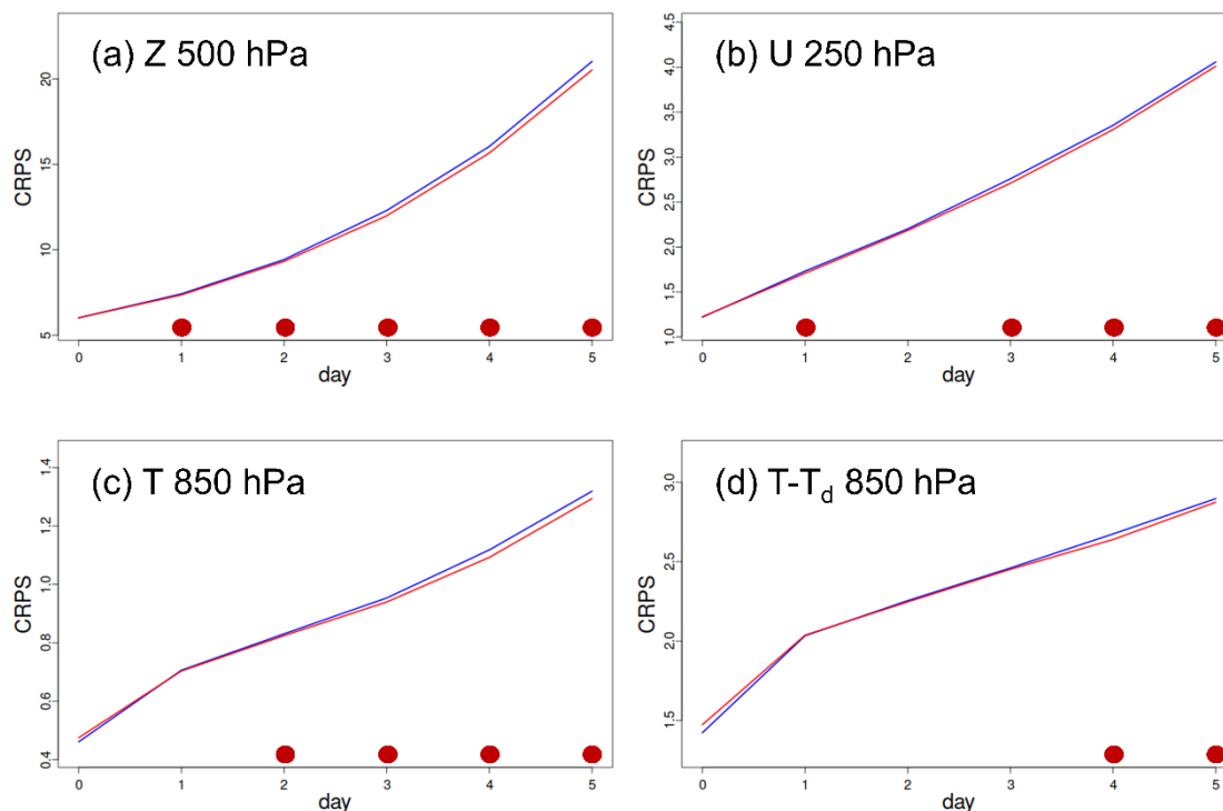
475 Figure 5: The CRPS of five-day ensemble forecasts from the previous EnKF system (in blue) and the new MIDAS-based LETKF 480 system (in red) computed with respect to the global network of radiosonde observations for (a) geopotential height at 500hPa, (b) zonal wind at 250hPa, (c) temperature at 850hPa, and (d) dew-point depression at 850hPa over the period January 1–25, 2017. The filled circles along the horizontal axis indicate lead-times when the difference in the score is considered statistically significant with the colour of the circle indicating the experiment with the better score. Note that these results use an earlier configuration of the LETKF and EnKF at lower spatial resolution and without ensemble recentering.
