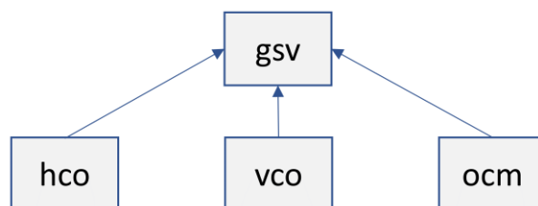
380 Figure 2: Relationship between the gridded state vector module ( gsv ) and lower-level modules that are used by this module through a composition relationship to represent the horizontal coordinate ( hco ), vertical coordinate ( vco ), and ocean mask ( ocm ).
