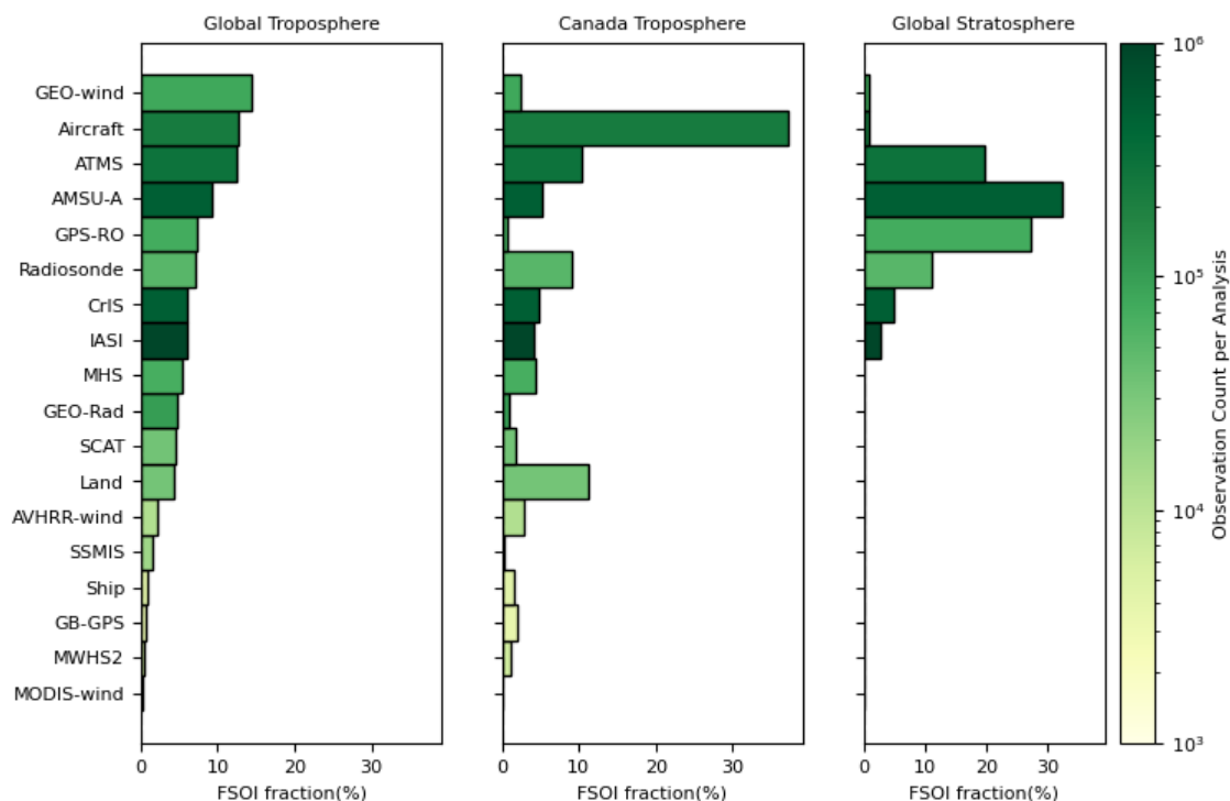
495 Figure 6: The average fractional observation impact on 24 h forecasts over the global domain (left) and over only Canada (middle) between the surface and 100hPa and for the global domain between 100hPa and 1hPa (right) separated by observation type. The colour of each bar indicates the average number of assimilated observations per analysis. The observation types are ordered according to the magnitude of their impact on global tropospheric forecasts.
