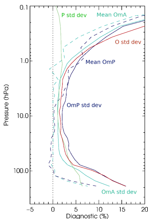
520 Figure 7: Global normalized mean (dashed) and stddev (solid) of MLS observation minus analysis (OmA, light blue) and observation minus short-term forecast (OmP, dark blue) differences and corresponding average observation-error stddev (O, red) and background-error stddev (P, green) used for assimilation. Results are for the June to August 2022 period.
