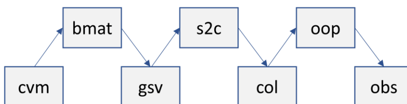
365 Figure 1: High-level relationship between some of the main MIDAS Fortran modules used for computing an analysis increment or background-error perturbation in observation space (see main text for definitions of module prefixes). The upper row of modules are transformations between the data-oriented modules in the lower row. Note that each module in the upper row includes “use” statements for the two modules in the lower row to which they are directly connected.
