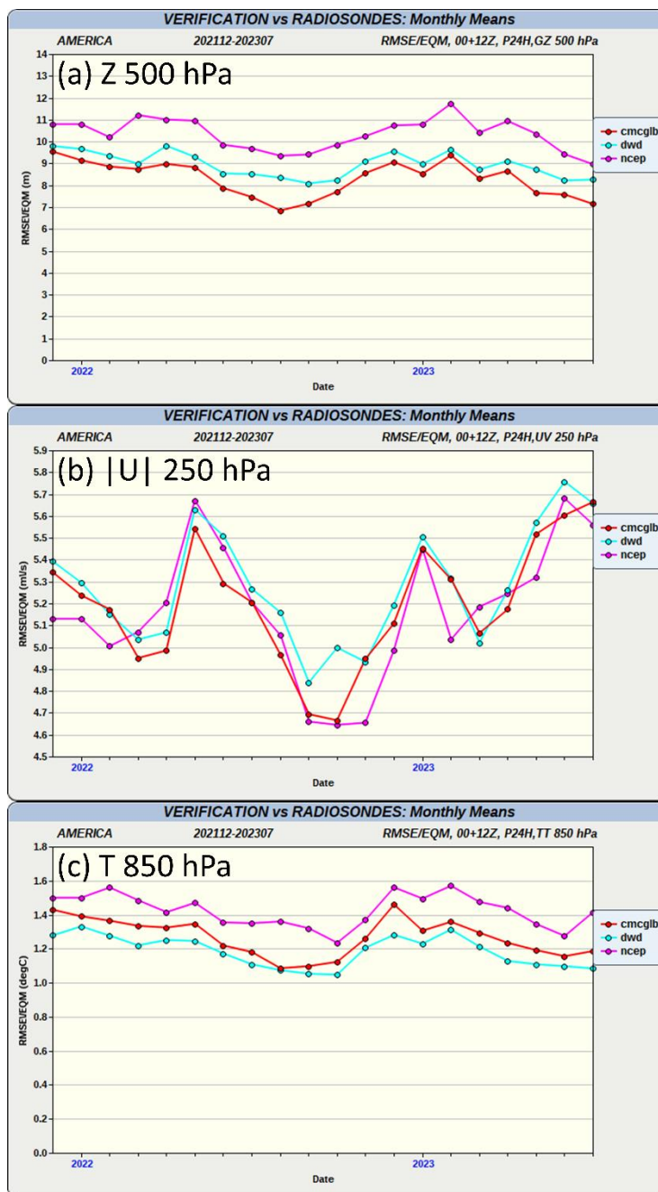
470 Figure 4: The RMS error of 24 h forecasts from the GDPS (in red) together with the same results from the German Weather Service (in light blue) and the U.S. National Centers for Environmental Prediction (in pink) computed with respect to the North American network of radiosonde observations for (a) geopotential height at 500hPa, (b) wind speed at 250hPa, and (c) temperature at 850hPa. (Note: a similar result, but only for 500hPa geopotential height is available on the public website: https://weather.gc.ca/verification/monthly_ts_e.html .)
