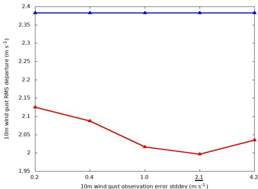
570 Figure 8: The red line shows the wind gust (10 m above the ground) RMS departure of the analysis from the withheld observations for different values of the specified observation-error stddev when using 10-fold cross-validation over a two-month period during the winter of 2020. The blue line shows the stddev of the observation departure from the HRDPS background state as measured using all of the wind gust observations.
