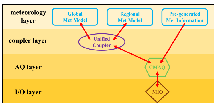
Figure 1. Synopsis of the Advanced Air Quality Modeling System (AAQMS). Arrows indicate the flow of information.
