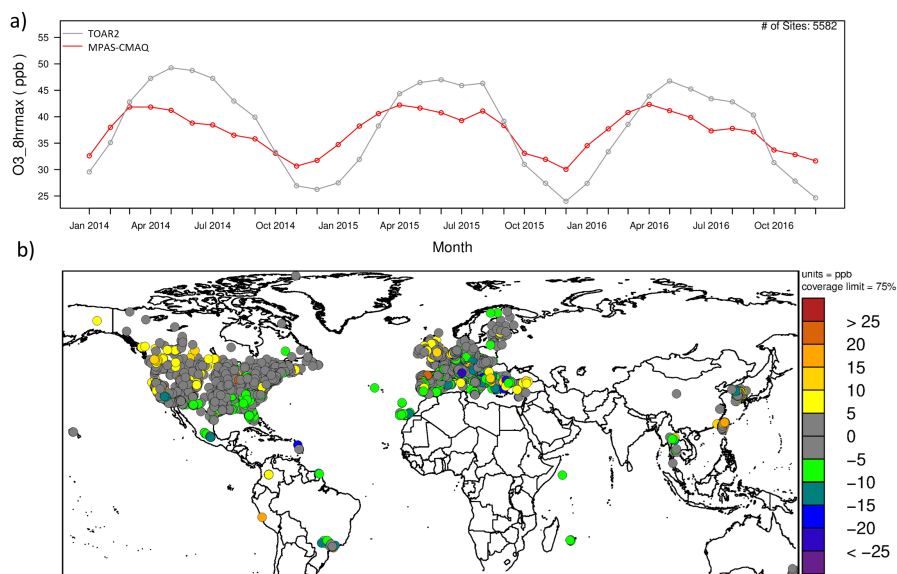
Figure 5. Modeled and observed surface ozone values for a) monthly average of all TOAR2 sites over time and b) average bias at each site for the three year period.
