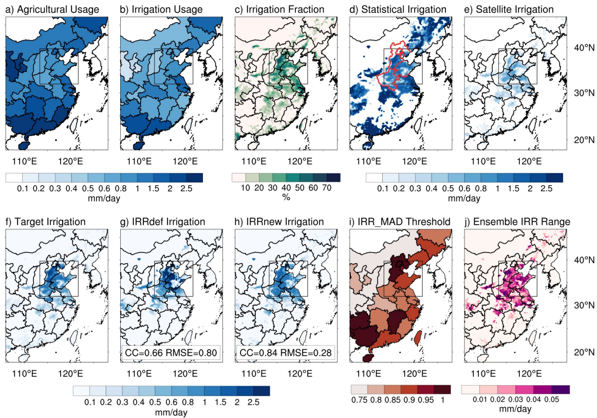
365 Figure 4. Spatial maps of 2005 (a) agricultural usage, (b) estimated irrigation usage, (c) irrigation fraction (same as Fig. 1d), (d) statistical irrigation, (e) satellite irrigation, (f) observation irrigation, (g) simulated irrigation using the default irrigation scheme (IRRdef), (h) simulated irrigation using improved irrigation scheme (IRRnew), (i) MAD (Manageable allowable deficit) irrigation threshold adopted in IRRnew and (j) irrigation range among 10 ensemble members using different initial conditions. For easy comparison, all subplots with blue colors (Fig. 4a,b,d,e,f,g,h) adopt the same color scale.
