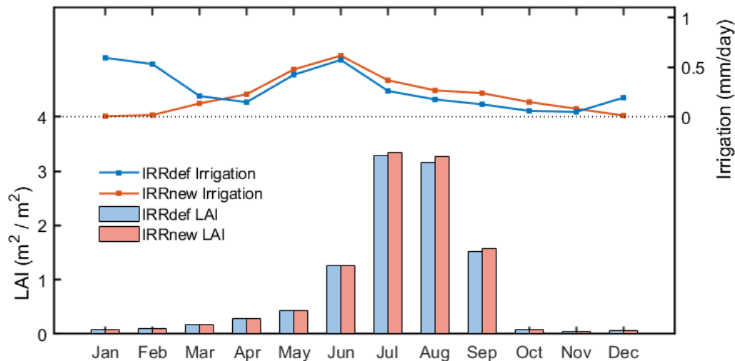
380 Figure 5. Monthly irrigation (lines) and LAI (bars) using default irrigation scheme (IRRdef) and improved irrigation scheme (IRRnew). Monthly values are the average of all crop grids in the NCP over the period of 2005-2014.
