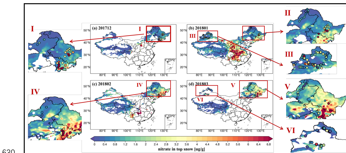
Figure 9. Spatial distribution of nitrate concentration in the top snow layer observed and simulated by WRF-Chem across China from December 2017 to March 2018. [Note: The background color in each figure represents the monthly average of the simulation results, while all the observations for each month are embedded in each panel.]
