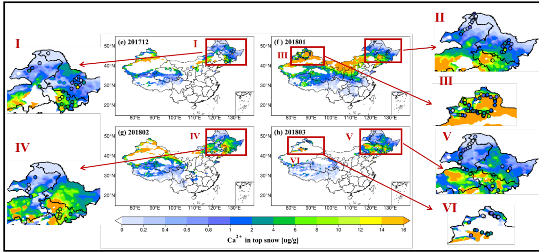
470 Figure 6. Spatial distribution of calcium ion concentrations (µg/g) in the top snow layer simulated by WRF-Chem, with field campaign observations embedded at specific locations for each month (e–h) across China from December 2017 to March 2018.
