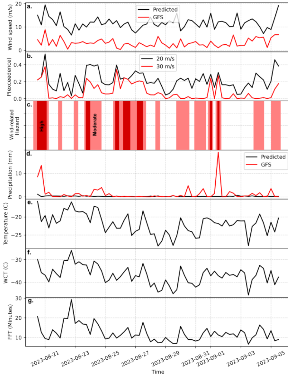
Figure 9. Example of real-time forecast for wind(a.), precipitation (d.), temperature (e.), as well as derivate variables of wind chill temperature (f., WCT) and facial frostbite time (g., FFT; Moore and Semple, 2011). The raw GFS estimates of wind speed and precipitation are shown in red alongside our predictions, note how the AtmOS wind speed estimates are substantially higher and precipitation substantially higher. The probability of exceedance of different wind speed thresholds, 20 and 30 m/s, is also shown in (b.), with related hazard classification with medium hazard denoted as >20% probability of winds exceeding 20 m/s and high hazard as >20% probability of winds exceeding 30 m/s.
