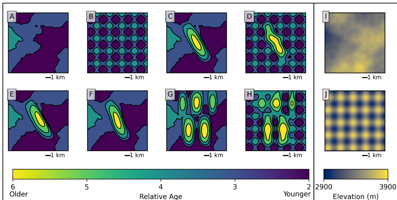
Figure 6: (A-H) Geologic maps of synthetic models colored by the relative age of the units: A) Flat model, B) Flat model with egg-box topography, C) Single symmetric anticline model, D) Single symmetric anticline model with egg-box topography, E) Asymmetric anticline, F) Sigmoidal anticline, G) Multiple folds, H) Multiple folds with egg-box topography. (I-J) Topography used in the models: (I) is the Perlin-noise based topography, and (J) is the egg-box topography.
