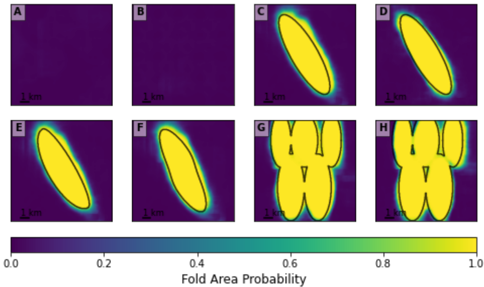
380 Figure 10: Fold area detection by the convolutional neural network supervised learning method for the synthetic maps in Figure 6. Colors indicate the probability of each pixel being within the area of the fold (including the axis).
