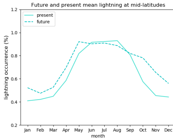
Figure 9. Mid-latitude Northern mid-latitude seasonal mean in lightning occurrence (%) in the present (solid line, 2017-2019) and future (dashed line, 2098-2100) in SSP5-8.5.
