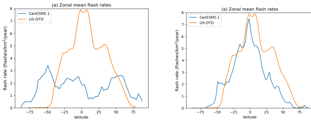
Fig 2: Zonal evaluation of lightning flash rates. (left) Figure 5a from the original manuscript, (right) after the CAPE standardisation correction.
