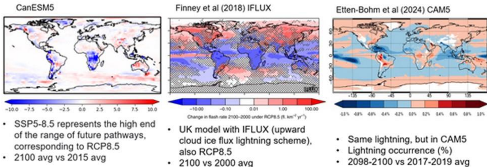
Fig AR1(b): future minus present changes in lightning: our study, vs two other studies.
