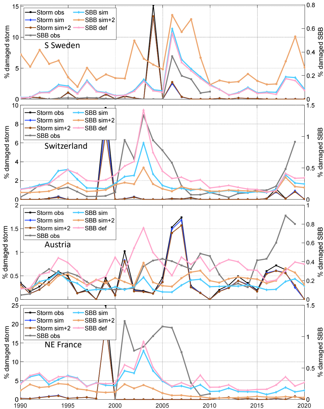
Figure 6: Sensitivity test of modelled storm and spruce bark beetle damage for temperature and model environment. Model output from the calibrated stand-alone version with tree structure and storm damage input from the default LPJ-GUESS run (def, “All4 opt” in Fig. 3) and the calibrated model run with LPJ-GUESS with normal climate (SBB sim) and with +2 ° temperature (sim+2) compared to observations (obs).
