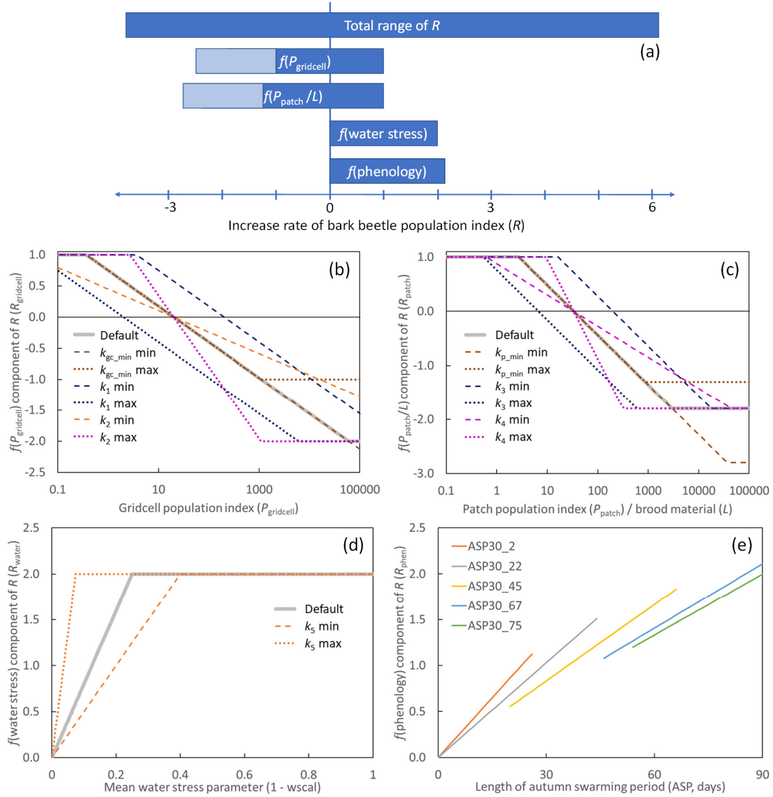
Figure 1: The different components of the increase rate of the bark beetle population index ( R ). (a) Ranges of the components and the total (Eq. 4). For f(P_{\text{gridcell}}) and f(P_{\text{patch}}/L) , the light shaded areas show the part of the ranges that were varied in the parameter optimization, where the sum of the minimum of f(P_{\text{gridcell}}) and f(P_{\text{patch}}/L) were kept constant to have the possible total negative feedback from the population index constant (see section 2.6). (b-e) Shape of the functions for the components of the increase rate of the bark beetle population index ( R ), b Eq. 7, c Eq. 8, d Eq. 10, e Eq. 12. The default parameter setting (Table 7) is shown by thick grey lines (b-d). The functions are also shown in colour for the min and max value of parameters included in the calibration and sensitivity analysis (section 2.6), using the default setting for the other parameters. For f(\text{phenology}) , (e), no parameters were tested but the response depends on the grid-cell's 30-year running mean of the length of the autumn swarming period (ASP, ASP30) and function are shown for ASP30 from 2 to 75 days.
