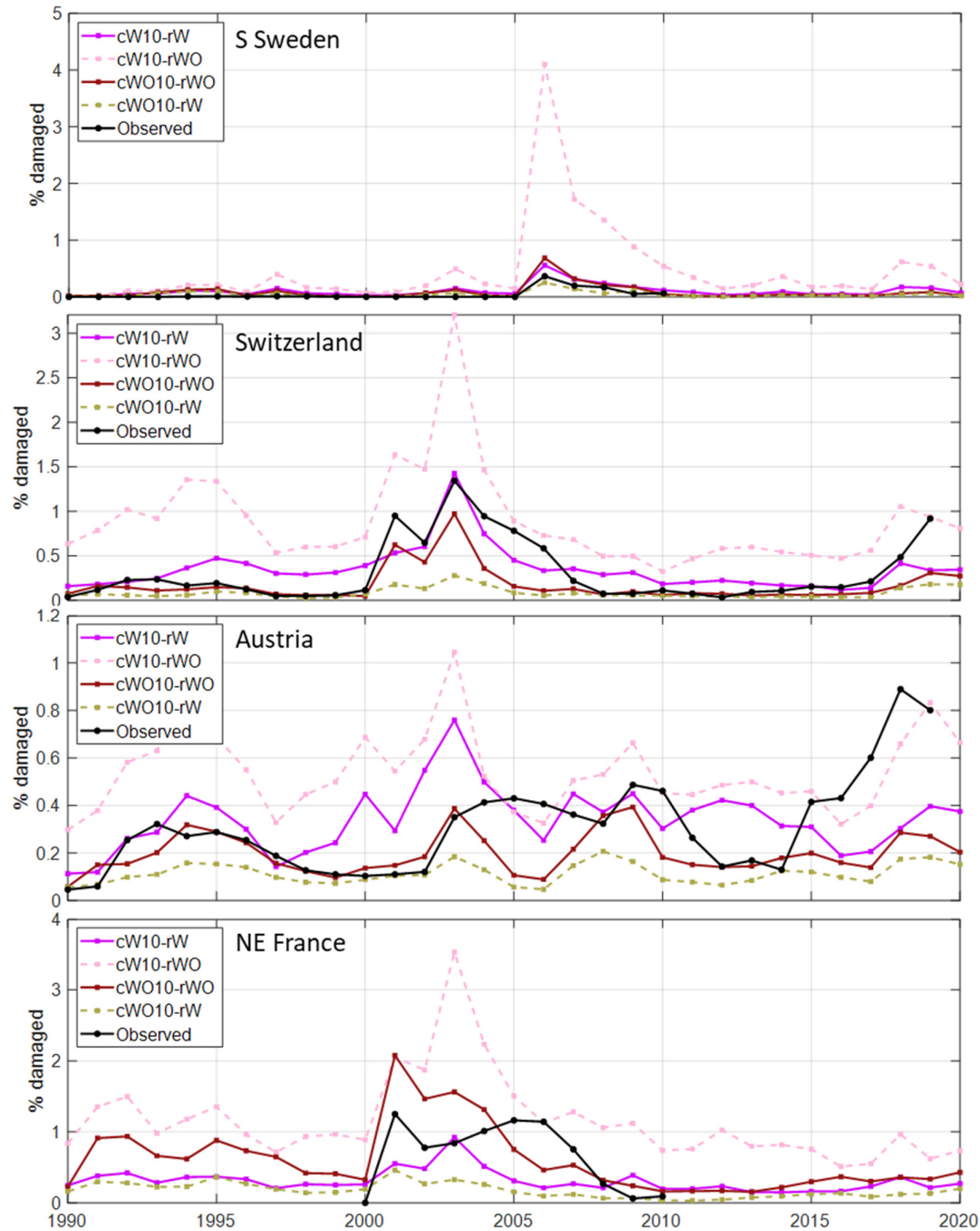
425 Figure 5: Test of the sensitivity of including salvage cutting of storm felled trees and sanitary cutting of infected trees (SSC) for the fraction of SBB killed trees. The calibrations with (cW) and without (cWO) SSC using calibration data for 1990-2010 (10) were run both with (rW) and without (rWO) SSC. In Fig. S5, the calibrations also including 2011-2019 data for Austria and Switzerland are shown.
