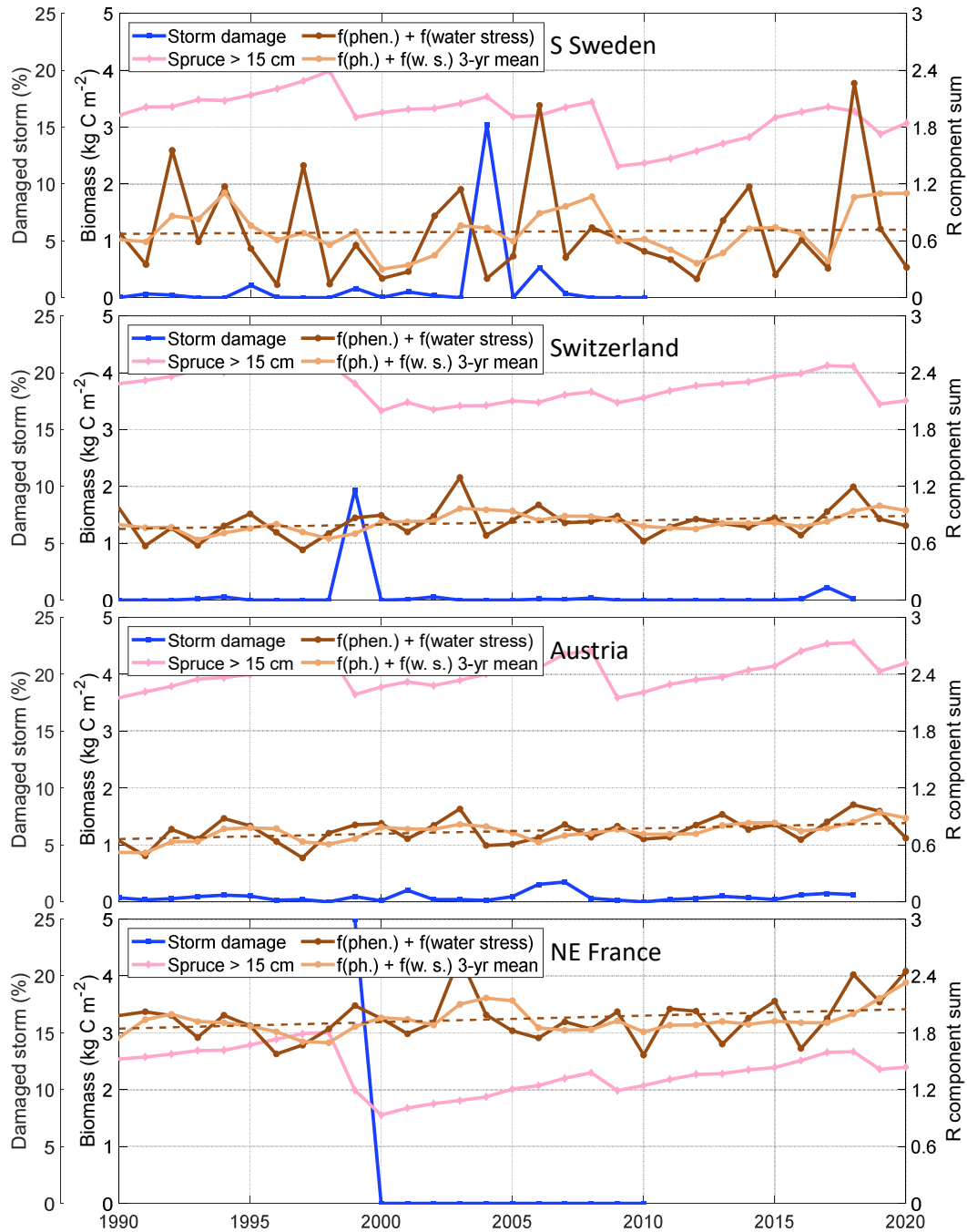
Figure 7: Sensitivity for SBB outbreak divided in predisposing (biomass of spruce trees with a diameter larger than 15 cm), triggering (fraction of spruce volume damaged by storm) and contributing (the sum of the phenology and water stress related components for the increase rate of the bark beetle population index, R Eq. 4) factors. For the phenology and water stress R components sum the running 3-year mean and the trend over time (dashed line) are also shown.
