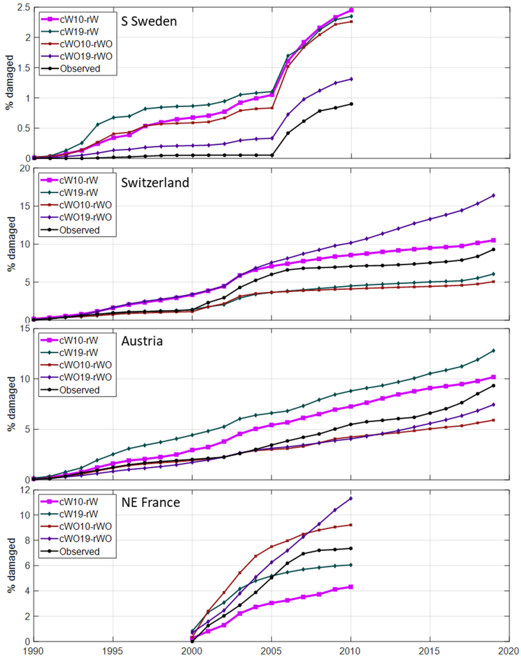
Figure 4: Accumulated fraction of simulated and observed spruce forest damaged by SBB over the period with observations. Calibrations are shown using only data up until 2010 (10) and also including data for Switzerland and Austria 2011-2019 (19) as well as with (W) or without (WO) salvage and sanitary cutting. The main base run setting, cW10-rW, is showed by bold line.
