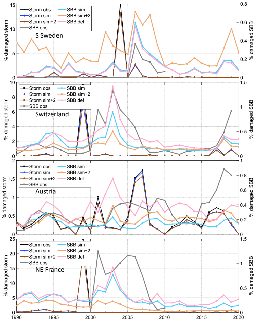
460 Figure 6: Sensitivity test of modelled storm and spruce bark beetle damage for temperature and model environment. Model output from the calibrated stand-alone version with tree structure and storm damage input from the default LPJ-GUESS run (def, "All4 opt" in Fig. 3) and the calibrated model run with LPJ-GUESS with normal climate (SBB sim) and with +2 ° temperature (sim+2) compared to observations (obs).
