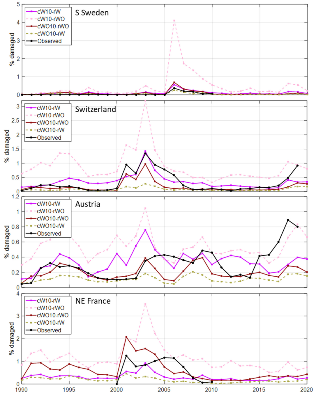
Figure 5: Test of the sensitivity of including salvage cutting of storm felled trees and sanitary cutting of infected trees (SSC) for the fraction of SBB killed trees. The calibrations with (cW) and without (cWO) SSC using calibration data for 1990-2010 (10) were run both with (rW) and without (rWO) SSC. In Fig. S5, the calibrations also including 2011-2019 data for Austria and Switzerland are shown.
