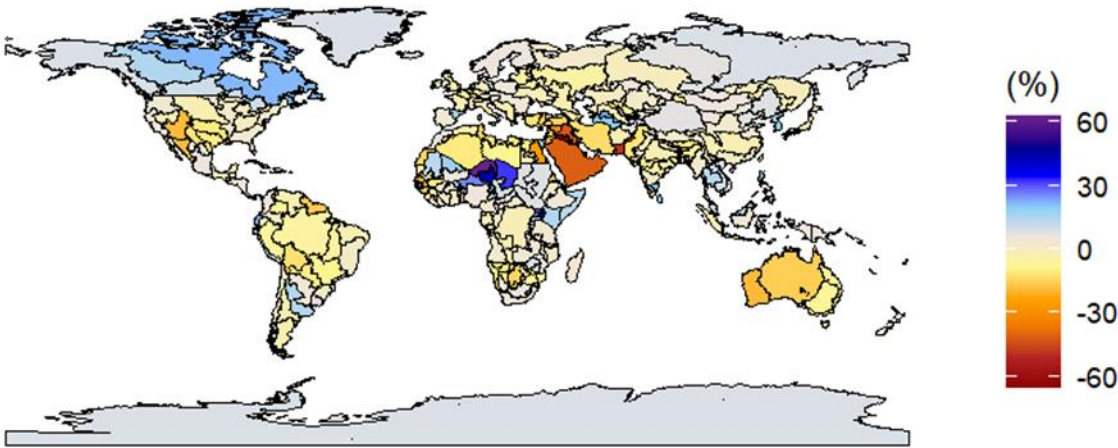
385 Figure 3: Runoff change between 2010 and 2050 based on CWatM simulations using average climate forcing data from 4 GCMs under RCP6.0
