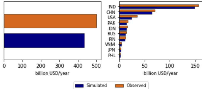
Figure 4: (a) The simulated and observed total water withdrawals by sector and water source at the global scale in 2010 and the ten countries with highest withdrawals. (b) The simulated and observed irrigated area at the global scale in 2010 and the ten countries with highest irrigated areas. (c) The simulated and observed agricultural income at the global scale in 2010 and the ten countries with the highest agricultural incomes. Full names for countries are provided in Table A2 in the appendices. Crop full names are:
