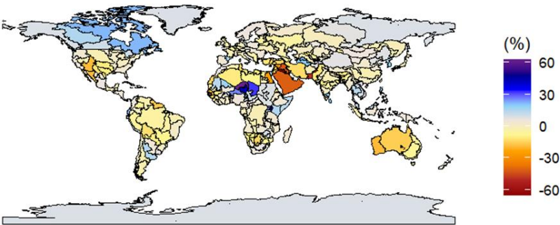
390 Figure 3: Runoff change between 2010 and 2050 based on CWatM simulations using average climate forcing data from 4 GCMs under RCP6.0
