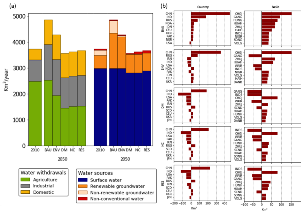
555 Figure 5: (a) Global water withdrawals by water use sector and water source for each scenario. (b) Ten countries (left column) and basins (right column) with highest change in withdrawals between 2010 and 2050 for each scenario. Non-conventional water includes both desalinated water and treated wastewater. Full names for countries and basins are provided in Table A2 in the appendices.
