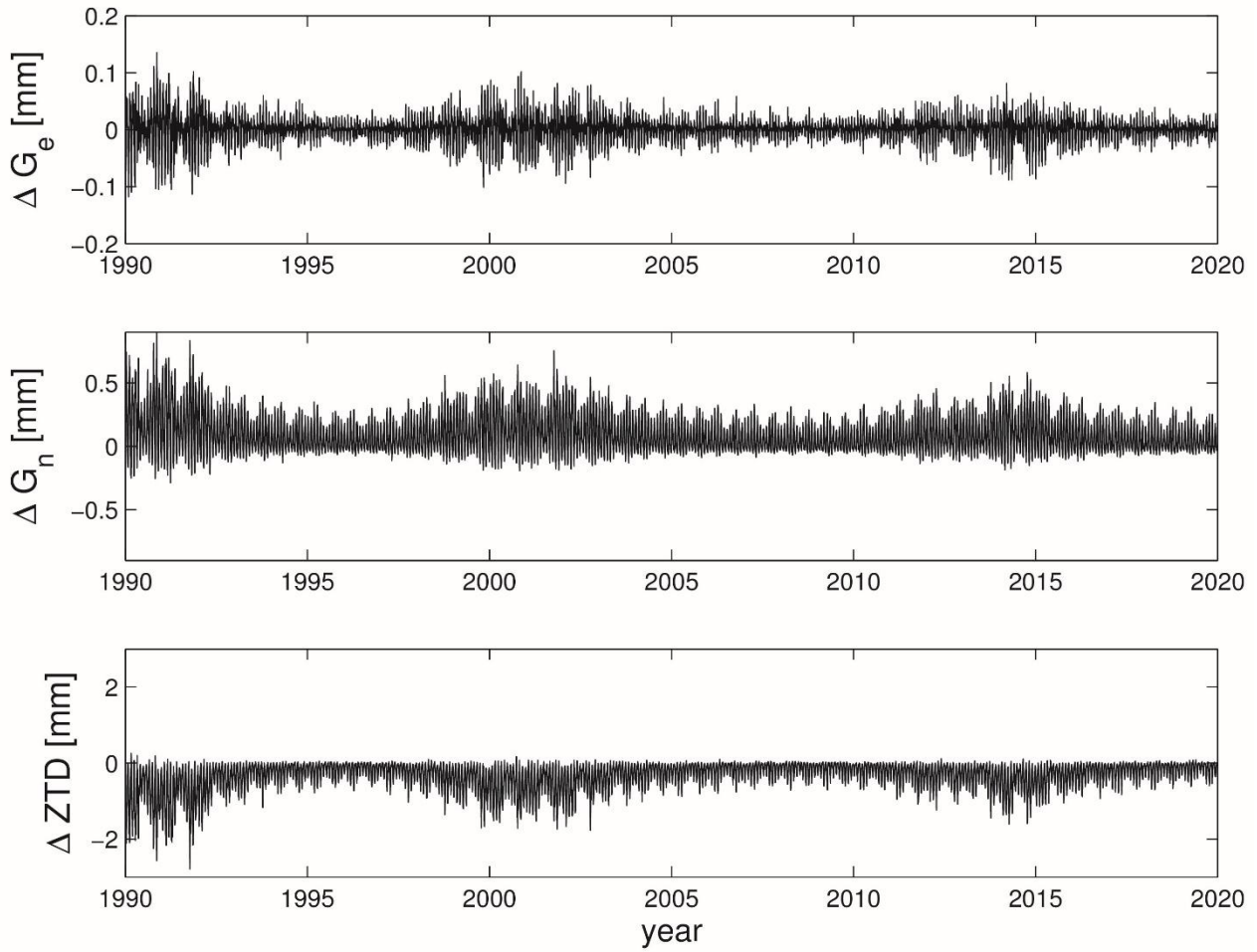
525 Figure 11: Impact of higher-order ionospheric corrections on estimated zenith delays and tropospheric gradient components in PPP for one station in China (Wuhan) (Year 1990-2019). Each month consists of one day only (15 th day of each month). Each day consists of 24 epochs (1h resolution).
