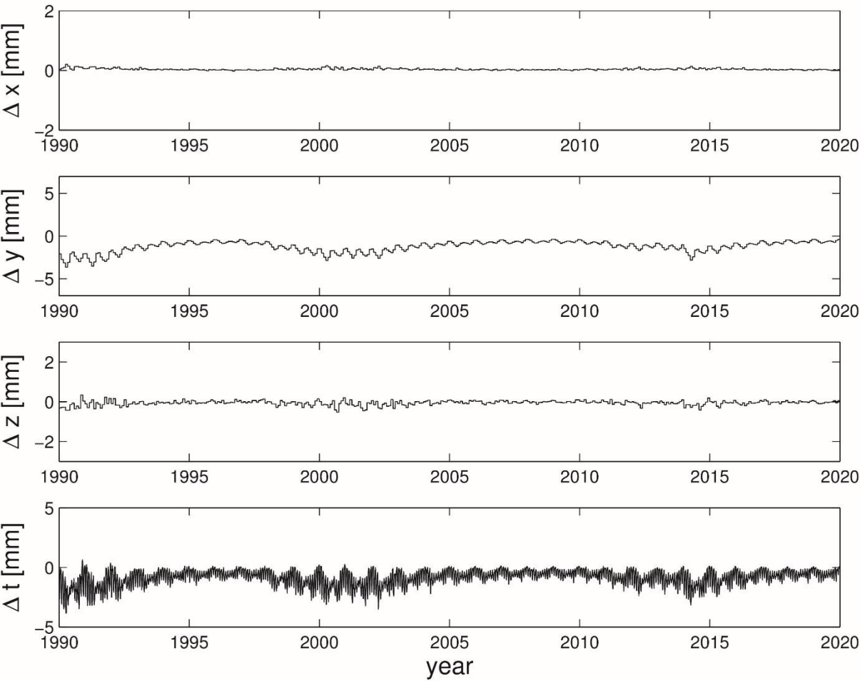
520 Figure 10: Impact of higher-order ionospheric corrections on the estimated station coordinate and clock (expressed in mm) in PPP for one station in China (Wuhan) (Year 1990-2019). Each month consists of one day only (15 th day of each month). Each day consists of 24 epochs (1h resolution).
