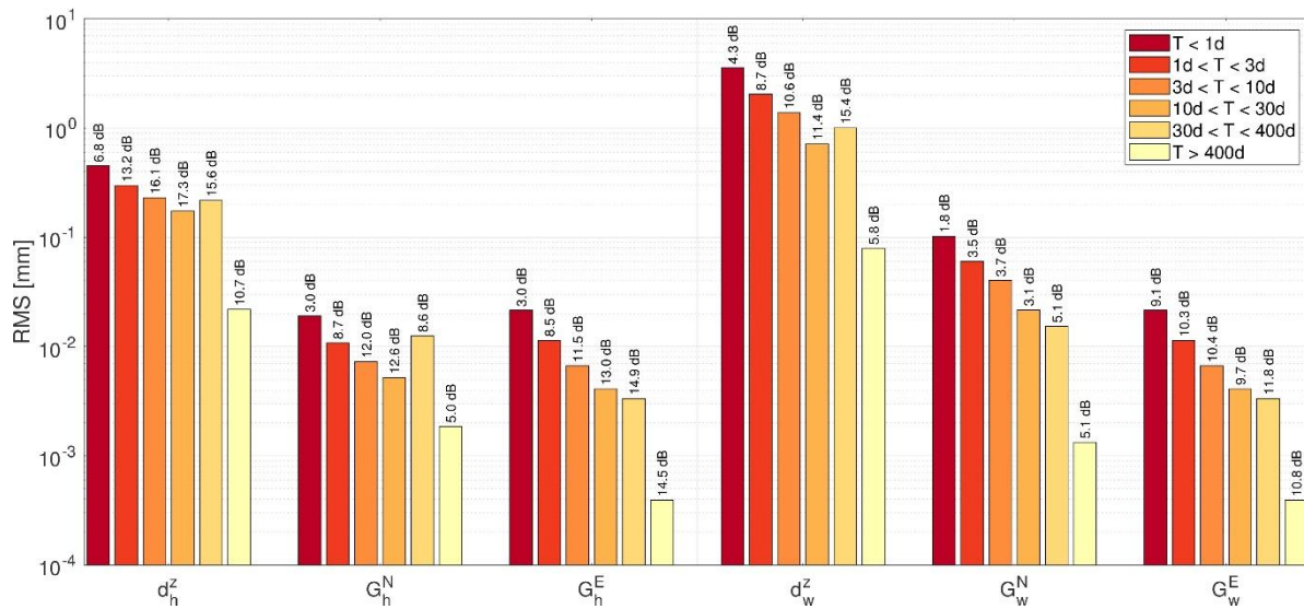
405 Figure 5: Root mean square of band-pass-filtered atmospheric delay coefficient differences between IFS and ERA5 employing DNS for the station Wettzell (Germany).
