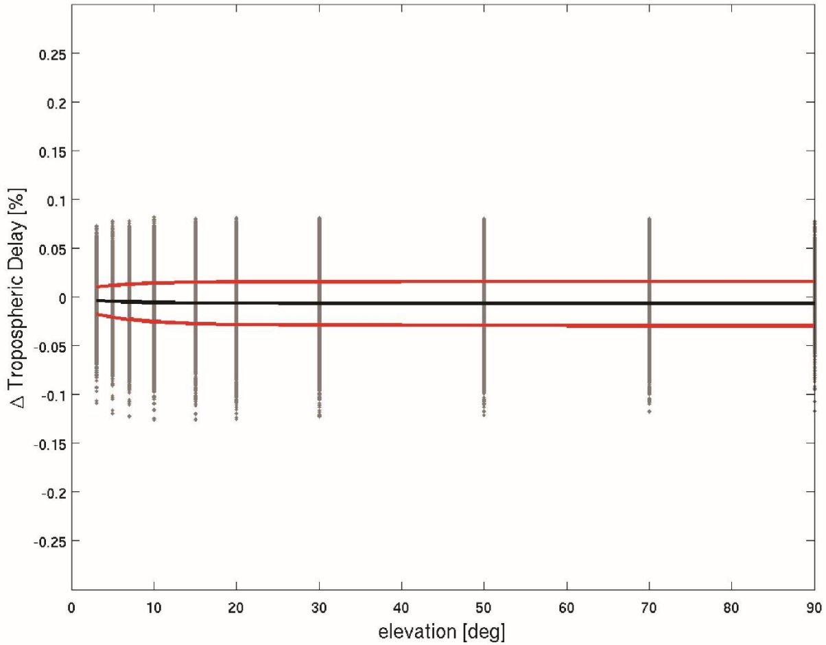
355 Figure 3: Relative differences of tropospheric delays between RADIATE and DNS as a function of the elevation angle (15 February 2024, 12UTC). We consider 2592 globally distributed grid point coordinates and compute 120 tropospheric delays per grid point. The black line shows the mean deviation and the red lines show the one-sigma deviation around the mean deviation.
