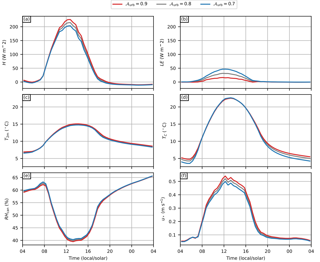
Figure 4. Diurnal cycles of the sensitivity test target variables (a) sensible heat flux H , (b) latent heat flux LE , (c) 2-metre air temperature T_{2m} , (d) area-weighted total urban surface temperature T_C , (e) canyon relative humidity RH_{\text{can}} , and (f) total friction velocity u_* , presented for three different urban fractions \mathcal{A}_{\text{urb}} .
