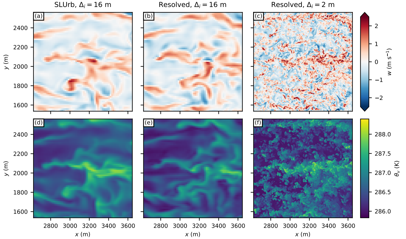
Figure 9. Instantaneous (x, y) cross sections of model vertical velocity w (a-c) and virtual potential temperature \theta_v (d-f) over the analysis area from a model level closest to z = 42 m at 12:00 (solar noon). The cross sections are presented for SLUrb at 16 m grid resolutions (a and d) and for the resolved urban canopy at 16 m and 2 m grid resolutions (b, e and c, f respectively).
