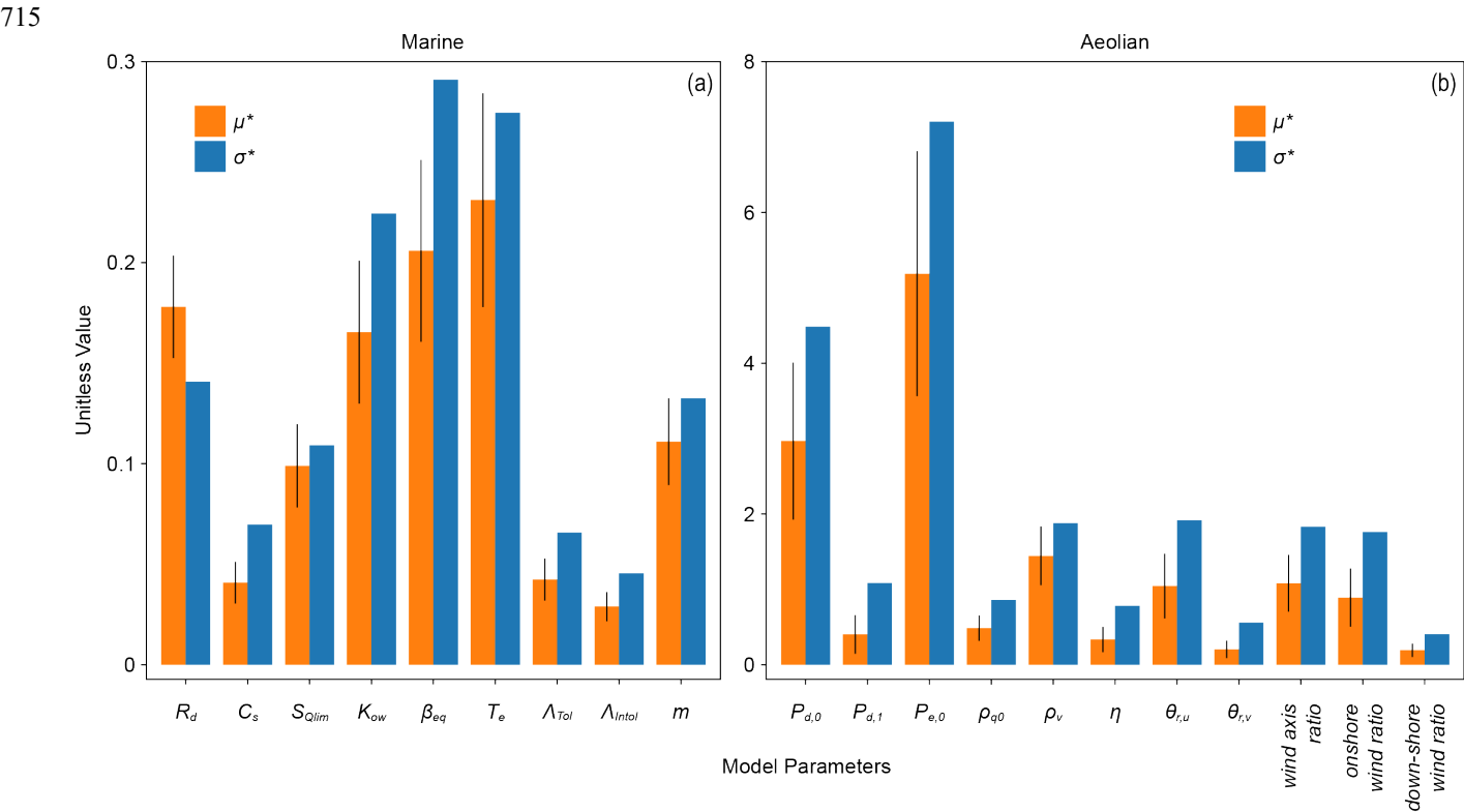
720 Figure 7: Sensitivity analyses of model parameters for the (a) Marine and (b) Aeolian model components. Marine and aeolian parameters are analyzed separately following the same design and parameter ranges as the parameter calibration simulations. Unitless values for the overall importance of a parameter ( \mu^* ) and its degree of interaction with other parameters ( \sigma^* ) are given in orange and blue, respectively. Black lines represent the 95% confidence interval.
