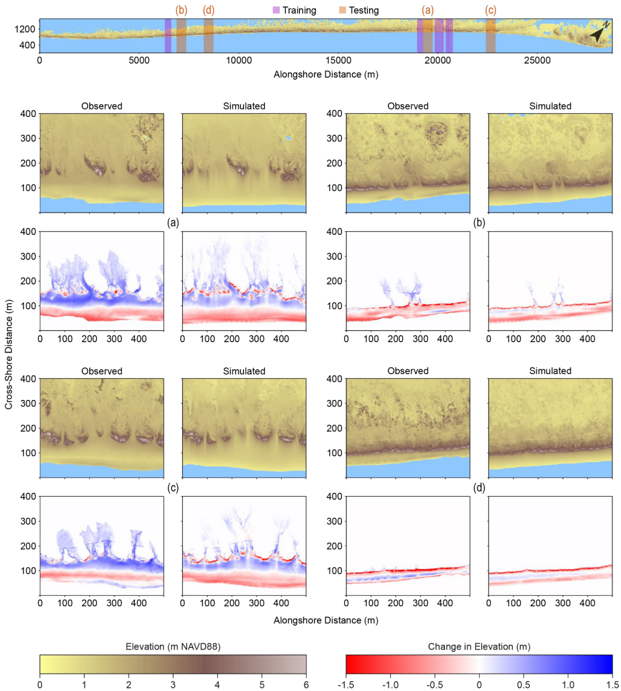
Figure 5: Hindcast simulations testing MEEB performance with calibrated marine parameters. (a-d) Observed and simulated post-Florence elevation and pre- to post-Florence elevation change at 4 test locations across North Core Banks, NC, USA. Locations of each marine testing site, as well as each marine training site used in calibration, are indicated in the top map. Skill scores for each hindcast (a-d) are given in Table 3.
