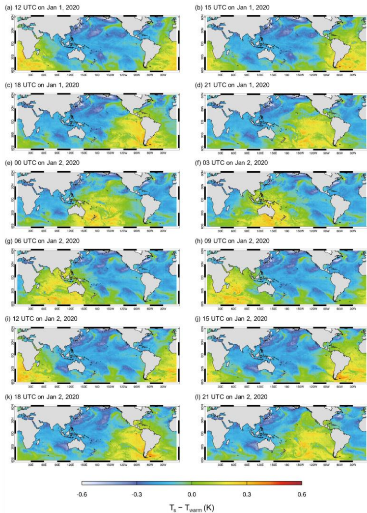
600 Figure 7. Same as in Fig. 4 but for T_s simulated with the revised OML model.
