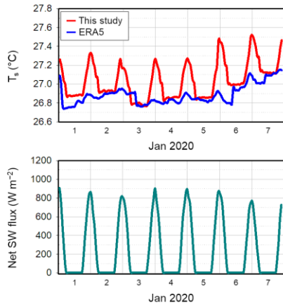
605 Figure 9. Time series of T_s from the model simulations and ERA5 (top panel of each figure), and ERA5 surface net solar radiation flux (bottom panel of each figure), for a week period from January 1 to 7, 2020, at four locations: (a) 20°S 80°E, (b) 20°N 180°, (c) 0° 155°W, and (d) 30°S 120°W.
