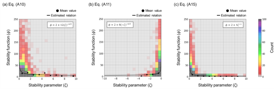
610 Figure B1. Scatterplots of stability functions ( \Phi ) vs stability parameters ( \zeta ), derived from ATLAS buoy measurements at 0^\circ and 140^\circ\text{W} in the period from 2001 to 2020. The color scale is for the data count, and the obtained \Phi - \zeta relations are given with black solid lines. (a) Eq. (A10), (b) Eq. (A11), and (c) Eq. (A15), respectively.
