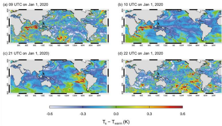
Figure 5. Same as Fig. 4, but given in hourly departures at (a) 09 UTC, (b) 10 UTC, (c) 21 UTC, and (d) 22 UTC 1 January 2020.
