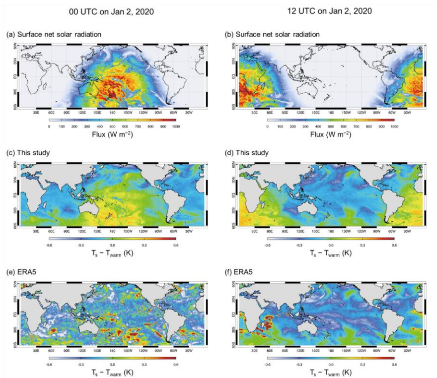
Figure 8. Geographical distributions of (a–b) surface net solar radiation flux from ERA5 and T_s hourly variations from (c–d) the revised OML model and (e–f) ERA5 at 00 UTC (left panels) and 12 UTC (right panels) on 2 January 2020.
