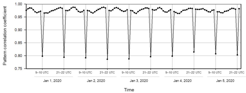
Figure 6. Time series of the pattern correlation coefficient for ERA5 T_e variations over the global ocean between two consecutive hourly distributions (between n th and n+1 st hourly data, expressed as n-n+1 UTC), in the period from January 1 to January 5, 2020. Only 9–10 UTC and 21–22 UTC are given as labels.
