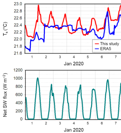
605 Figure 9. Time series of T_s from the model simulations and ERA5 (top panel of each figure), and ERA5 surface net solar radiation flux (bottom panel of each figure), for a week period from January 1 to 7, 2020, at four locations: (a) 20°S 80°E, (b) 20°N 180°, (c) 0° 155°W, and (d) 30°S 120°W.
