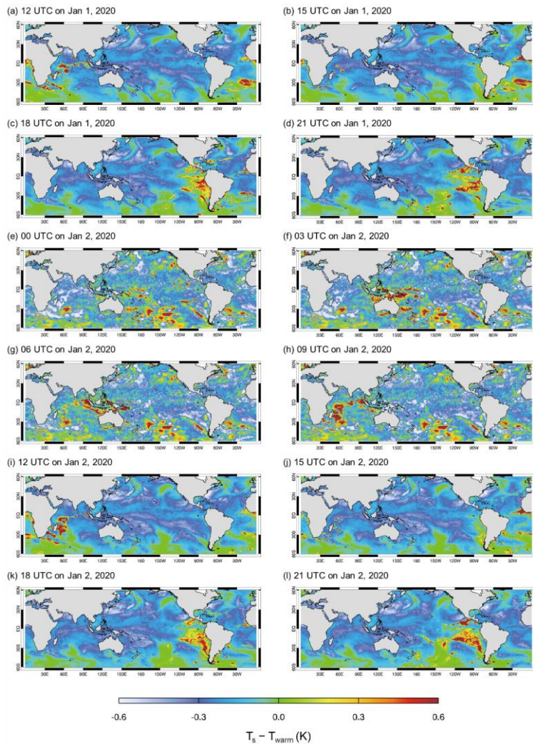
590 Figure 4. Geographical distributions of hourly variations in ERA5 T_s from 12 UTC 1 January to 21 UTC 2 January in 2020 with a 3-hour interval. Values are given in departures of ERA5 ocean skin temperature from ERA5 SST (i.e., T_s - T_{\text{warm}} ).
