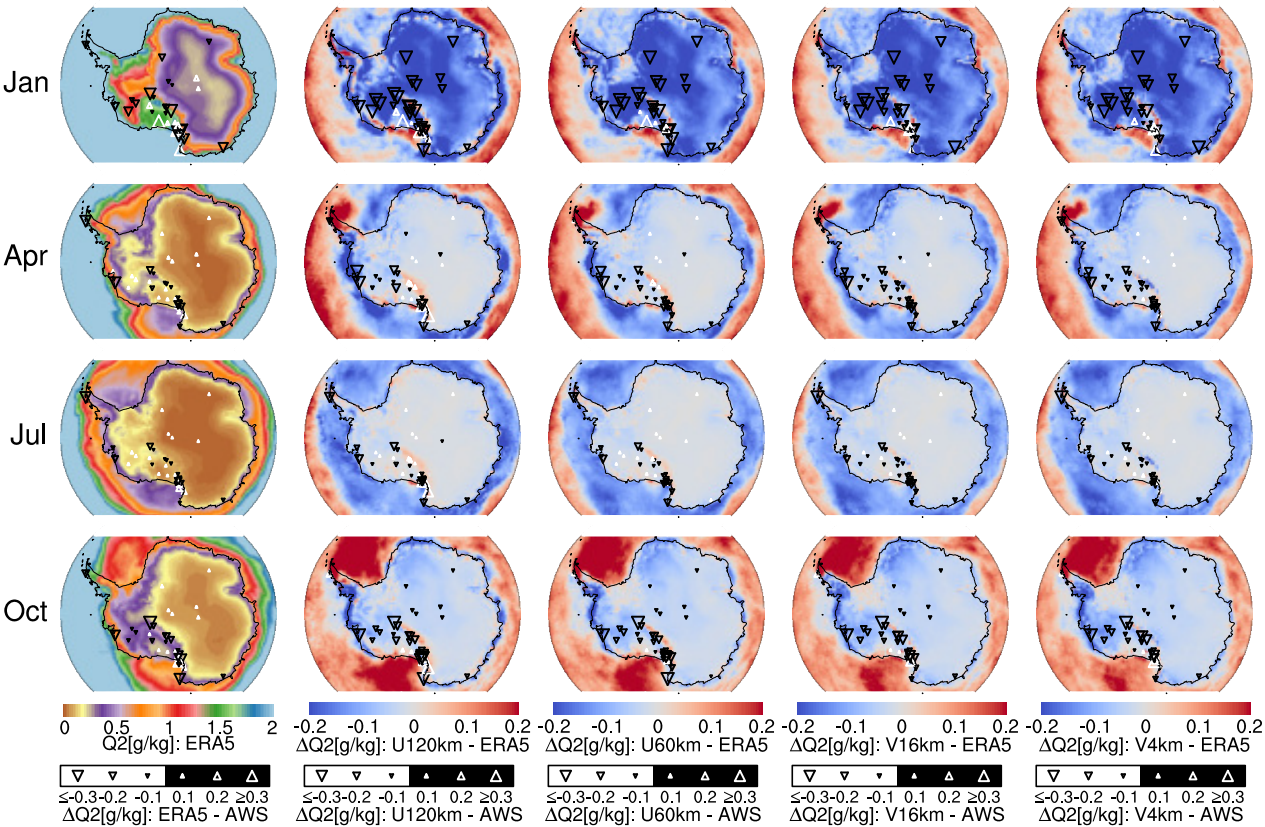
Figure 6. As Fig. 3 but for 2-m specific humidity ( Q2 [g \text{ kg}^{-1}] ). Number of stations: 32 (January), 34 (April), 35 (July), 35 (October).
