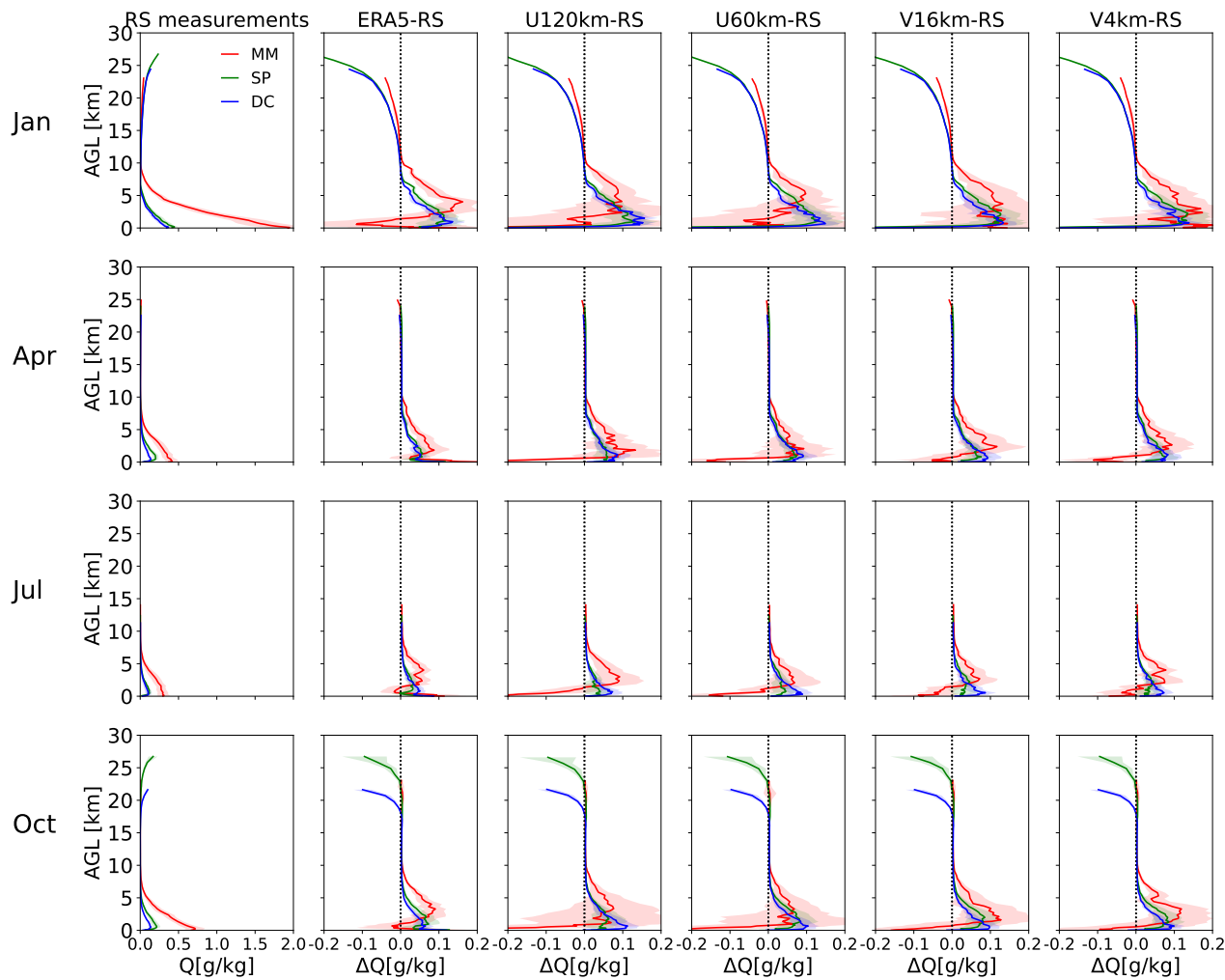
Figure 10. As Fig. 8 but for specific humidity ( Q [ \text{g kg}^{-1} ]) profile.
