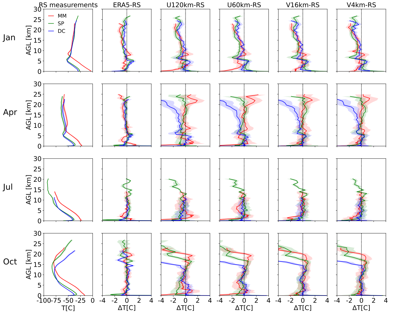
Figure 8. The first column displays the monthly medians of radiosonde-measured temperature ( T [°C]) profiles. The five rightmost columns present the monthly median temperature biases ( \Delta T [°C]) for ERA5 and iAMAS (U120km, U60km, V16km, and V4km) compared to radiosonde measurements. The shading represents the standard error.
