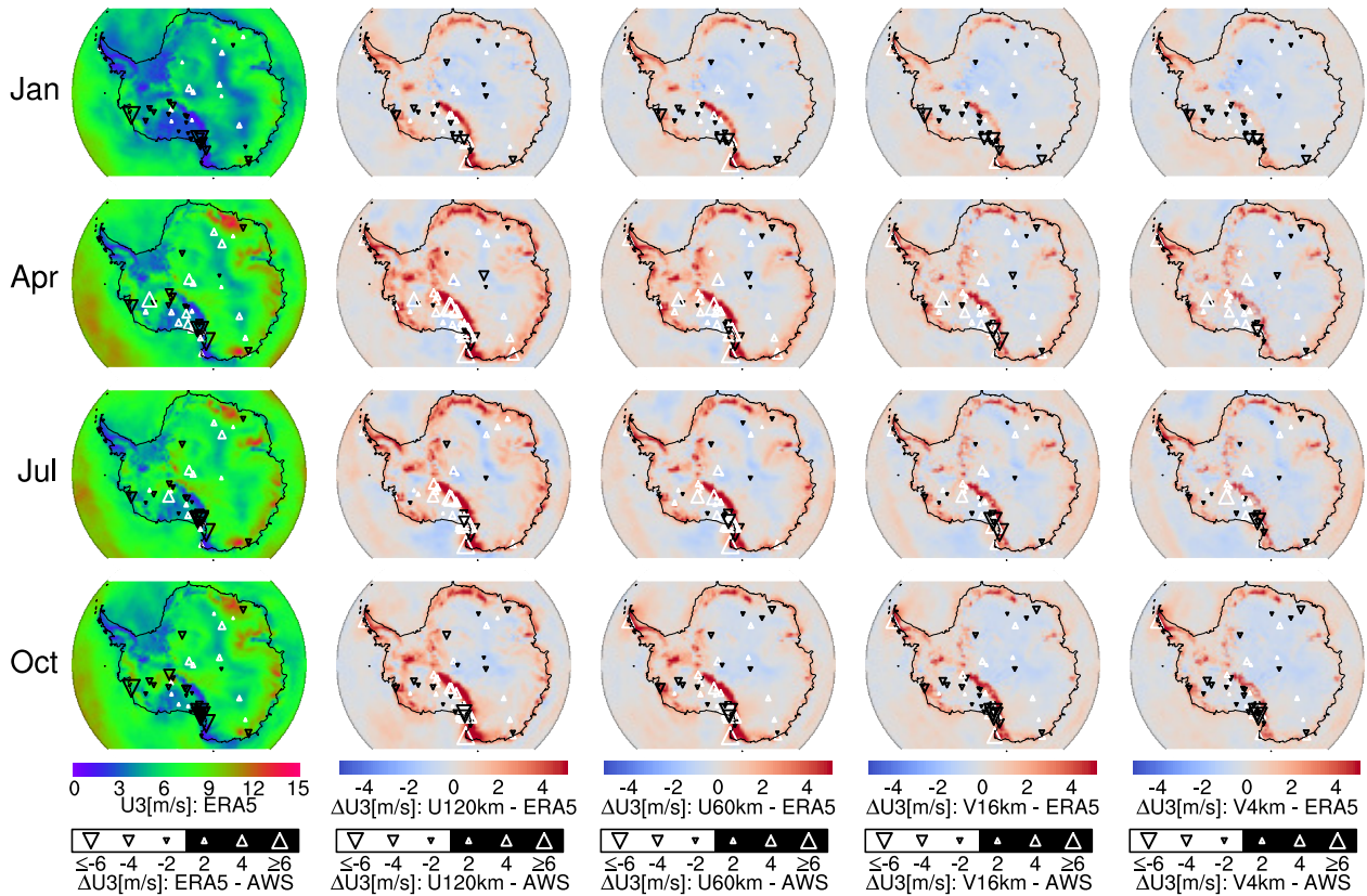
Figure 7. As Fig. 3 but for 3-m wind speed ( U3 [ \text{m s}^{-1} ]). Number of stations: 41 (January), 42 (April), 41 (July), 47 (October).
