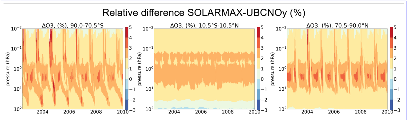
Figure 2. Impact of SSI changes on ozone in ICON-Linoz-ICON-ART (Percentage difference between SOLMAX and UBC-NO y relative to SOLMAXUBC-NO y ). From left to right: 70-90°S, 10°S-10°N, 70-90°N respectively.
