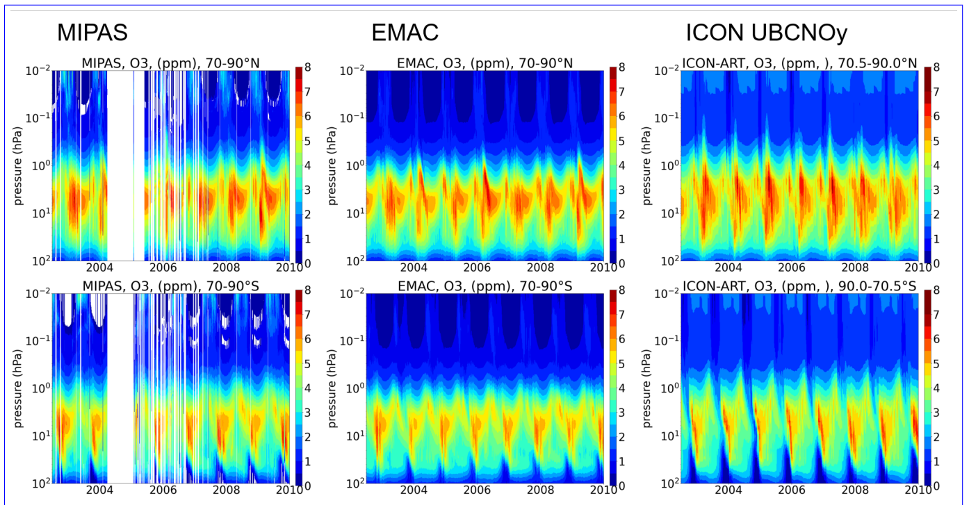
Figure 6. Daily mean, area weighted ozone after inclusion of the \text{NO}_y -based tendency in 70-90°N (top) and 70-90°S (bottom) from (left) MIPAS/ENVISAT v5, (middle) EMAC, and (right) ICON UBC- \text{NO}_y . The EMAC and MIPAS data are from Sinnhuber et al. (2018).
