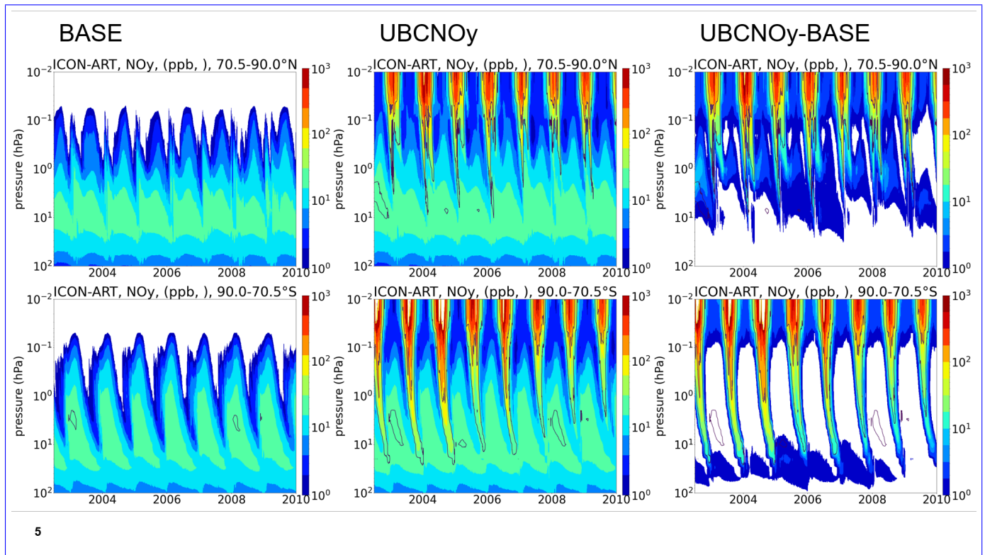
Figure 1. Daily mean, area-weighted NO y in 70-90°N (top) and 70-90°S (bottom) from ICON-ART. Left: experiment 1 (BASE), Middle: experiment 2 (UBC-NO y ), and Right: difference (UBC-NO y - BASE). Model runs are shown in 2002.5-2010 only to allow for 2.5 years of spin-up.
