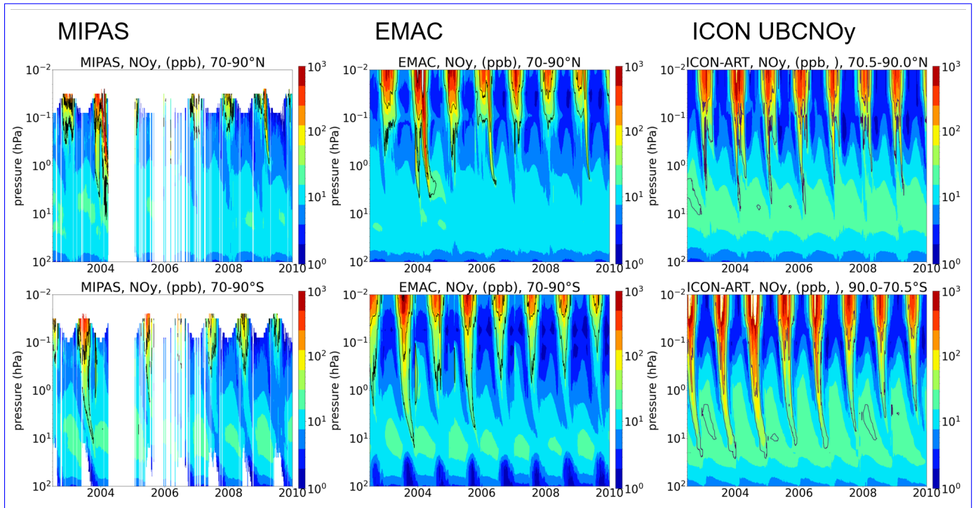
Figure 4. Daily mean, area-weighted \text{NO}_y in 70\text{--}90^\circ\text{N} (top) and 70\text{--}90^\circ\text{S} (bottom) from (left) MIPAS/ENVISAT v5, (middle) EMAC, and (right) ICON-ART (UBC- \text{NO}_y ). EMAC and MIPAS data are from Sinnhuber et al. (2018).
