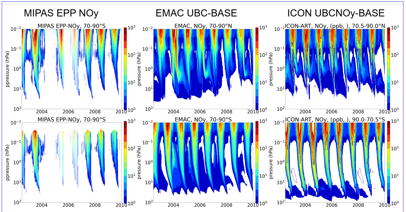
Figure 5. Daily mean area-weighted EPP-NO y . Left: MIPAS/ENVISAT v8, —courtesy (Funke et al., 2023) v5 adapted from (Sinnhuber et al., 2018) ; Middle: EMAC, difference from model run with UBCNO UBC-NO y to base run without UBCNO UBC-NO y but identical in every other respect (Sinnhuber et al., 2018); right: ICON UBCNO UBC-NO y -BASE.
