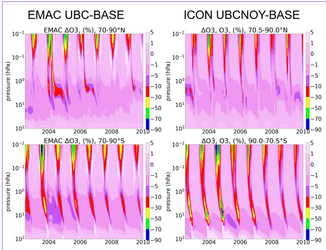
Figure 7. Daily mean area-weighted ozone change due to EPP-NO y in percentage in 70-90°N (top) and 70-90°S (bottom) from (left) EMAC Sinnhuber et al. (2018), and (right) ICON-ART. The contour intervals are the same as in Sinnhuber et al. (2018) (figures 12 and 13).
