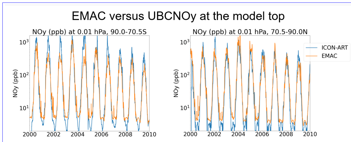
Figure 3. Daily mean, area weighted NO y in at 0.01 hPa in 70-90°S (left) and 70-90°N (right) from the chemistry-climate model ICON-ART (experiment 2, UBC-NO y ) and EMAC model results from Sinnhuber et al. (2018)., also using the NO y upper boundary condition of Funke et al. (2016).
