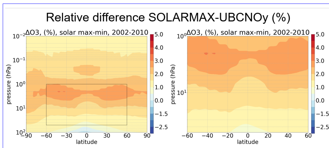
Figure 8. Impact of solar spectral irradiance (SSI) on ozone in ICON-ART: Percentage difference between SOLMAX and UBC-NO y relative to UBC-NO y (left). Same, but with pressure and latitude range adapted to ozone solar signal figures (two different datasets (SAGEII/SBUV)) in Maycock et al. (2016) (right).
