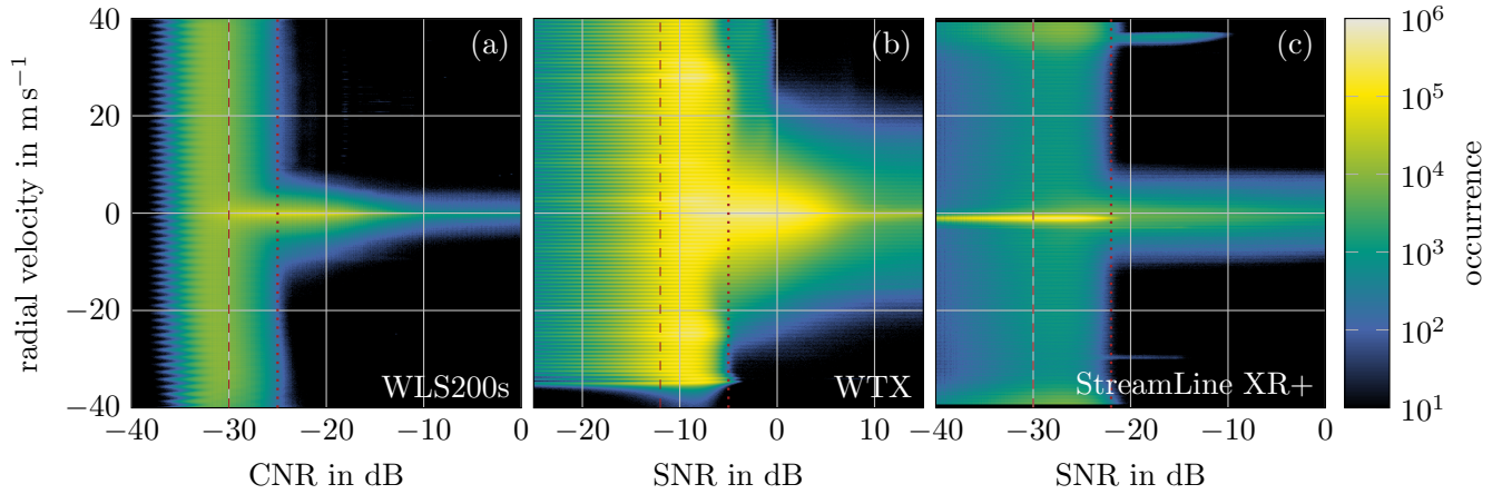
Figure 8. Occurrence of radial velocities for different \text{SNR}-\text{CNR} values for WLS200s at Payerne (a), WTX at Villingen-Schwenningen (b), and StreamLine XR+ at Neumayer Station (c). All radial velocities are summed up in bins of 0.1 dB and 0.1 \text{m s}^{-1} between June and August 2023 for (a) and (b), and between 3 rd January 2024 and 26 th November 2024 for (c). The selected conservative CNR thresholds are marked dotted, the weak thresholds dashed.
