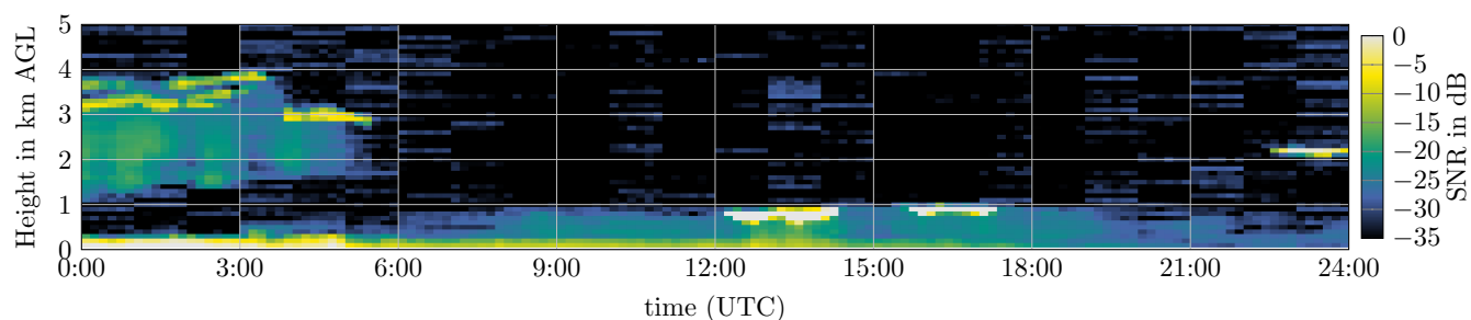
Figure D2. Doppler lidar SNR at Neumayer Station on 19 th May 2024. The Median of the SNR values of all measurements available per bin is displayed.
