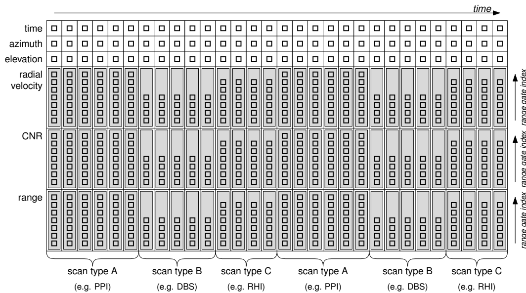
Figure 1. Visualization of typical scan patterns employed for wind profile retrieval. The respective range gate centres of all beams in the cone are mapped to the same heights, as typical for PPI and DBS scans. In contrast, the associated height of the range gate centres in RHI scans depend on the elevation angle, which is displayed on the plane. Retrieving the wind vector based on height bins enables the consideration of all measurements within the considered time period and, therefore, maximizes the data availability.
