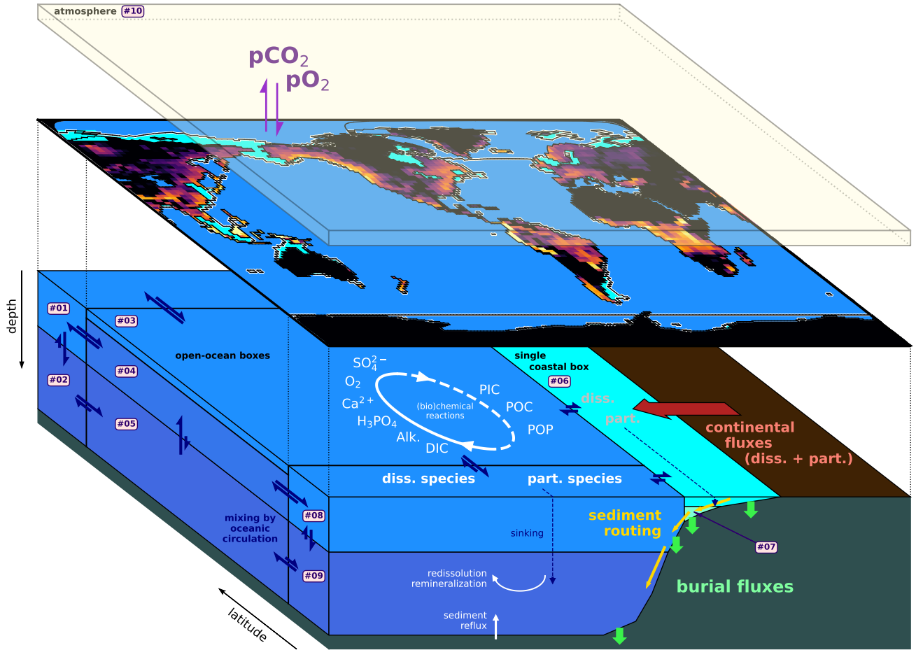
Figure 1. Schematics of GEOCLIM default 10 boxes configuration (9 oceanic + 1 atmospheric), with the number of each box indicated. The continental discretization is showed by the map of silicate weathering field. The 10 main GEOCLIM geochemical species (excluding tracers and isotopes) are indicated, and their global cycles broadly represented.
