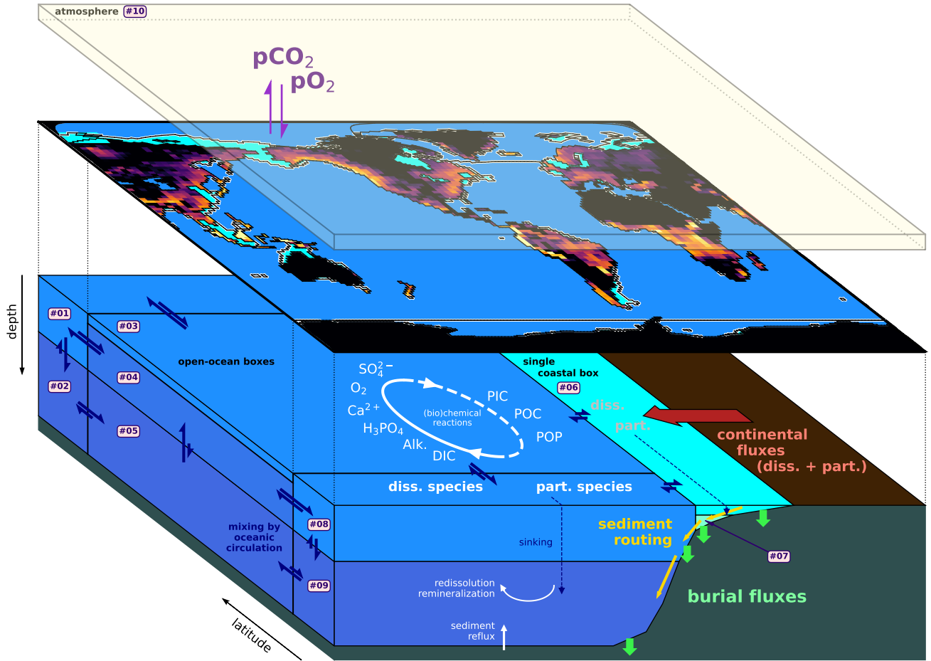
Figure 1. Schematics of GEOCLIM default 10 boxes configuration (9 oceanic + 1 atmospheric), with the number of each box indicated . The continental discretization is showed by the map of silicate weathering field. The 10 main GEOCLIM geochemical species (excluding tracers and isotopes) are indicated, and their global cycles broadly represented.
