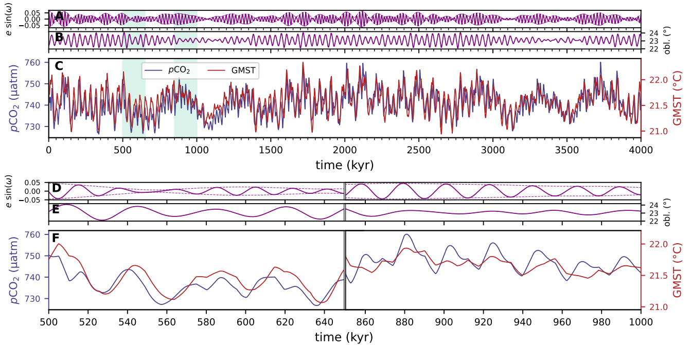
Figure 10. Time-series of orbital parameters (panels A, B, D and E), atmospheric p\text{CO}_2 and Global Mean Surface Temperature (panels C and F). First 4 Myrs of the 10 Myrs long GEOCLIM simulation with Laskar 95–85 Ma orbital solution, configuration o28'-APx0.25 (see Table 6), and \text{CO}_2 degassing set to 5 \text{ Tmol yr}^{-1} . Panels D-E-F show a zoom of the two time ranges indicated by the green shading on panels A-B-C, emphasizing the signal from obliquity (left block) and from precession (right block).
