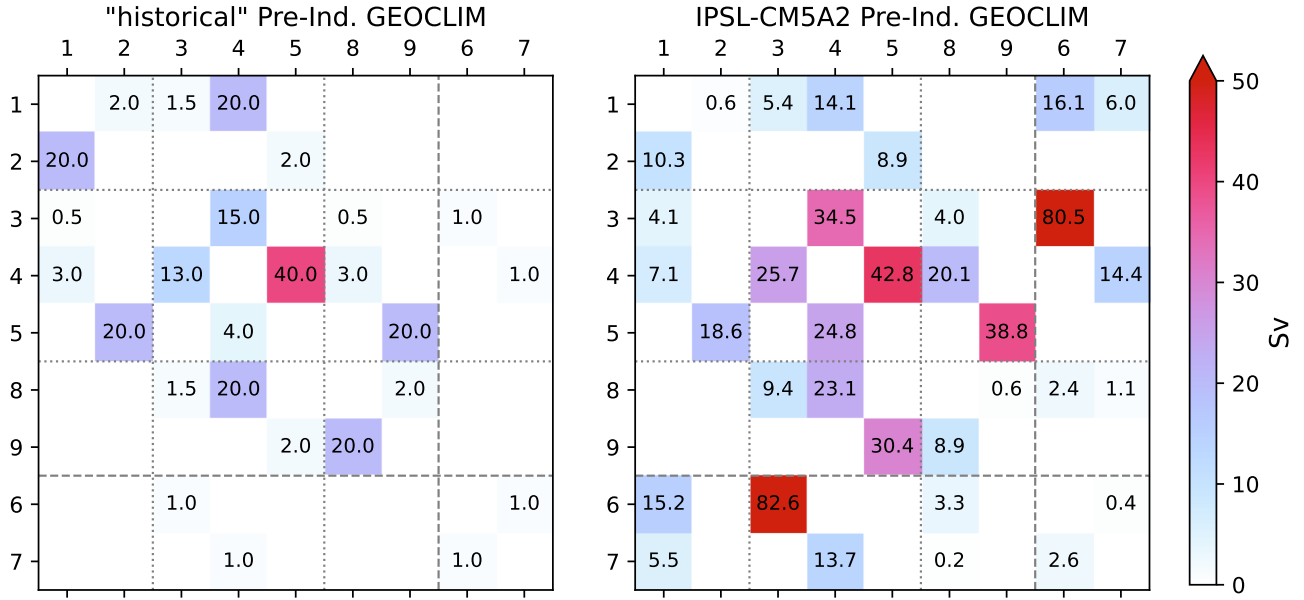
Figure C1. Flux matrices \mathbf{W} representing oceanic circulation between GEOCLIM boxes in pre-industrial default 9-boxes GEOCLIM configuration. Fluxes are oriented from column i to line j . The numbering of boxes is the default GEOCLIM one (#1–2: N hemisphere high-latitude (surface and deep), #3–4–5: mid-latitude (surface, intermediate and deep), #6–7: coastal oceans (surface and deep), #8–9: S hemisphere high-latitude). However, the positions of the box pairs (6,7) and (8,9) have been swapped on the figure, to better illustrate the distinction between “open-ocean” and “coastal” boxes.
