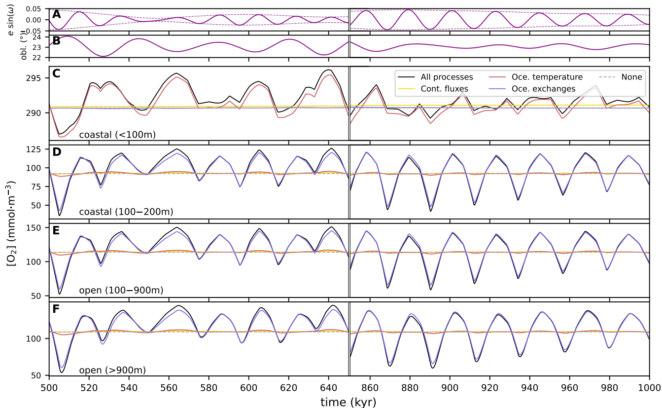
Figure 12. Orbital parameters and oxygen concentration (C–F) in Arctic basin. Transient GEOCLIM simulation with configuration o28’-APx0.25. The same two time ranges than as in Fig. 11 are shown. (A): Eccentricity (thin dashed line) and eccentricity times sine of precession angle (solid line); (B): Obliquity; (C)–(F): O_2 concentration in (C): Coastal surface box, (D): Coastal deep box, (E): Open-ocean intermediate box (F): Open-ocean deep box. Individual processes (i.e., continental fluxes, oceanic temperature and oceanic circulation) are switched on and off. “All processes” means that all processes are “active”. In the other cases, only the mentioned process is active, the other are kept constant at their initial values. “None” means that all the processes are kept constant.
