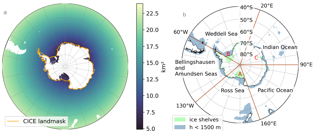
Figure 1. (a) Horizontal resolution of the domain in \text{km}^2 (from 40^\circ \text{S} ). The white area shows the ROMS land mask, and the orange line shows the edge of the CICE land mask around Antarctica. The area between these land masks contains the ice shelves that are included in ROMS, but not in CICE. (b) Map of the five Antarctic sectors used in the analysis. The light green shading shows the ice shelf cavities and the blue indicates areas with depths up to 1500 m, marking the continental shelves. The legends A, B and C in red indicate the three largest ice shelves: the Ross, Filchner-Ronne and Amery Ice Shelves, respectively.
