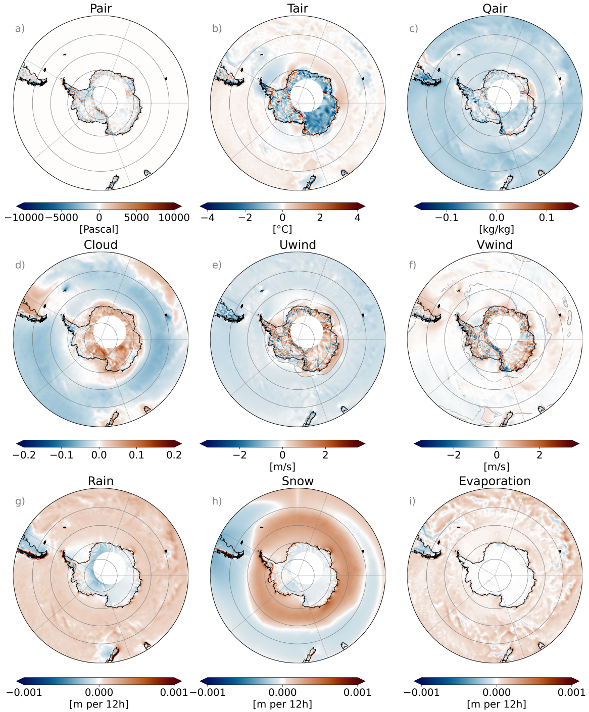
Figure B1. Differences between ERA5 and ERAI forcing fields calculated from 1992-2018 average. For Uwind and Vwind the plots (e,f) shows the change of the strength of the wind component in it's-its direction calculated as wind\_diff = (wind\_era5 / abs(wind\_era5)) * (wind\_era5 - wind\_eraI) , and the gray lines indicates the areas where the direction of the wind vector flips into the opposite direction.
