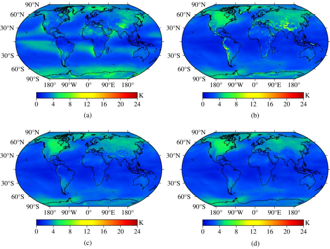
355 Figure 7 The RMSE distributions of the four models tested using global surface gridded T_m data from the ERA5 reanalysis product in 2017. (a) Bevis model. (b) GPT3-5 model. (c) GPT3-1 model. (d) NGGTm model.
