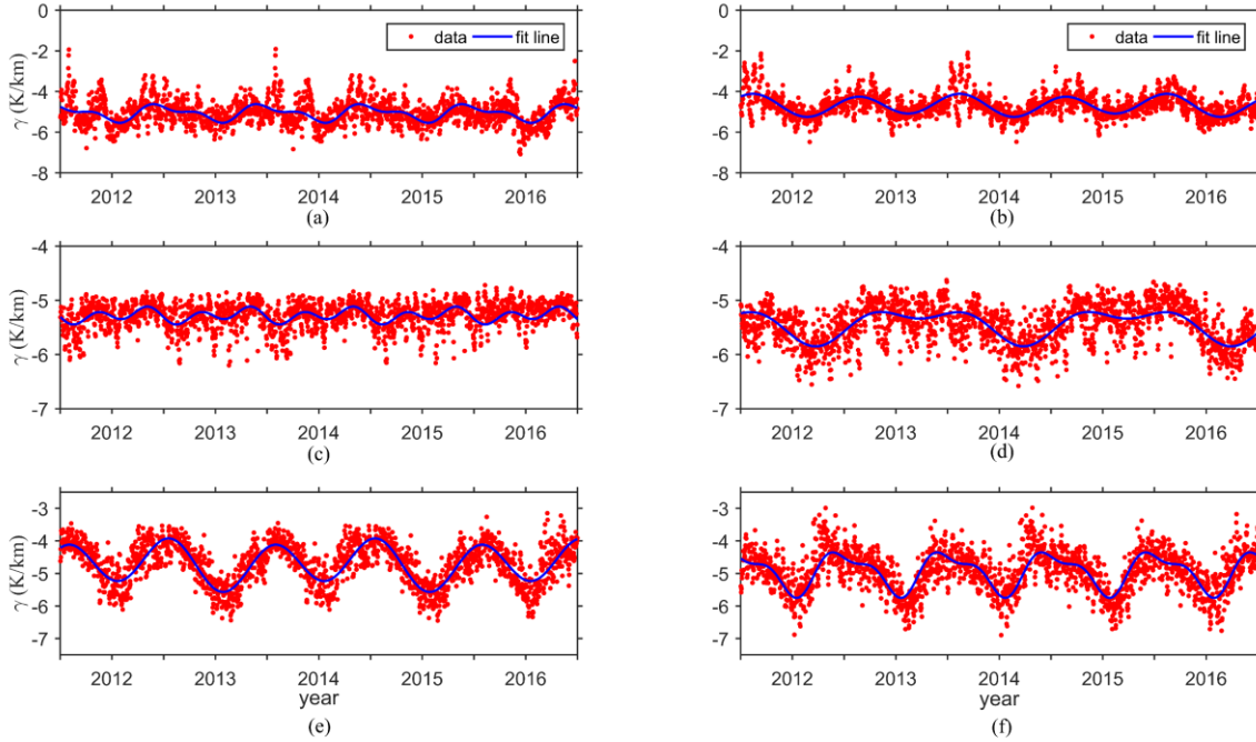
180 Figure 2 The time-series variations in the T_m lapse rate from the ERA5 reanalysis data at six representative grid points. (a) (60° N, 90° W). (b) (60° N, 90° E). (c) (0°, 90° W). (d) (0°, 90° E). (e) (60° S, 90° W). (f) (60° S, 90° E).
