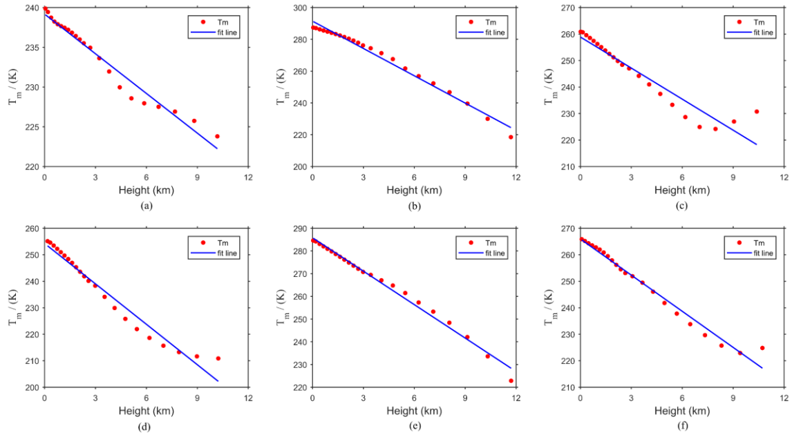
Figure 1 T_m changes with elevation at six representative ERA5 reanalysis data gridded points on January 1st, 2017. (a) (60° N, 90° W). (b) (0°, 90° W). (c) (60° S, 90° E). (d) (60° N, 90° E). (e) (0°, 90° E). (f) (60° S, 90° W).
