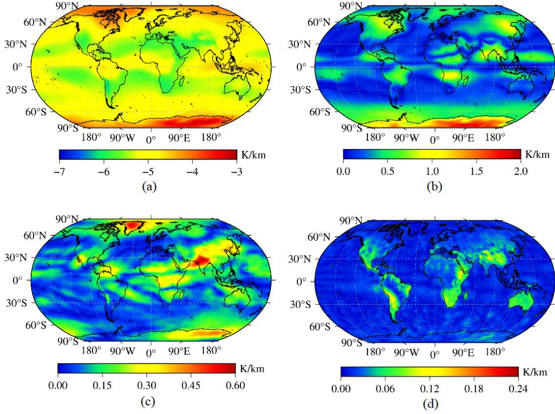
190 Figure 3 The distributions of the annual mean value and amplitudes of the T_m lapse rate calculated using global ERA5 reanalysis data. (a) annual average value. (b) annual cycle amplitude. (c) semiannual cycle amplitude. (d) daily cycle amplitude.
