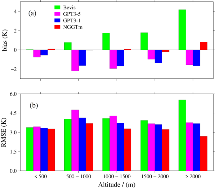
400 Figure 10 The bias and RMSE distributions within different elevation intervals for the four models tested using global T_m data from 378 radiosonde stations in 2017. (a) bias. (b) RMSE.
