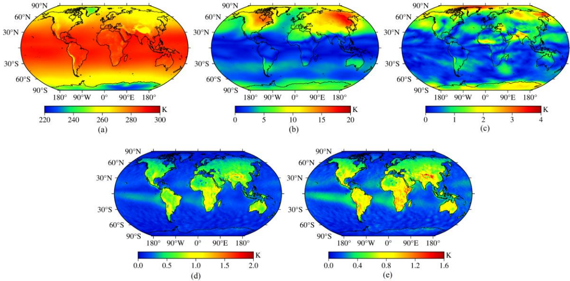
280 Figure 5 The distributions of the annual mean value and amplitudes of T_m calculated using global ERA5 reanalysis data. (a) annual mean value. (b) annual cycle amplitude. (c) semiannual cycle amplitude. (d) daily cycle amplitude. (e) half-day cycle amplitude.
