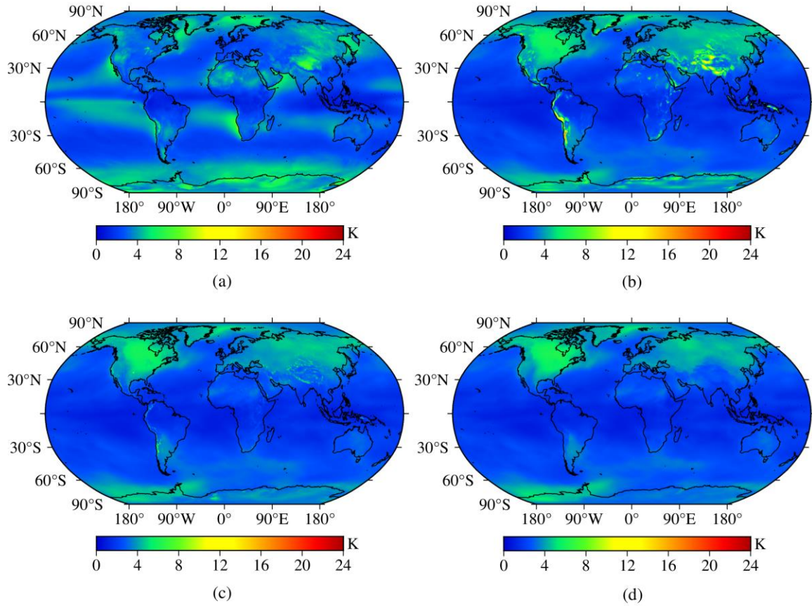
355 Figure 7 The RMSE distributions of the four models tested using global surface-level gridded T_m data from the ERA5 reanalysis product in 2017. (a) Bevis model. (b) GPT3-5 model. (c) GPT3-1 model. (d) NGGTm model.
