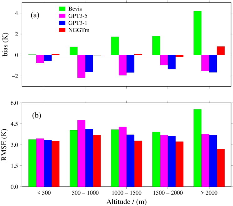
405 Figure 10 The bias and RMSE distributions within different elevation intervals for the four models tested using global T_m data from 378 radiosonde stations in 2017. (a) bias. (b) RMSE.
