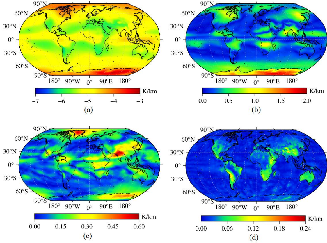
195 Figure 3 The distributions of the annual mean value and amplitudes of the T_m lapse rate calculated using global ERA5 reanalysis data. (a) annual average value. (b) annual cycle amplitude. (c) semiannual cycle amplitude. (d) daily cycle amplitude.
