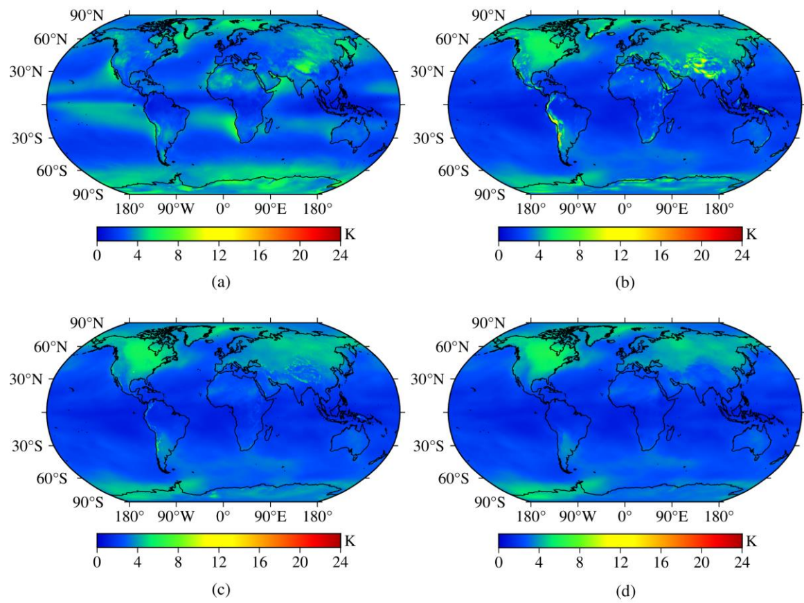
Figure 7 The RMSE distributions of the four models tested using global surface-level gridded T_m data from the 360 ERA5 reanalysis product in 2017. (a) Bevis model. (b) GPT3-5 model. (c) GPT3-1 model. (d) NGGTm model.
