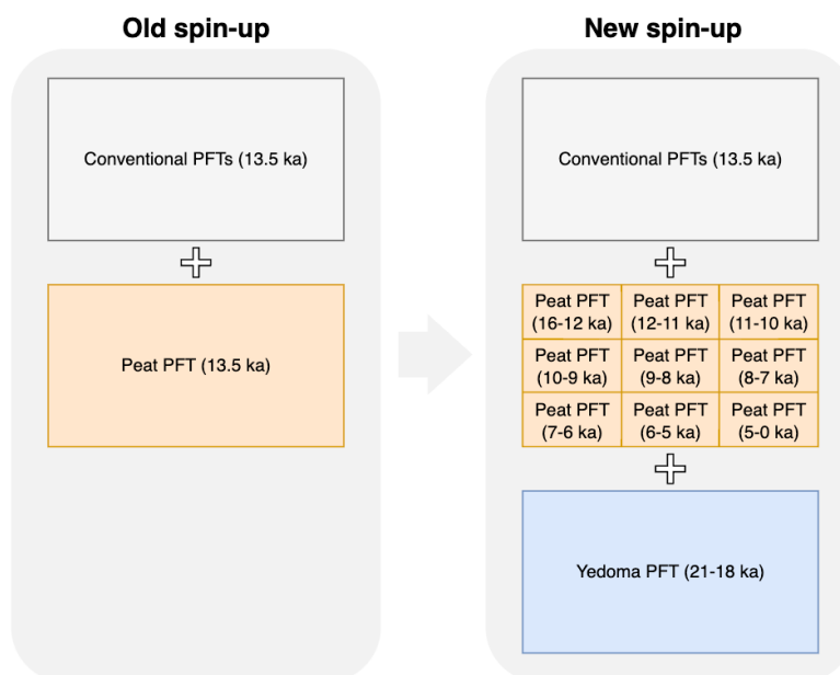
Figure 1: Schematic representation of carbon types simulated by the old and new spin-up simulations. The numbers in brackets show the inception time of each plant function type (PFT). Compared to the old spin-up, a new PFT, Yedoma, and nine age cohorts for peat PFT were considered in the new spin-up.
