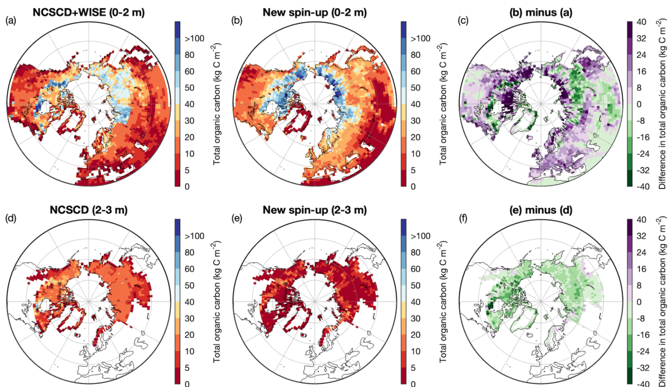
Figure 9: Comparison of spatial distributions of total organic carbon for 0-2 m and 2-3 m soil layers over the Northern Hemisphere (> 30°N) between two observation-based soil datasets (NCSCD for 0-3 m soil layers in permafrost regions, and WISE for 0-2 m soil layers in non-permafrost regions) and the new spin-up simulation. The first two columns show total organic carbon from the two observation-based soil datasets ((a) and (d)) and new spin-up simulations ((b) and (e)), and the third column for the difference between simulations and observations. 435
