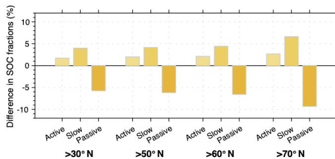
460 Figure 10: Difference in SOC fractions between the new and old spin-up simulations for areas > 30°N, > 50°N, > 60°N, and > 70°N. The four areas include 100%, 79%, 55%, and 11% of total SOC of the study area, respectively in the new spin-up simulation.
