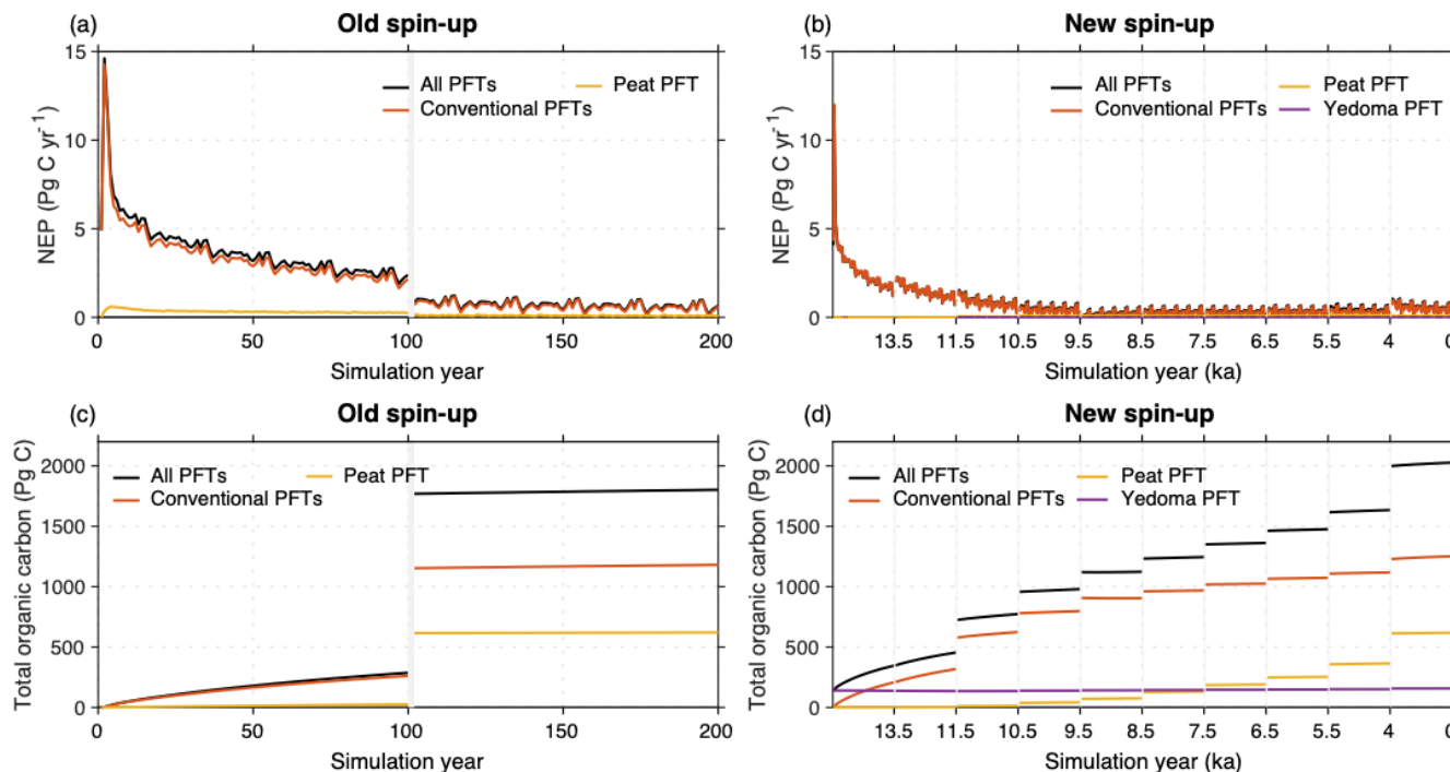
300 Figure 5: Time series of net ecosystem productivity (NEP) and total organic carbon over the Northern Hemisphere ( > 30^{\circ}\text{N} ) from the old ((a) and (c)) and the new ((b) and (d)) spin-up simulations. Conventional PFTs indicate the 15 non-yedoma and non-peat PFTs including bare soil, 8 tree PFTs, 4 grass PFTs, and 2 crop PFTs. The simulation periods using the stand-alone soil carbon module (SubC) are not plotted in all figures as the model only outputs the simulation results of the last year of each period to save storage space.
