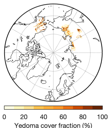
220 Figure 2: Spatial distribution of present-day Yedoma region from Strauss et al. (2021), shown at the initial spatial resolution of 0.05^\circ \times 0.05^\circ .
