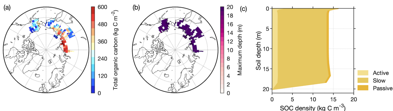
285 Figure 4: Yedoma carbon accumulation from the new spin-up simulation. Spatial distribution of simulated (a) total organic carbon (per \text{m}^2 Yedoma deposits) and (b) the maximum depth of total organic carbon, and (c) the simulated mean vertical distribution of carbon density of three soil carbon pools (active, slow and passive) over present-day Yedoma region by the end of the LGM.
