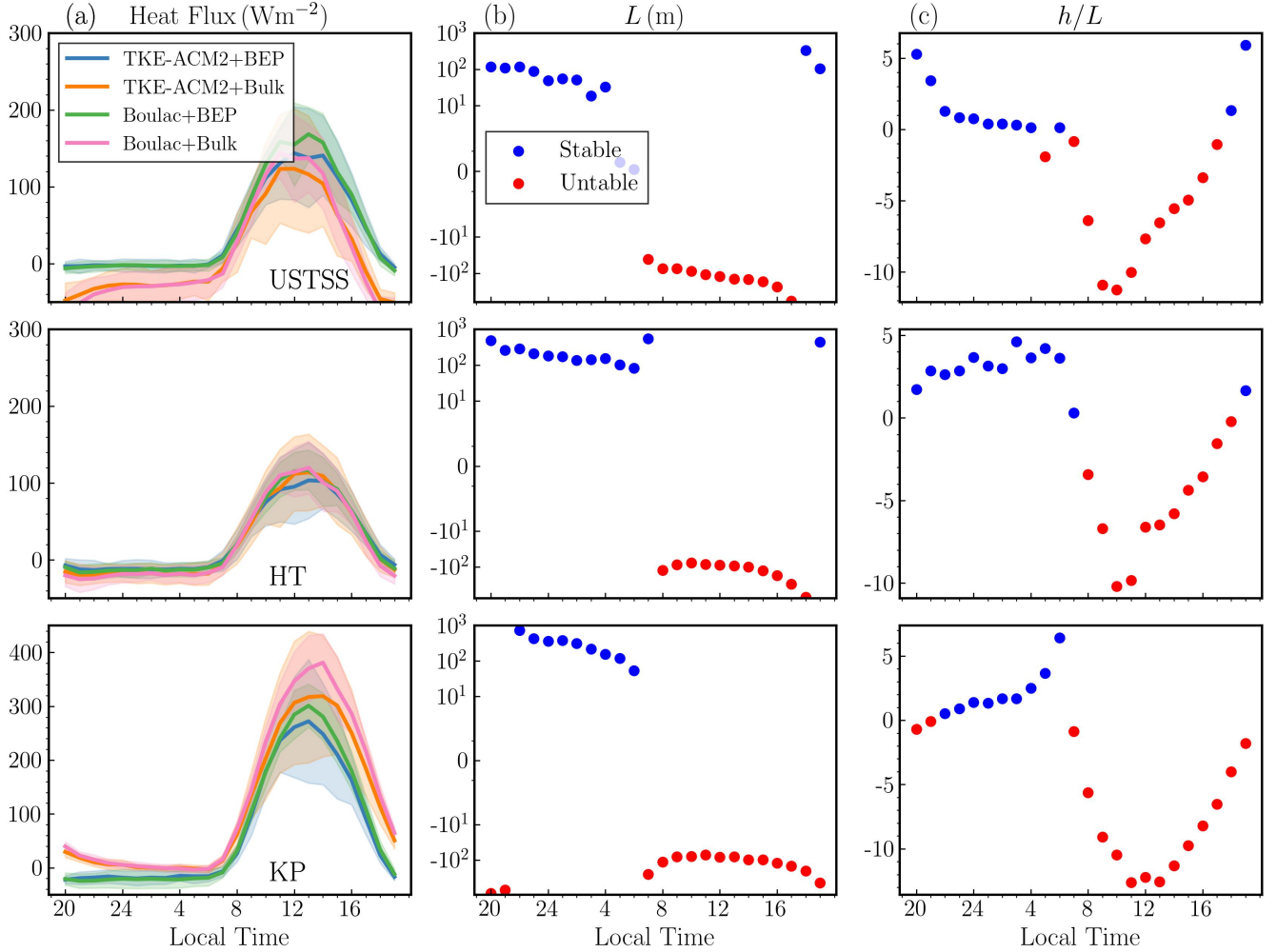
Figure 9. Column a) monthly mean diurnal patterns of the surface heat flux for USTSS_LCZ5, HT_rural, and KP_LCZ1 from top to bottom; Column b) Monin-Obukhov length ( L ) with a semi-log y -axis; Column c) stability parameter ( h/L ). The integration is from 2000 UTC+8 on 18 th July in 2022 to 2000 UTC+8 on 18 th August in 2022.
