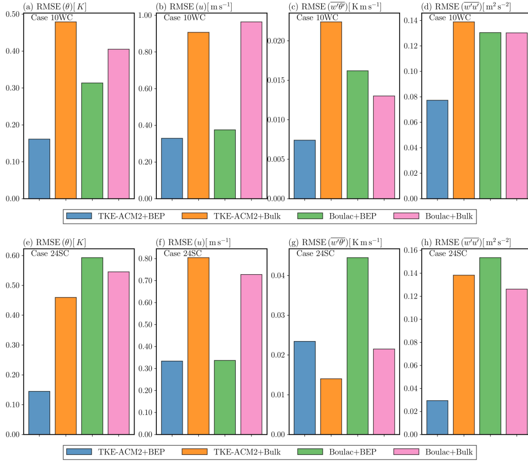
Figure 6. a-d): RMSEs for \theta , u , \overline{w'\theta'} , and \overline{w'u'} , calculated below the PBL height for Case 10WC by taking the LES results as the ground truth, respectively; e-h): same as a-d) but for Case 24SC.
