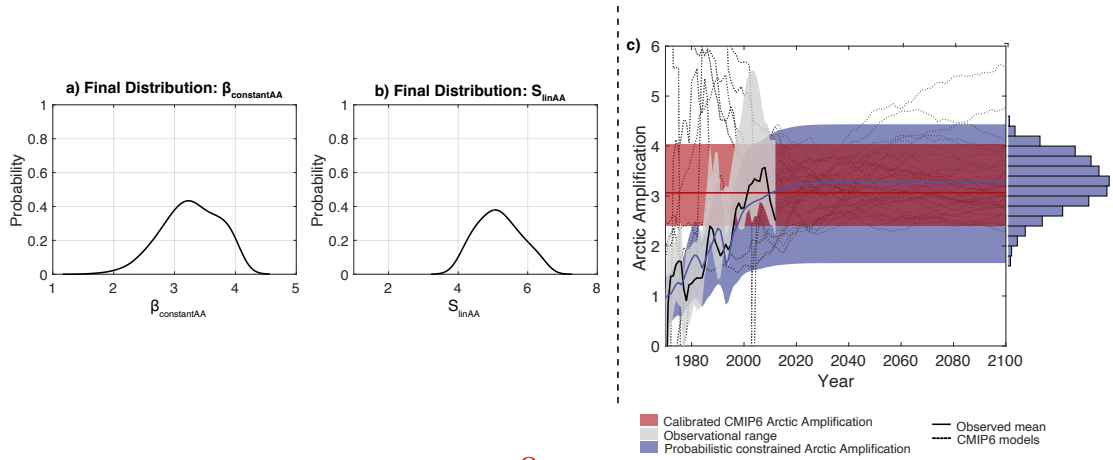
Figure 3. Constrained Arctic amplifications Amplification from our parameterisation framework, as presented in Eq. 2. a and b) represent the probability distributions of \beta_{\text{constantAA}} and S_{\text{linAA}} respectively, the driving parameters in our constrained Arctic Amplification equation (Eq. 2). c) shows the final constrained Arctic Amplification. Light grey shading represents the ‘very likely’ (5th-95th percentile) observational observed Arctic Amplification range, where whereas the black solid line is the observational mean. Red shading represents the ‘very likely’ CMIP6 calibrated Arctic Amplification range (Eq. 1), where whereas the red solid line is the CMIP6 calibrated multi-model mean. Blue shading represents the final constrained uncertainty range, while the blue histogram represents the frequency of each Arctic Amplification uncertainty value in the range. We take 2012 as the final year of observations, as it is the last year a central point can be taken with 10 years either side to calculate the 21-year trend without reducing the number of years in the trend, which could bias the trend of the final years.
