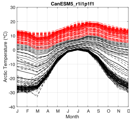
Figure A5. Comparison of our emulated seasonal Arctic temperature evolution with its CMIP6 counterpart to 2300. Black lines represent the 1850-2100 temperature cycle, while red lines represent the 2100-2300 seasonal cycle temperature evolution. Solid lines represent our emulation of the CMIP6 trend, while dashed lines represent CMIP6 data for the first ensemble member of model CanESM5.
