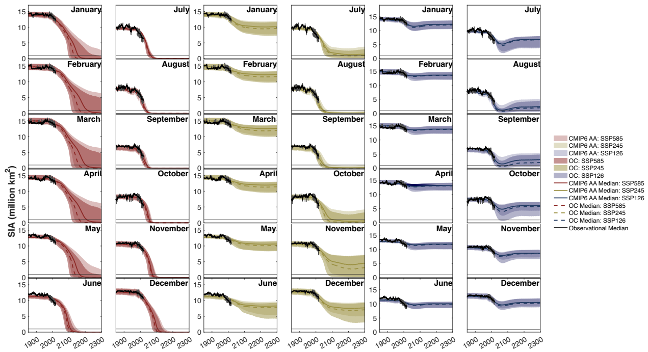
Figure B2. Emulated likely range of the monthly Arctic SIA over the time period 1850-2300 when our emulator is forced with the MAGICC 600-member ensemble global mean temperature anomaly. Red, yellow and blue shading represents SSP5-8.5, SSP2-4.5 and SSP1-2.6 respectively. Darker shading represents the projections from our observationally constrained emulator, and lighter shading represents the projections when forcing our emulator with the CMIP6 calibrated (linear) Arctic Amplification. The dashed and solid lines represent the mean SIA from each set of projections respectively. The black line spanning 1850-2020 represents observational data.
