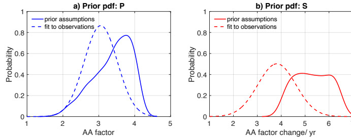
Figure A1. Contribution of each parameter to the observationally constrained Arctic Amplification between 1970 and 2100. a and b) show the two initial distributions for parameters \sigma_{\text{linAA}} and p_{\text{constantAA}} before they are averaged and normalised. The solid line reflects our assumptions of current and future Arctic Amplification, while the dashed line reflects actual trends from both observations and CMIP6 models.
