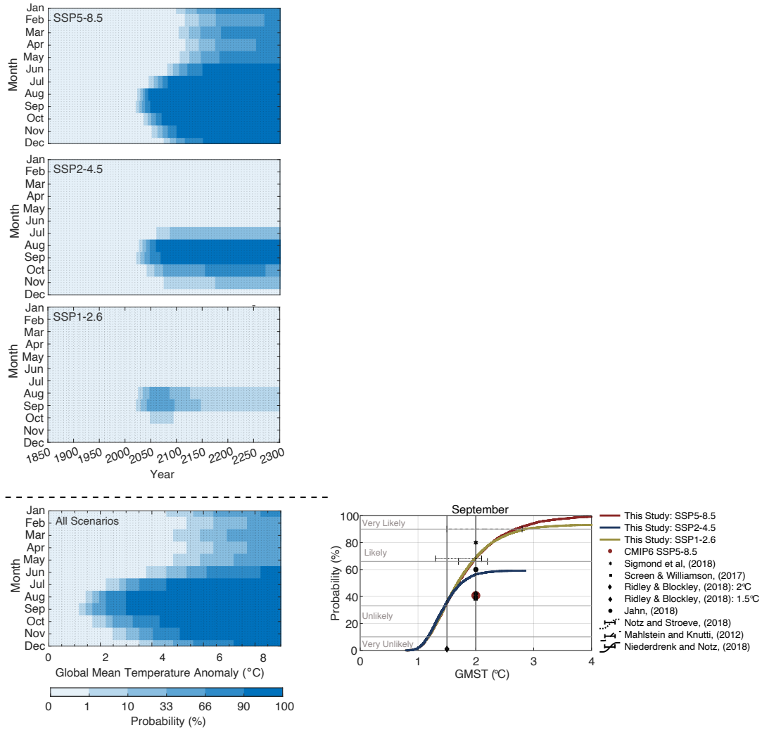
Figure 9. The probability of ice-free conditions in each month, year and global mean temperature by 2300 generated from our observationally constrained emulator parameterisations . The probability in each year under SSP5-8.5, SSP2-4.5 and SSP1-2.6 are given in the upper three panels. The probability as a function of global temperature is shown in the bottom panel, and is calculated from the likelihood of ice-free conditions at each global temperature under all three scenarios combined. Darker blue patches represent increasingly ice-free conditions, while whiter patches indicate years and temperatures where a high percentage of emulator ensemble members project high ice cover above 1 million square kilometers. The right panel represents the cumulative probability of the global mean temperature at which the SIA falls below 1 million km 2 for the first time in our observationally constrained emulator parameterisations . Red, yellow and blue represent SSP5-8.5, SSP2-4.5 and SSP1-2.6 respectively. Errorbars and scattered shapes represent probability ranges from other studies.
