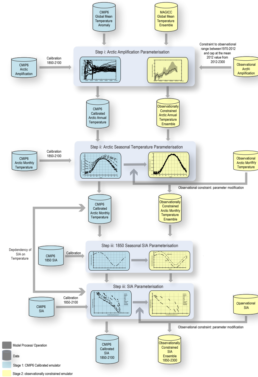
Figure 1. A work-flow of emulator development the parameterisation framework. Blue cylinders and boxes represent the calibration to CMIP6 models in Stage 1. Yellow cylinders and boxes represent the constraint to observational data in Stage 2. Cylinders represent the data that is used in each parameterisation step, while boxes represent the output from each parameterisation step. Refer to Sections 4.2.1 and 4.2.1 for more information on Step i. Refer to Section 4.3 for more information on Step ii. While section 4.4 provides more information on Step iii.
