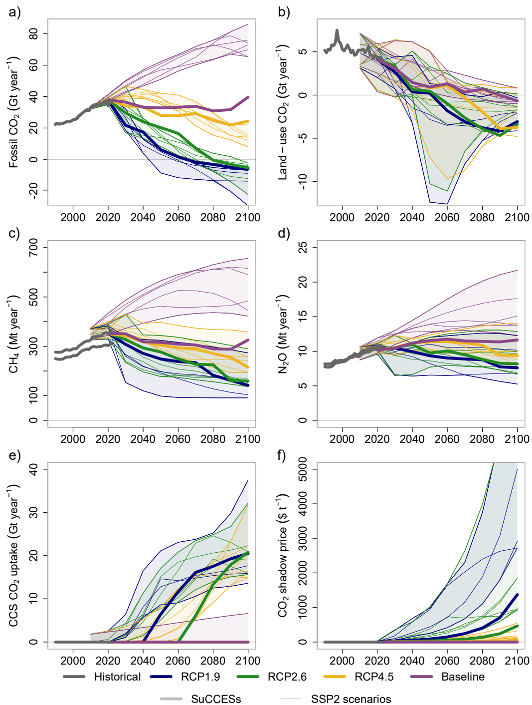
Figure 5: Comparison of a) fossil and industry \text{CO}_2 , b) land-use \text{CO}_2 , c) \text{CH}_4 , and d) \text{N}_2\text{O} emissions, and e) \text{CO}_2 uptake by CCS and f) carbon prices between historical estimates (grey), and baseline, RCP4.5, RCP2.6 and RCP1.9 scenarios (indicated by colour) from SuCCESs (thick lines) and other IAMs from the SSP database (thin lines, with shaded areas indicating the range).
