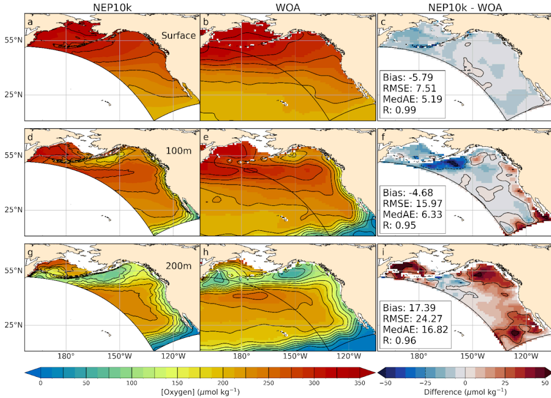
Figure 12: Dissolved oxygen comparisons. Annual mean surface and subsurface (100m, 200m) dissolved oxygen compared against WOA23. Comparison time frames cover 1993-2019. Reference contours are depicted in black at 25 \mu\text{mol oxygen kg}^{-1} sea water in the mean state (left and center columns) and difference (right column) plots; contours representing negative values in the difference plot are drawn as dashed lines. Bias, Root Mean Squared Error (RMSE), Median Absolute Error (MedAE) and Pearson Correlation Coefficient (R) are reported in the right column of figures depicting the difference between NEP10k and WOA23. The extent of the NEP10k domain is outlined in black in all figures.
