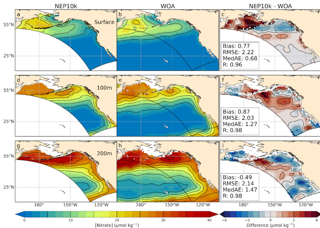
Figure 7: Nitrate comparisons. Annual mean surface and subsurface (100m, 200m) nitrate compared against WOA23. Comparison time frames cover 1993-2019. Reference contours are depicted in black at 5 and 1.5 \mu\text{mol nitrate kg}^{-1} sea water in the mean state (left and center columns) and difference (right column) plots, respectively; contours representing negative values in the difference plot are drawn as dashed lines. Bias, Root Mean Squared Error (RMSE), Median Absolute Error (MedAE) and Pearson Correlation Coefficient (R) are reported in the right column of figures depicting the difference between NEP10k and WOA23. The extent of the NEP10k domain is outlined in black in all figures.
