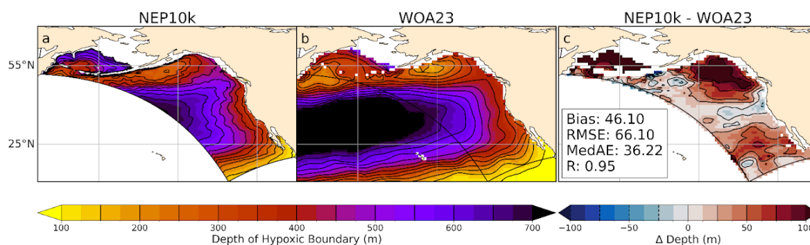
Figure 13: Hypoxic Boundary Layer Depth. Annual mean hypoxic boundary layer depth (i.e., depth at which dissolved oxygen concentration drops below 61.7 \mu\text{mol oxygen kg}^{-1} sea water) compared against WOA23. Black reference contours indicate 150 meter and 25 meter intervals in the mean state (a, b) and difference (c) plots, respectively; contours representing negative values in c are drawn as dashed lines. Area-weighted mean bias (Bias) and root mean squared error (RMSE), and the median absolute error (MedAE) and Pearson correlation coefficient (R) are reported in panel c. The extent of the NEP10k domain is outlined in black in all figures.
