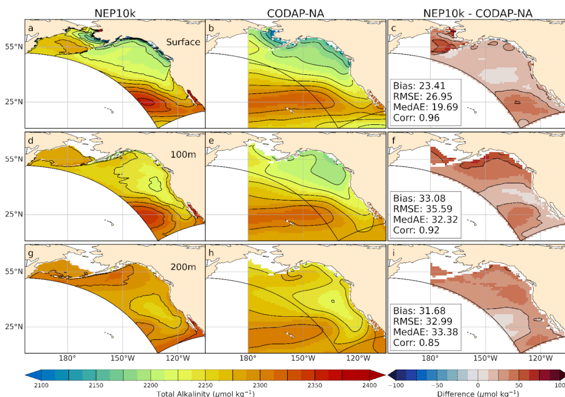
Figure 14: Total Alkalinity Comparisons. Annual mean surface and subsurface (100m, 200m) total alkalinity compared against CODAP-NA. Comparison time frames cover 2004-2018. Reference contours are depicted in black at 25 \mu\text{mol alkalinity kg}^{-1} sea water in the mean state (left and center columns) and difference (right column) plots. Area-weighted mean bias (Bias) and root mean squared error (RMSE), and the median absolute error (MedAE) and Pearson Correlation coefficient (R) are reported in the right column of the difference plots. All correlation values are significant at p < 0.001 . The extent of the NEP10k domain is outlined in black in all figures.
