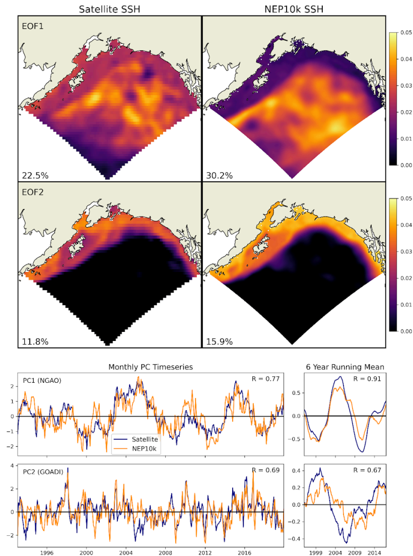
Figure 22: GOA SSH EOFs and principal component timeseries. Spatial maps of the first (top row) and second (middle row) EOFs for satellite (left) and NEP10k (right) SSH variability. These are complemented with timeseries comparisons (monthly, left; 6 year running mean, right) for the first two principal components (NGAO, top row; GOADI, bottom row) from the empirical orthogonal function analyses of Gulf of Alaska sea surface height for NEP10k (orange) and the CMEMS satellite product (navy). R values indicate the Pearson Correlation coefficient calculated between NEP10k and the Satellite product, all of which are significant at p < 0.001 . X-axis labels indicate January 1st of the specified year.
