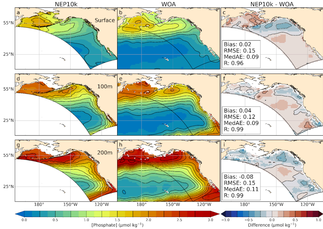
Figure 8: Phosphate comparisons. Annual mean surface and subsurface (100m, 200m) phosphate compared against WOA23. Comparison time frames cover 1993-2019. Reference contours are depicted in black at 0.25 \mu\text{mol phosphate kg}^{-1} sea water in the mean state (left and center columns) and difference (right column) plots; contours representing negative values in the difference plot are drawn as dashed lines. Bias, Root Mean Squared Error (RMSE), Median Absolute Error (MedAE) and Pearson Correlation Coefficient (R) are reported in the right column of figures depicting the difference between NEP10k and WOA23. The extent of the NEP10k domain is outlined in black in all figures.
