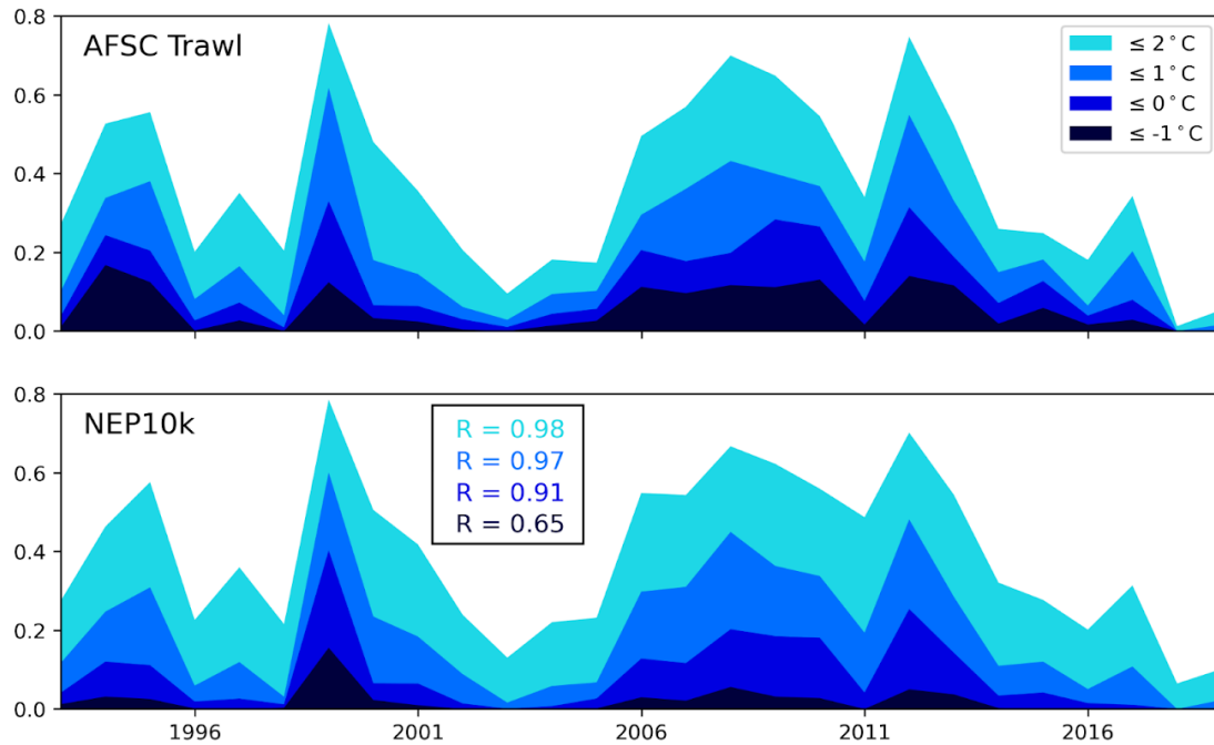
Figure 20: Southeastern Bering Sea cold pool area index. Comparison of the cold pool index timeseries derived from the AFSC bottom trawl survey data (top) and the spatially and temporally consistent NEP10k bottom temperature output (bottom) following the methods described in Rohan et al. (2022) and AFSC coldpool software repository. The plots report the fraction of the total survey south eastern Bering Sea trawl area (outlined in the figure above) that exhibits bottom temperatures under the specified thermal thresholds. We report Spearman correlation values between NEP10k and trawl indices in the bottom panel.
