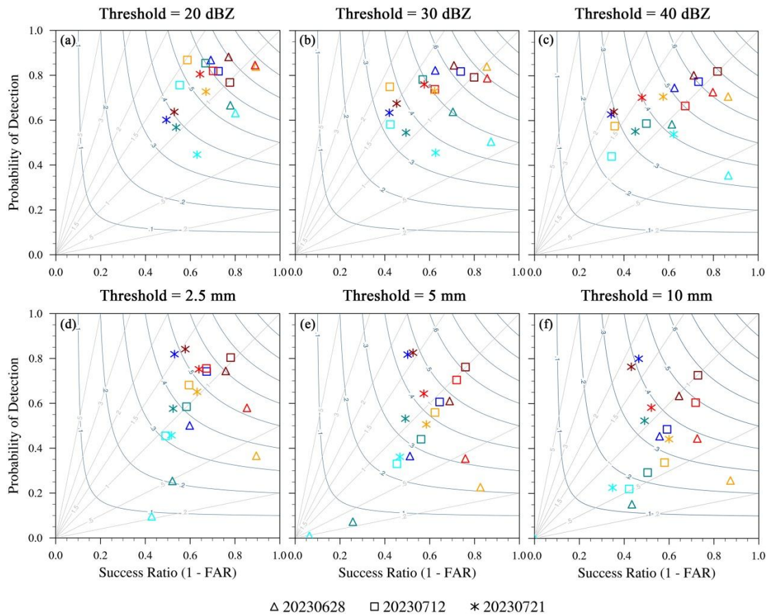
Figure 15. Performance diagram for 0-6 h CREF forecasts from the NoDA (cyan, dark cyan, and blue) and FH_RD (orange, red, and brown) experiments in each case at thresholds of (a) 20, (b) 30, and (c) 40 dBZ, respectively. (d–f) Same as in (a–c), but for 1-6 h HPRCP forecasts from each case at thresholds of (d) 2.5, (e) 5, and (f) 10 mm, respectively. Cyan and orange represent the analysis (1-h forecast for precipitation), dark cyan and red for 3-h forecasts, and blue and brown for 6-h forecasts. Results are shown for a neighborhood radius of 12-km.
