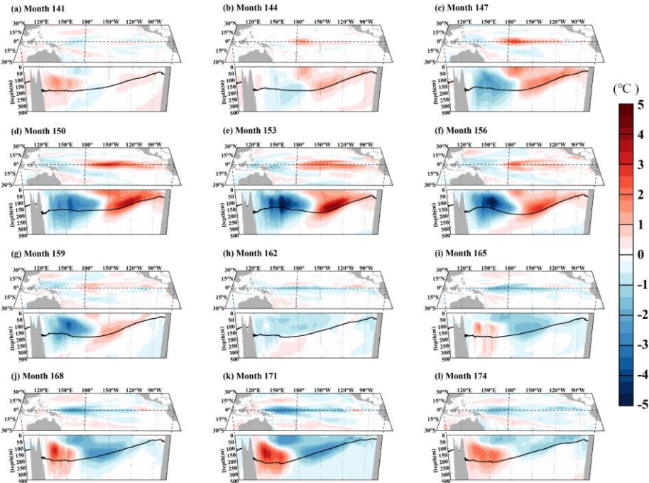
Figure 13: Three-dimensional temperature anomalies over the simulated ENSO cycle from month 141 to 174 in the sensitivity experiment with \alpha_r=1.5 .
