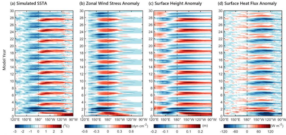
Figure 10: Hovmöller diagram of simulated (a) SSTA, (b) zonal wind stress anomaly, (c) surface height anomaly and (d) surface heat flux anomaly averaged over the tropical zone of 5 °S to 5 °N along the equator for the sensitivity experiment with \alpha_\tau=1.5 .
