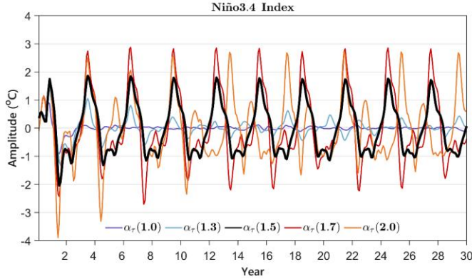
Figure 9: Simulated Niño 3.4 index in the sensitivity experiments with different interannual wind stress coupling coefficients. The purple line is for \alpha_\tau=1.0 , the blue line for \alpha_\tau=1.3 , the black line for \alpha_\tau=1.5 , the red line for \alpha_\tau=1.7 , and the orange line for \alpha_\tau=2.0 , respectively.
