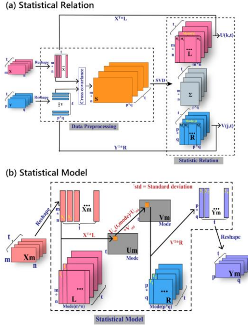
Figure 1: Flow chart of (a) SVD analysis and (b) SVD-based statistical model. \mathbf{X} and \mathbf{Y} in (a) are original interannual variation signals before SVD, \mathbf{S} is the covariance matrix between \mathbf{X} and \mathbf{Y} , \mathbf{L} is the left-singular vector and \mathbf{R} is the right-singular vector, \mathbf{U} and \mathbf{V} are, respectively, the time series of left-singular vector and right-singular vector, and \mathbf{\Sigma} is the singular value matrix. \mathbf{Xm} in (b) is the input left field to the statistical model, \mathbf{Ym} is the output right field, and \mathbf{Um} and \mathbf{Vm} are calculated time series of left field and right field in the statistical model, respectively.
