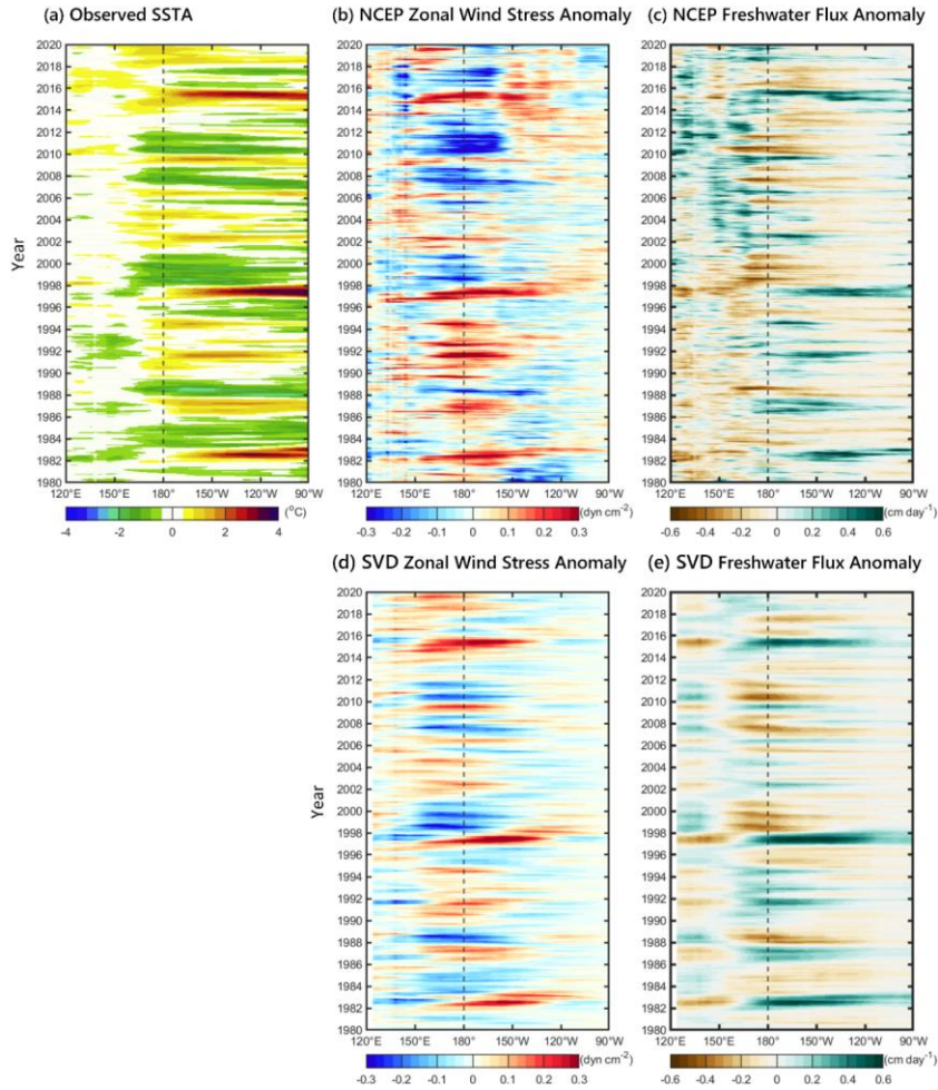
Figure 6: Hovmöller diagram of observed (a) SSTA, (b) zonal wind stress anomaly, and (c) FWF anomaly over the tropical zone of 5°S to 5°N from 1980 to 2020. (d) and (e) are respectively the retrieved zonal wind stress anomaly and FWF anomaly using the statistical atmospheric model forced by the observed SSTA. The vertical dashed line indicates the dateline.
