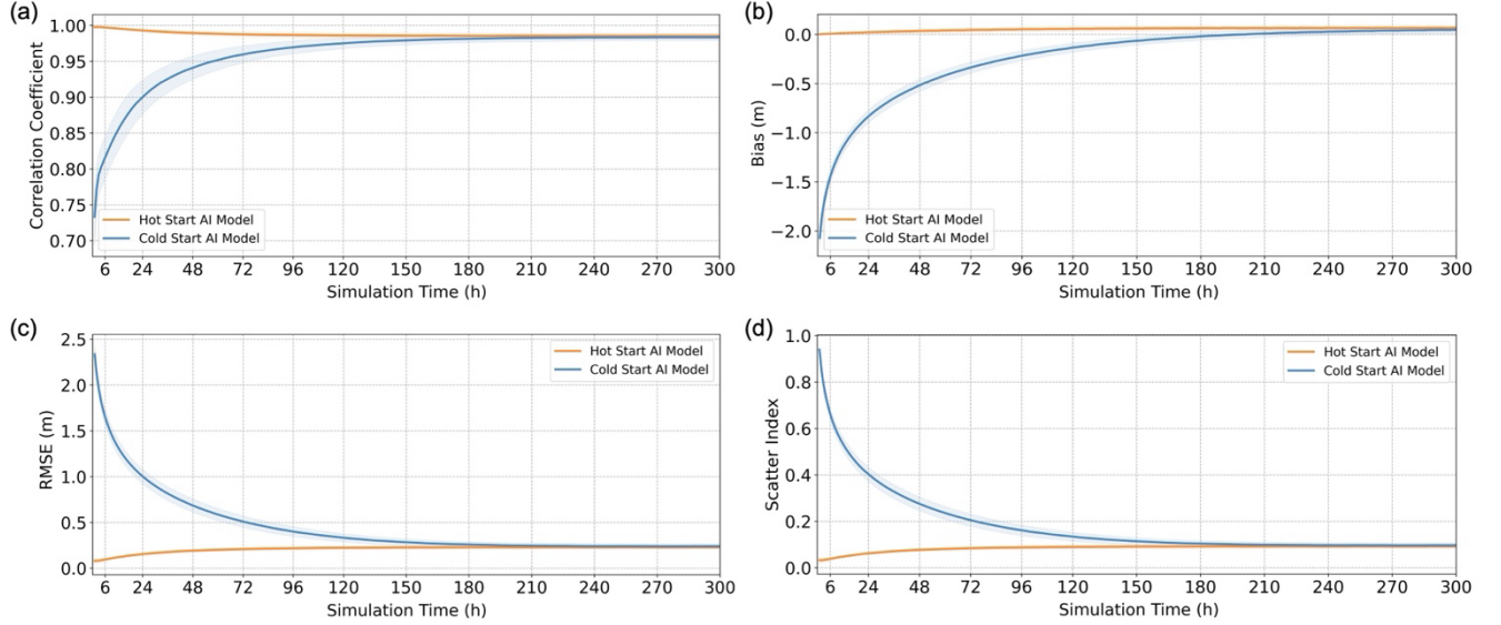
Figure 3: The variation of global overall error metrics between the AI SWH model outputs and ERA5 with simulation time: (a) CC, (b) bias, (c) RMSE, and (d) SI. The orange lines and shaded areas are the same as those in Fig. 2, but no epoch ensemble is used. The blue lines and shaded area are the corresponding results for the cold start with an initial field of zero SWH. These results do not use data assimilation.
