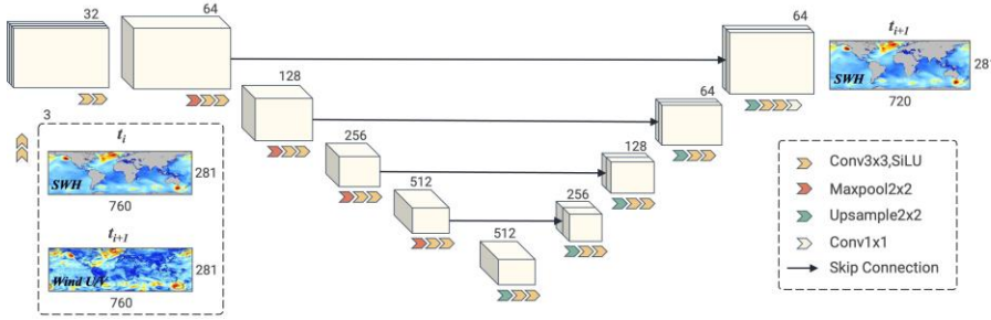
170 Figure 1: An illustration of the U-Net architecture used in this study. Each cube represents a feature map, with the numbers on the sides indicating the number of channels. The legend on the lower-right panel explains the meaning of the different arrows used in the schematic diagram.
