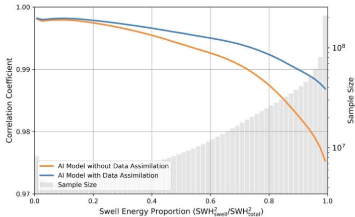
340 Figure 5: Correlation coefficient between AI model and ERA5 data as a function of swell energy proportion the global ocean in the year of 2020. The orange and blue lines represent the AI model before and after data assimilation, respectively, and the grey bars indicate the variation in sample size as a function of swell energy proportion.
