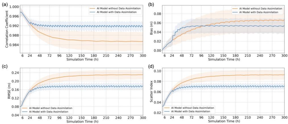
250 Figure 2: The variation of global overall error metrics between the AI SWH model outputs and ERA5 with simulation time: (a) CC, (b) bias, (c) RMSE, and (d) SI. The orange and blue lines represent the mean values of the error metrics for the 236 experiments starting from different initial SWH fields, before and after assimilation, respectively. The shaded areas around the lines indicate the range of error metrics across different experiments with varying initial SWH fields.
