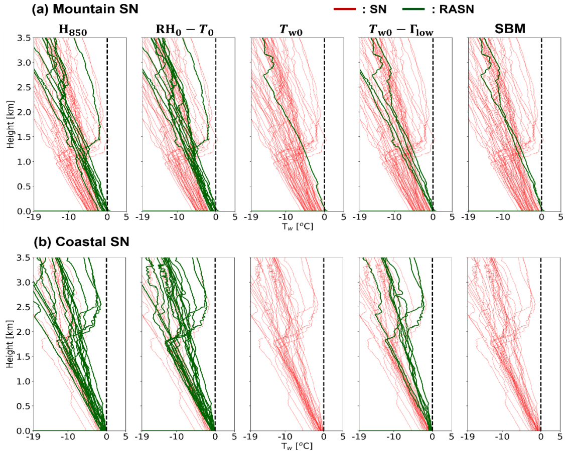
Figure 10. T_w profiles for observed SN cases occurring at (a) mountain sites and (b) coastal sites. The blue, red, and green lines indicate diagnosed RA, SN, and RASN cases, respectively, for the H_{850} thickness, shifted Matsuo scheme on RH_0 - T_0 method, wet-bulb temperature T_{w0} , T_{w0} - \Gamma_{low} method, and the current SBM methods. Bold lines indicate misdiagnosed cases.
