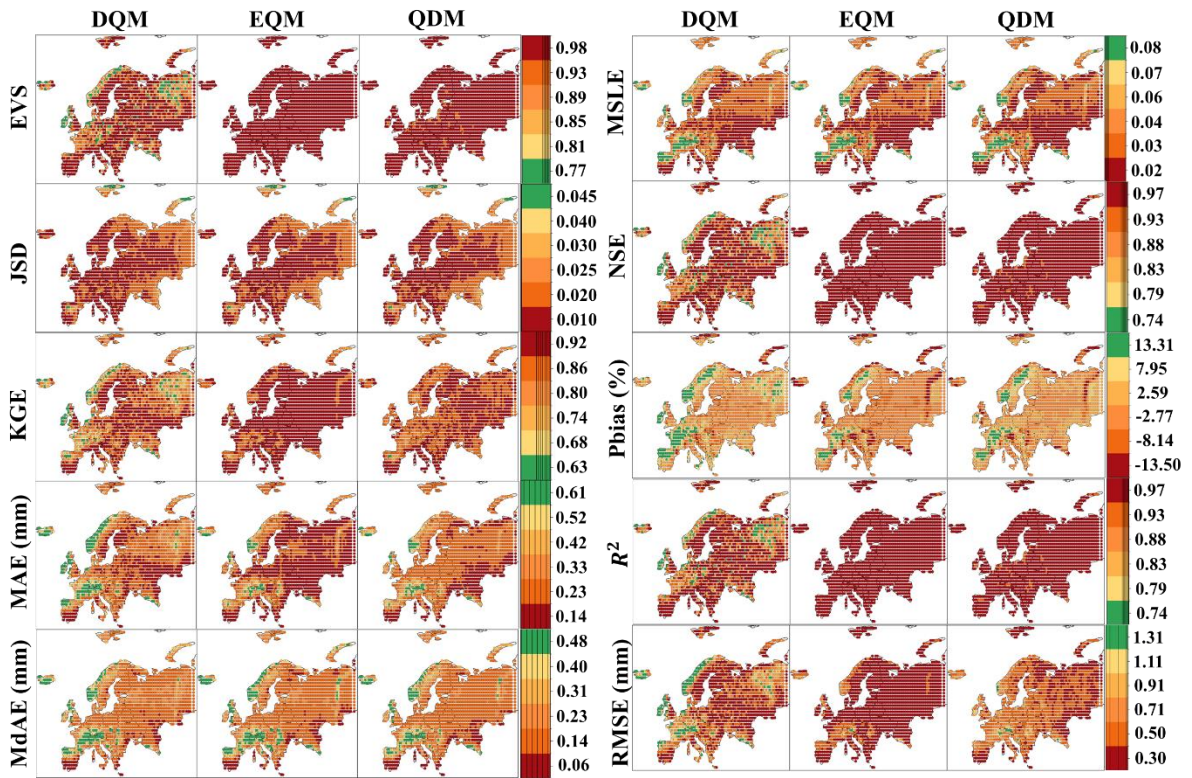
Figure 6. Performance comparison of DQM, EQM, and QDM for the validation period (1997-2014) using evaluation metrics for daily precipitation in Europe.
