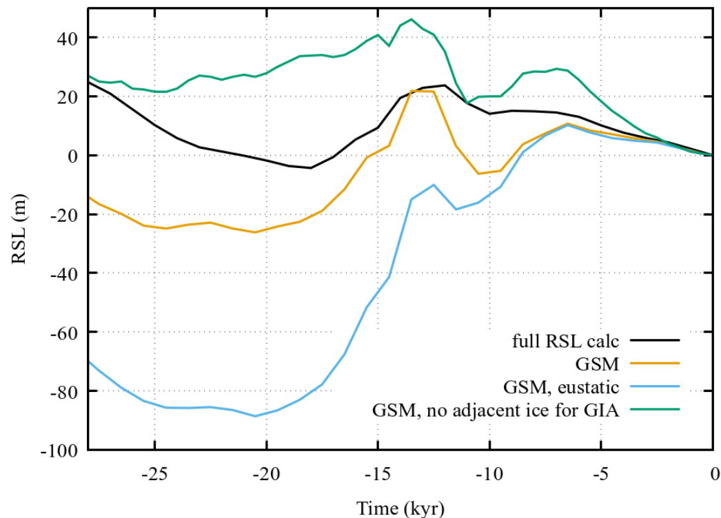
Figure 8. Comparison of computed relative sea level (RSL) for Franz Joseph Fjord Greenland ( 27.42^{\circ} west, 73.02^{\circ} N). Shown are: the gravitationally-self consistent solution from post-processing (“full RSL calc”), the GSM internal solution using linear geoidal deflection (“GSM”), the solution when geoidal deflection is typically neglected (“GSM, eustatic”), and the GSM solution when ice outside of the regional grid is not accounted for in the visco-elastic bedrock response calculation (“GSM, no adjacent ice for GIA”).
